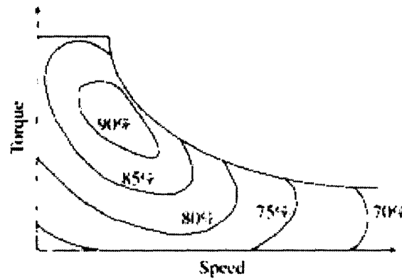
Figure 2.4: Efficiency at different torque-speed combinations for a one-gear electric motor. (Source: Chan, Chau, 2001)
