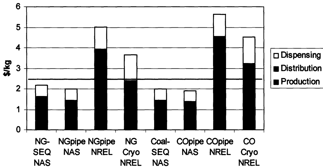
Figure 3.15: Cost estimates NREL, 2002 and NAS, 2004 by stage.
