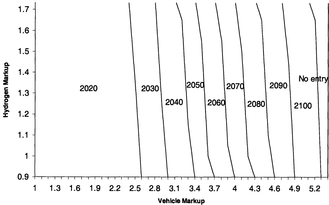
Figure 6.11: Entry decade in the Europe for scenario(vi)
