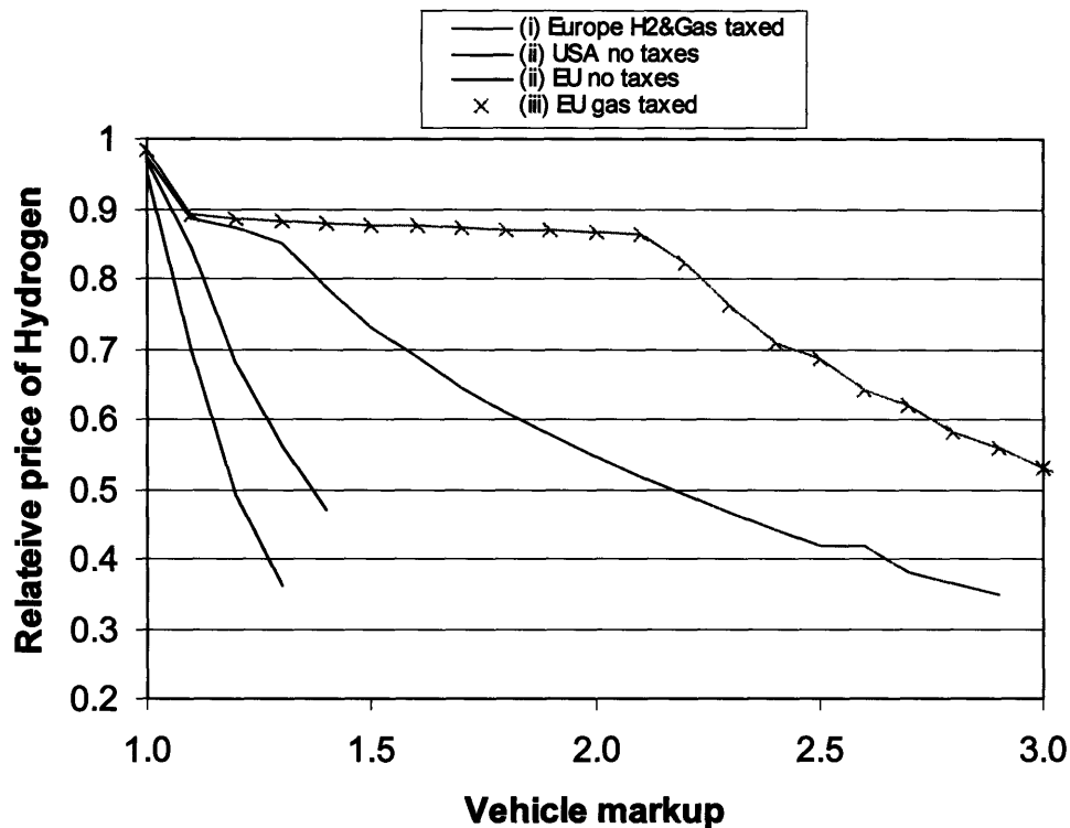
Figure 6.1: Relative hydrogen price at the moment of sector entry
