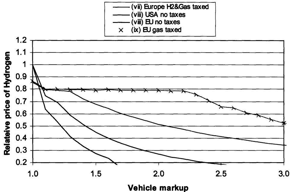
Figure 6.3: Relative hydrogen price at the moment of sector entry with a climate policy and without ethanol competition.
