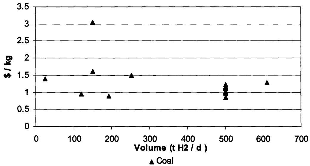
Figure 3.6: Cost estimates for hydrogen from coal gasification by size of plant.
