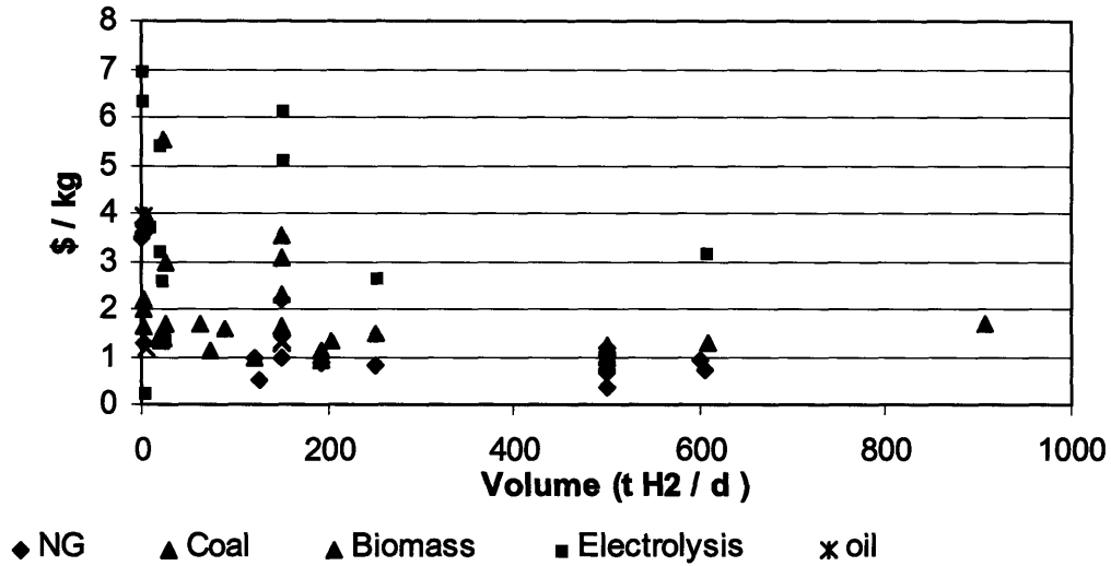
Figure 3.13: Cost estimates for hydrogen with all technologies by size of plant.
