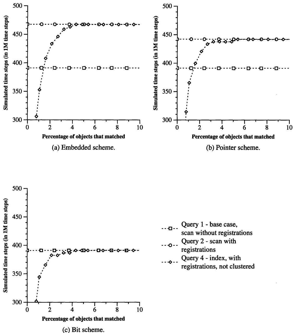
Figure 3.23: Detail of the results of Query 4 on the small DB3 with 8K segments with a cold cache.
