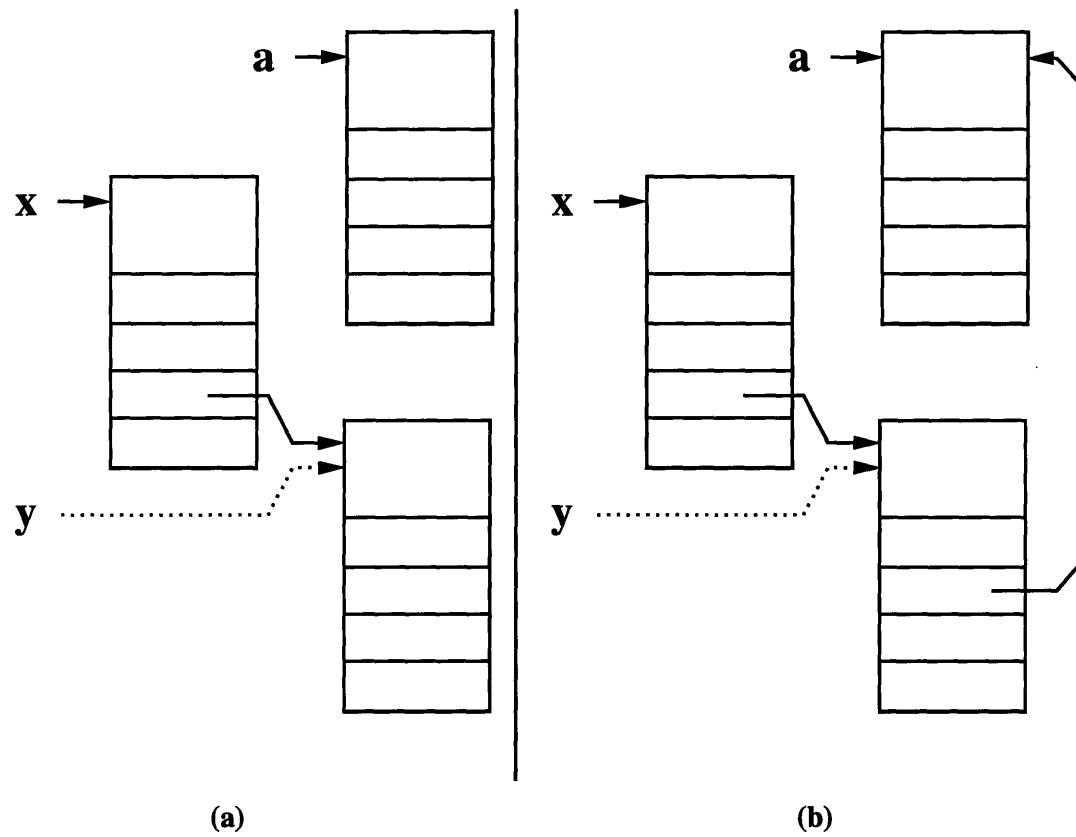
Figure 5.2: An example of how aliasing can happen: (a) after executing y := x[3] , (b) a possible outcome of y.foo(a) .
