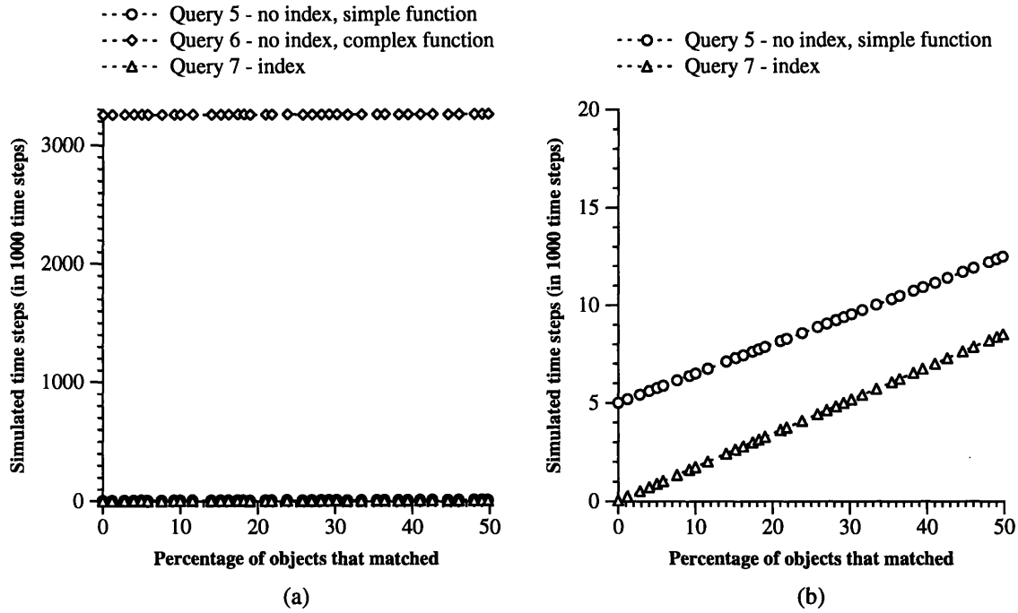
Figure 3.15: Results of Queries 5–7 for the small DB3 with 8K segments using bit scheme with a warm cache shown in graph (a). Graph (b) shows the details of the results of Query 5 and Query 7 on a different scale.
