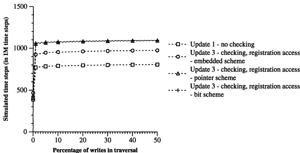
Figure 3.27: Comparison of results of Update 3 for the small DB3 with 8K segments with a cold cache.
