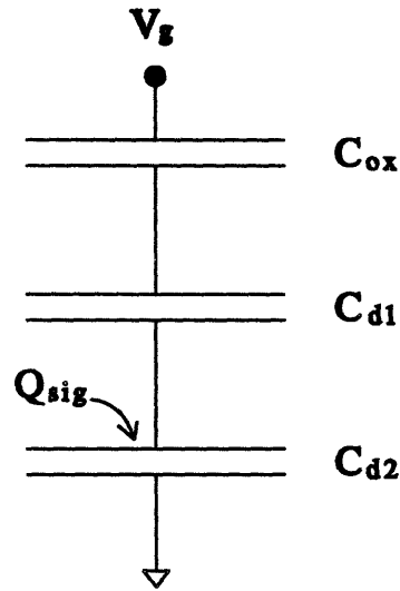
FIGURE 11-5: Lumped capacitance model of a BCCD
