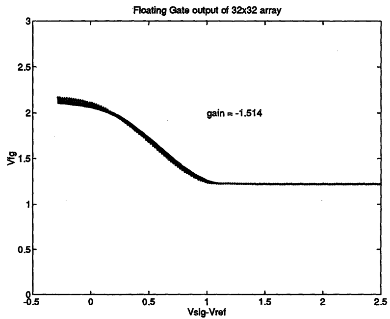
FIGURE 13-20: Floating-gate outputs of 32x32 array processor.
