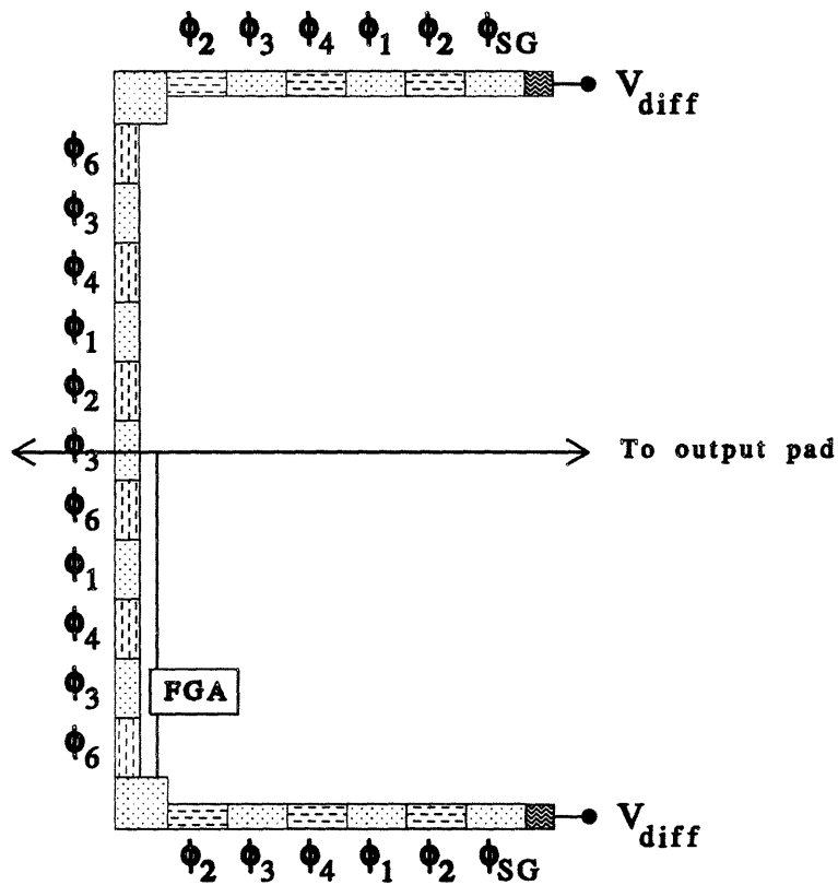
FIGURE 12-10: Boundary cell design (east).
