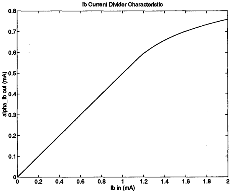
FIGURE 16-7: I_B current divider characteristic.
