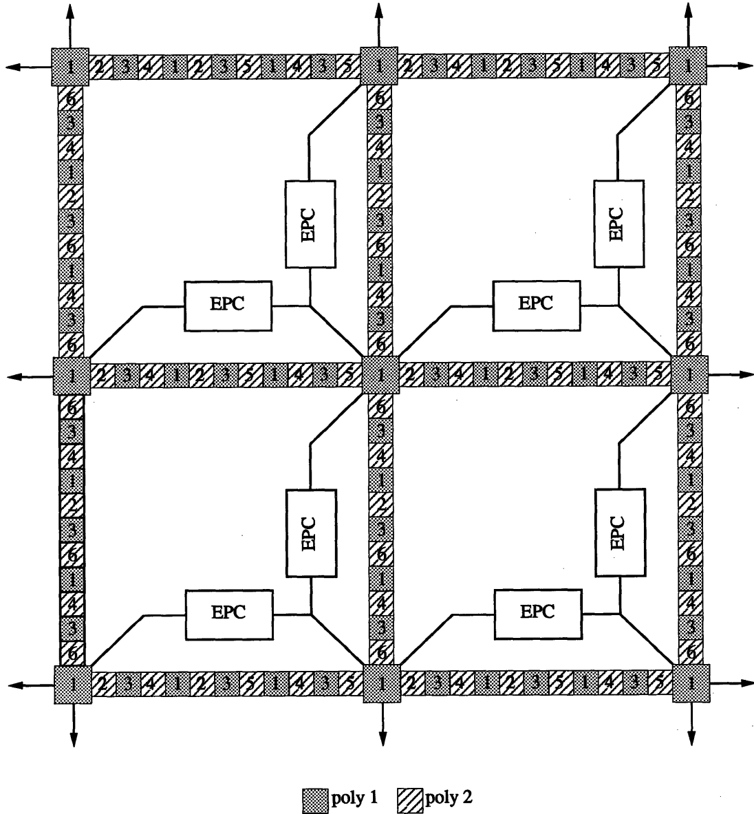
FIGURE 5-3: 2-D MSV edge detection array using charge-coupled devices (CCDs)
