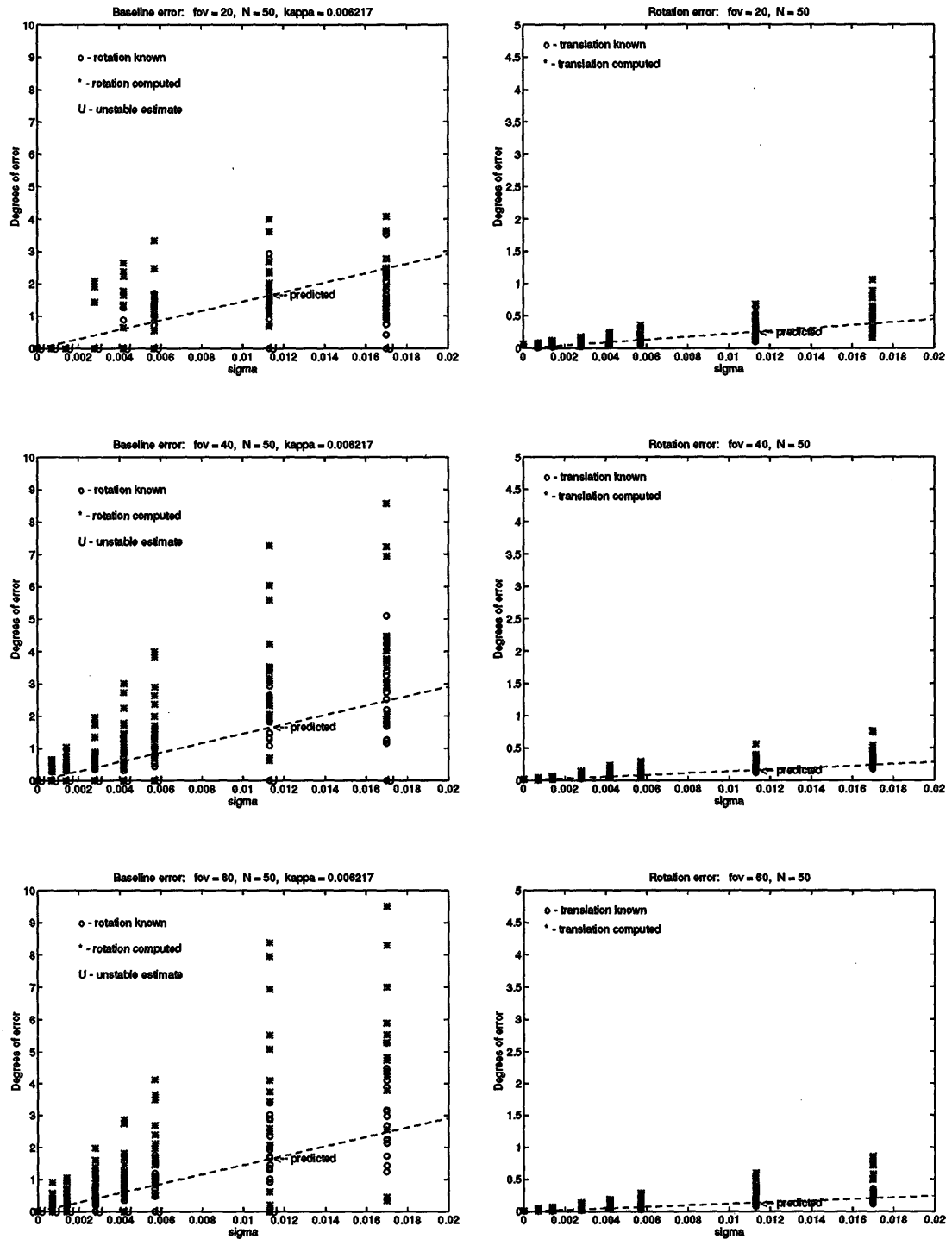
FIGURE 8-5: Estimation errors in translation and rotation with \mathbf{b} \parallel \hat{\mathbf{v}}_3 (uncorrelated measurement errors). \mathbf{b} = (0, 0, 1) , \hat{\boldsymbol{\omega}} = (0, 0, 1) , \theta = 5^\circ
