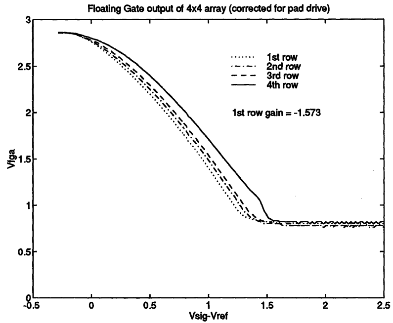
FIGURE 13-19: Floating-gate outputs of 4x4 array processor.
