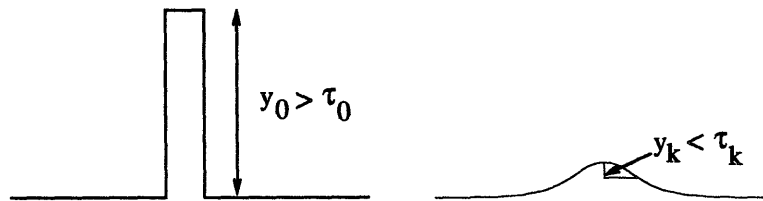
(b) Response to ideal point noise. The difference y_0 in the unsmoothed image is above threshold \tau_0 at n = 0 ; but the difference y_k in the smoothed image is below the threshold \tau_k . Hence no edge is marked.
