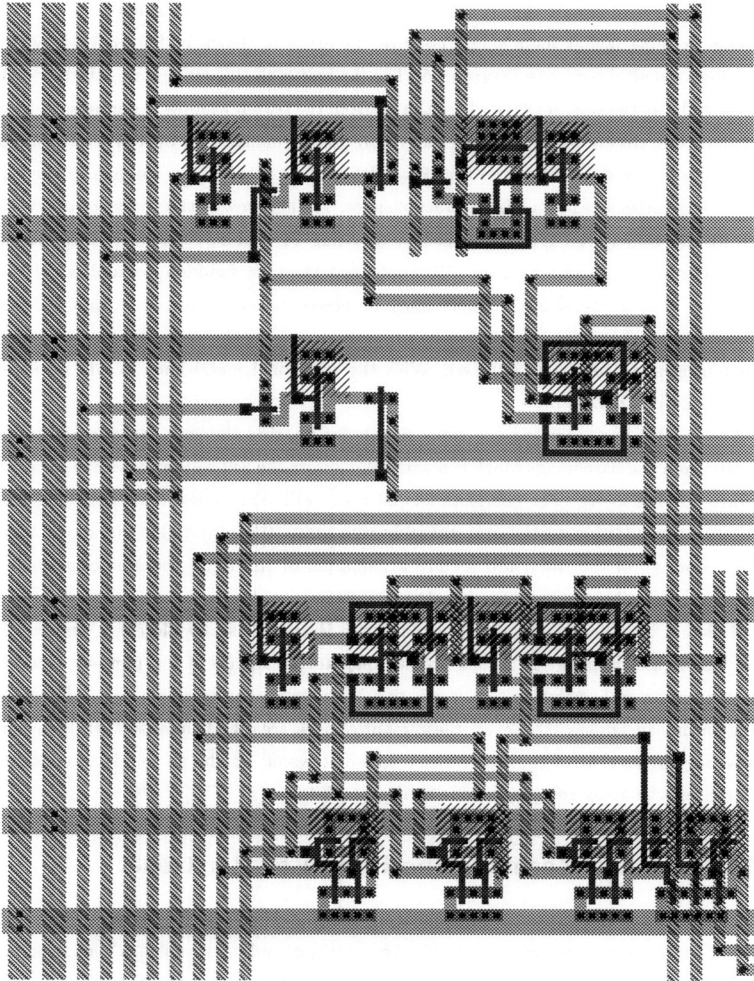
FIGURE 15-4: Layout of a unit cell including one full adder circuit.
