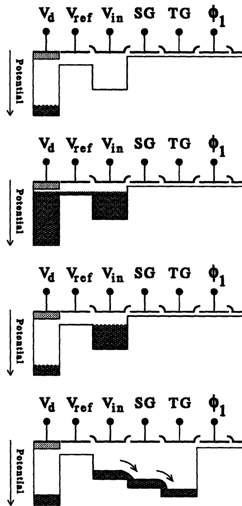
FIGURE 11-8: Fill-and-spill method for charge input
