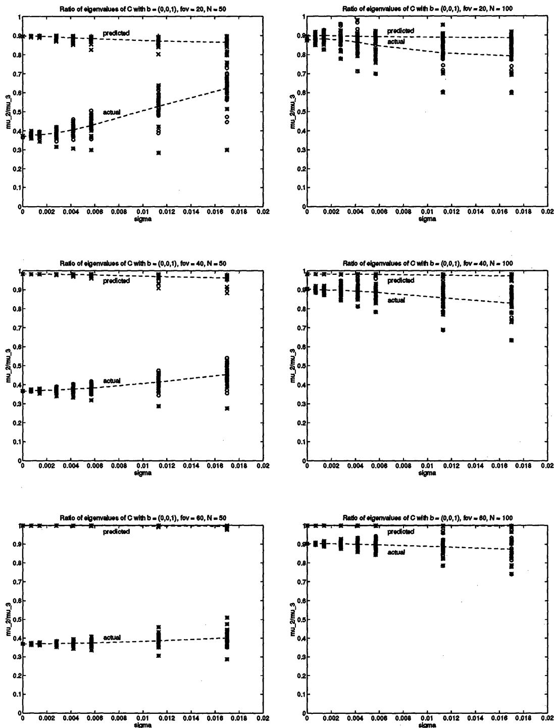
FIGURE 8-7: Actual and predicted values of \mu_2/\mu_3 for b \parallel \hat{v}_3 , for \phi = 20^\circ, 40^\circ , and 60^\circ with N = 50 and N = 100 .
