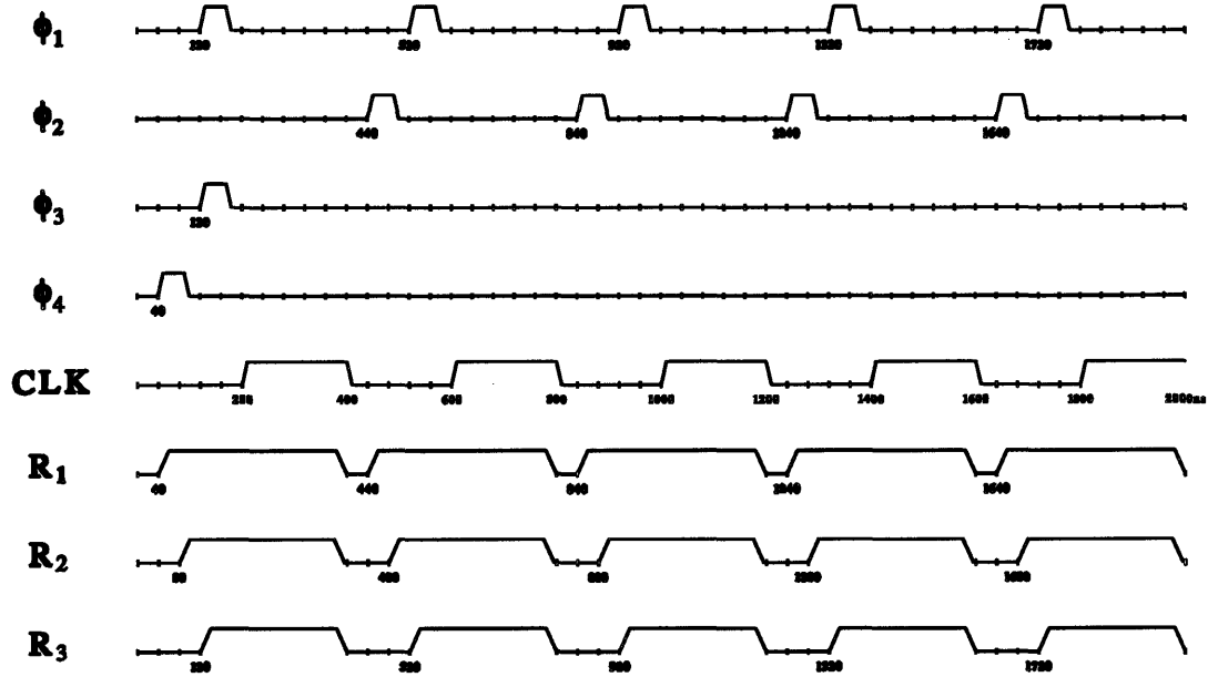
FIGURE 16-16: Clock waveforms.
