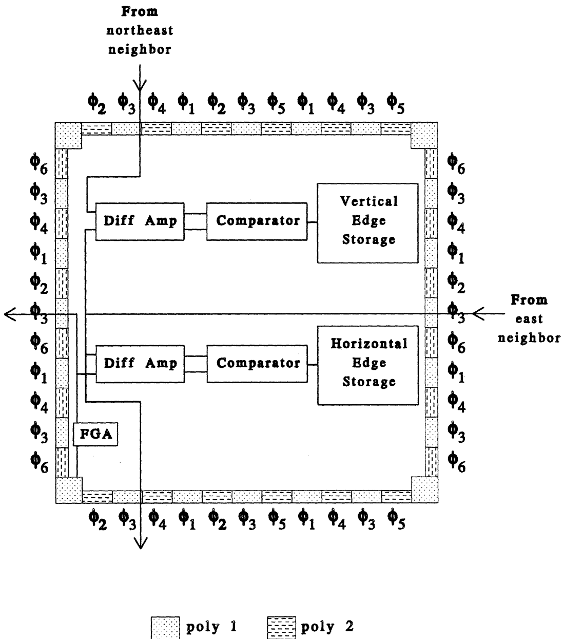
FIGURE 12-2: Unit cell architecture.
