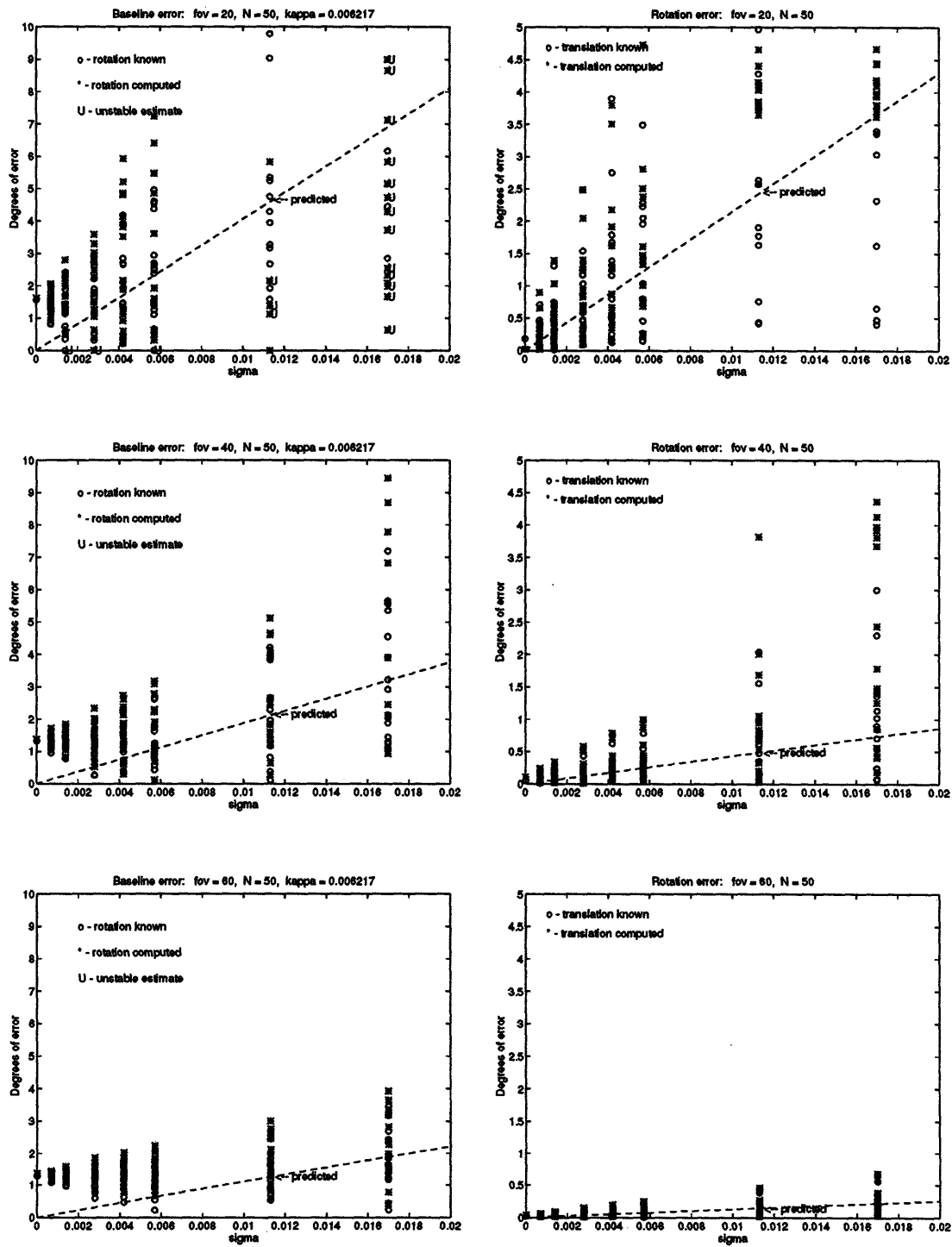
FIGURE 8-4: Estimation errors in translation and rotation with \mathbf{b} \perp \hat{\mathbf{v}}_3 (uncorrelated measurement errors). \mathbf{b} = (1, 0, 0) , \hat{\boldsymbol{\omega}} = (0, 0, 1) , \theta = 5^\circ
