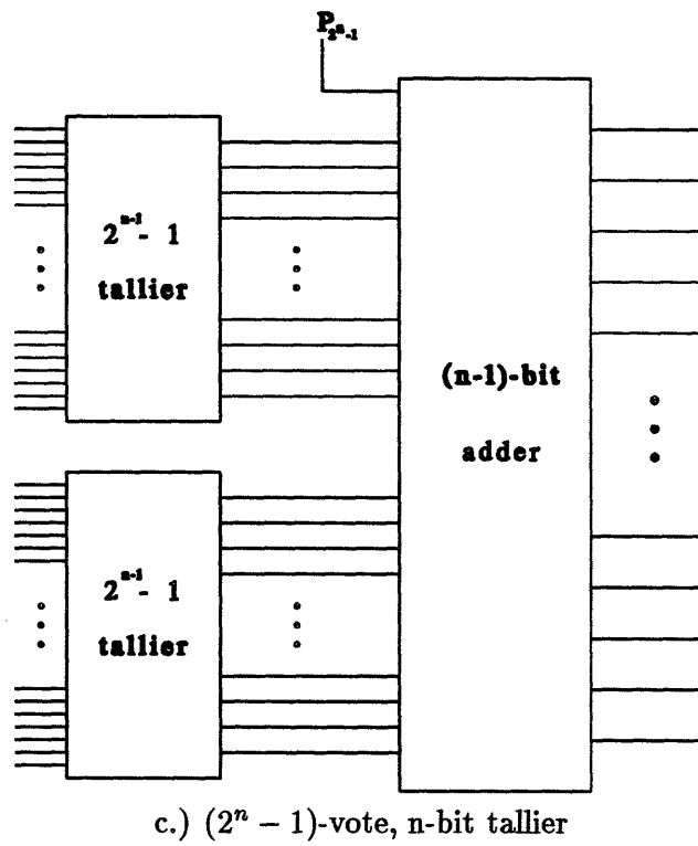
FIGURE 15-3: Tally circuit construction.
