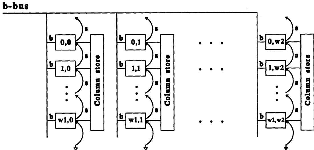
FIGURE 15-6: Offset processor array.
