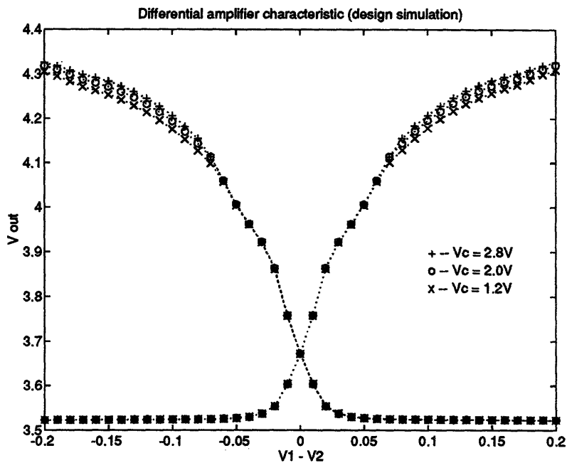
FIGURE 12-17: Simulated differential amplifier characteristic for common mode voltages V_c = 1.2V, 2.0V, and 2.8V ( V_{bias} = 1V ).
