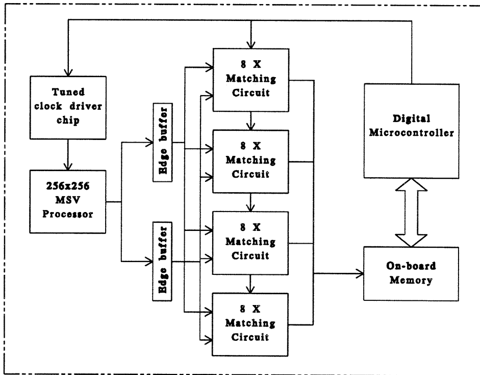
FIGURE 17-1: Single 'board' motion estimation system.
