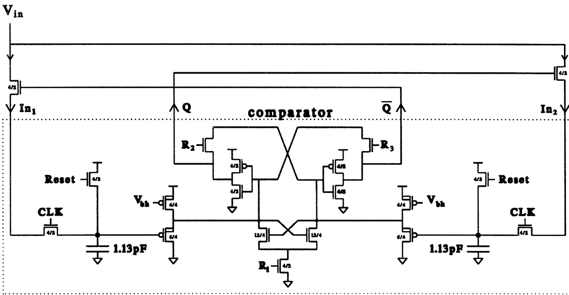
FIGURE 16-11: V_{min} circuit.
