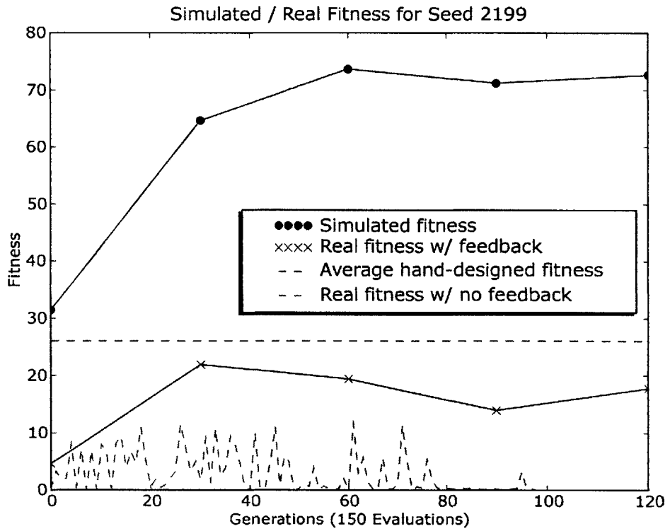
Figure 5-9: When feedback is incorporated into the evolutionary system, the resulting evolved controllers improve over time, approaching the average performance of the hand-designed algorithm. The bottom graph is the data from figure 5-5.
