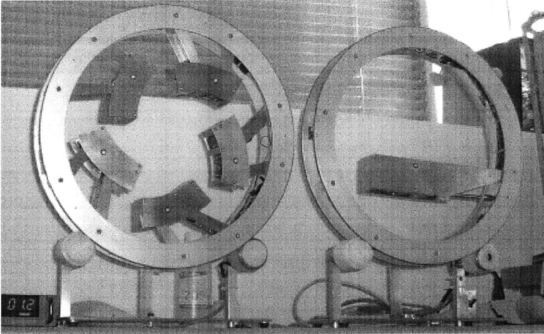
Figure 2-1: Julius Popp's robots, micro.adam (right) and micro.eva provide a unique problem domain for investigating evolved controllers.
