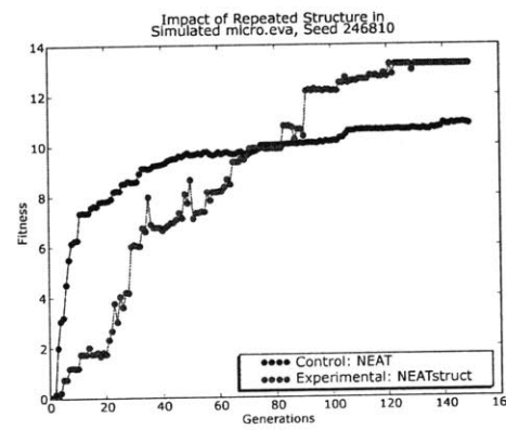
Figure 3-11: NEATstruct outperforms NEAT on simulated micro.eva .
