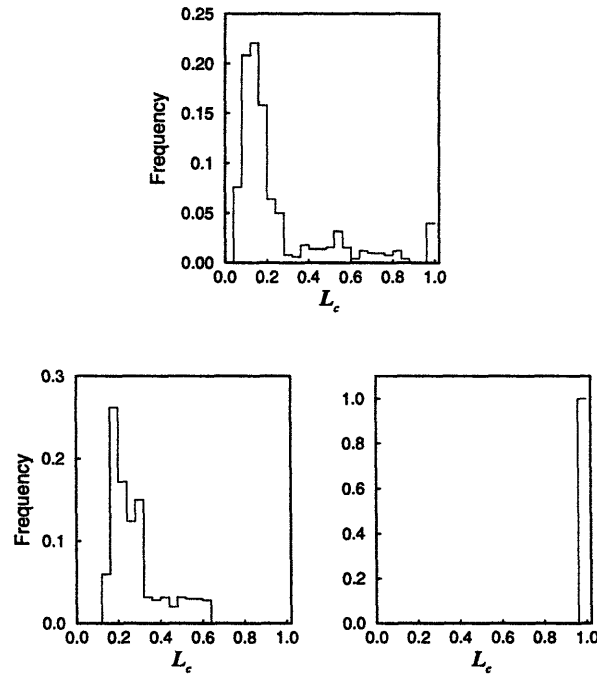
Figure 5-6: Histograms of characteristic scales for predator patterns. The diffusion coefficient is the same for all graphs. A and B differ in the slope of the gradient (in A: r(x) = -1.4x + 2 ; in B: r(x) = -0.1x + 0.7 ). A and C differ in the local dynamics that diffusion couples (in A: predator mortality m = 0.6 and diffusion couples local limit cycles; in B: m = 0.68 and diffusion couples local equilibria).
