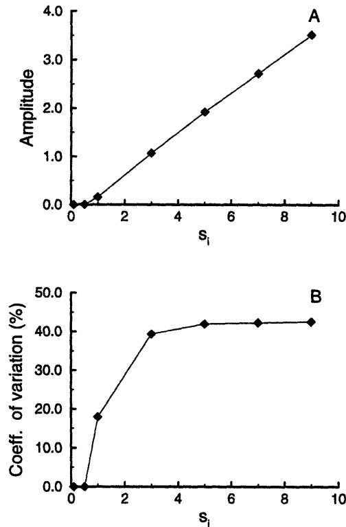
Figure 2-18: Bifurcation diagrams for an increasing nutrient inflow. As s_i increases the long-term dynamics of the system changes from a steady-state to a limit cycle. This is shown by plotting the amplitude (A) and the coefficient of variation (B) of total cell numbers for different values of s_i . ( v = 1 , U = 10 , d = 0.1 , [p_0, p_c] = [0.1, 0.4] .)
