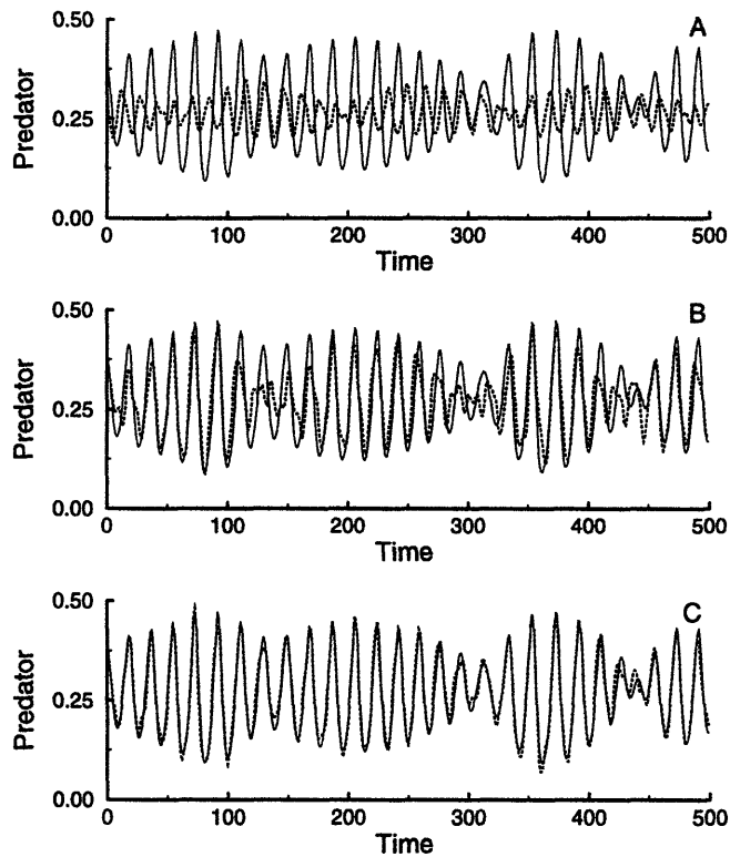
Figure 5-8: Approximation to chaotic solutions. Temporal solutions for predator numbers are shown at a fixed location in space, x = 0.85 , for d = 10^{-4} (continuous line). Approximations (dotted line) use an increasing number of modes from top to bottom (A: three modes; B: five modes; C: seven modes).
