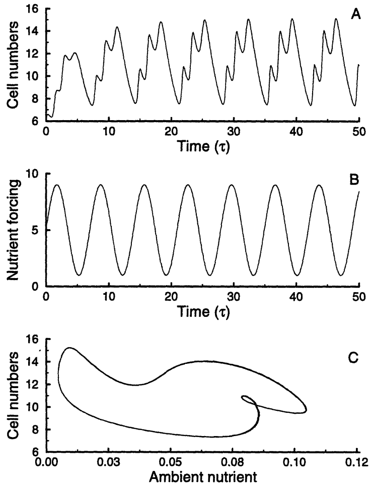
Figure 2-14: Periodic response to periodic forcing. Total cell numbers oscillates with the forcing frequency but displays multiple peaks in each cycle.
