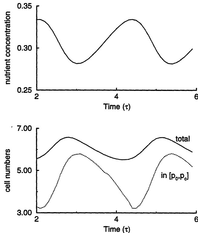
Figure 2-7: The anatomy of generation cycles. A complete oscillation of the model is shown for total cell numbers, cell numbers in the segment [p_0, p_c] , and ambient nutrient levels. The model oscillations involve changes in the population distribution. For a complete description of this figure see text (section 2.2.3). ( s_i = 5 , v = 1 , [p_0, p_c] = [0.1, 0.5] , d = 0.3 ).
