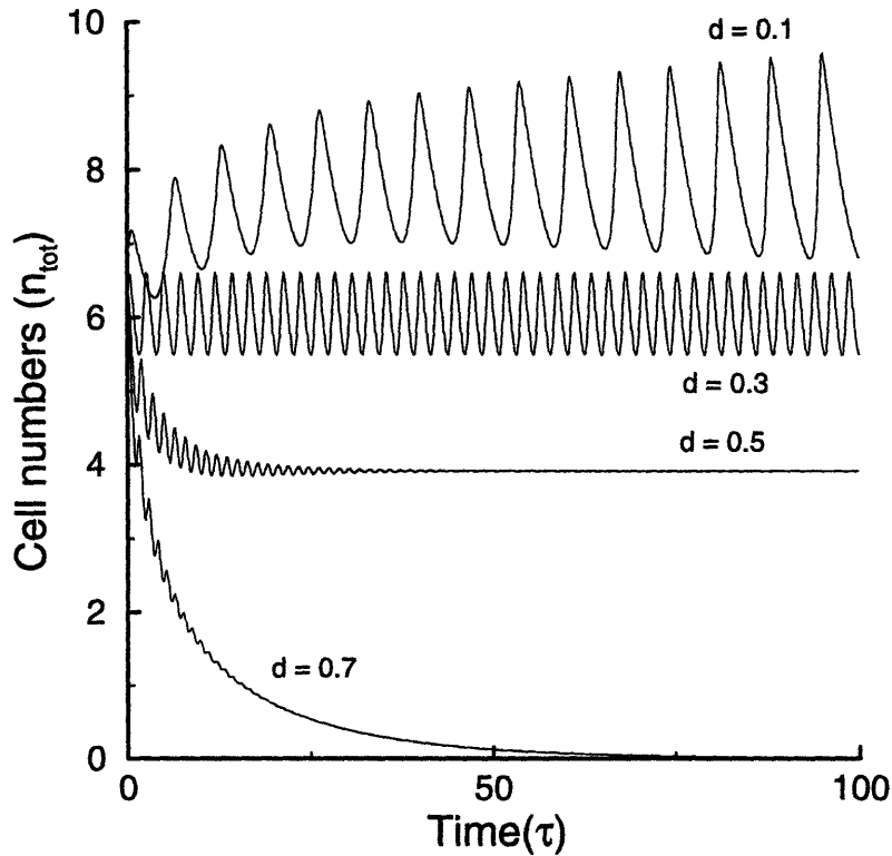
Figure 2-6: Oscillatory dynamics for low dilution rates. At low dilution rates the model converges to a limit cycle ( d = 0.3 and d = 0.1 ). For higher d = 0.5 , the population reaches a steady-state. For d = 0.7 , cell losses are too high for the population to persist in the chemostat. Initial conditions are the limit cycle for d = 0.3 . ( s_i = 5 , v = 1 , [p_0, p_c] = [0.1, 0.5] ).
