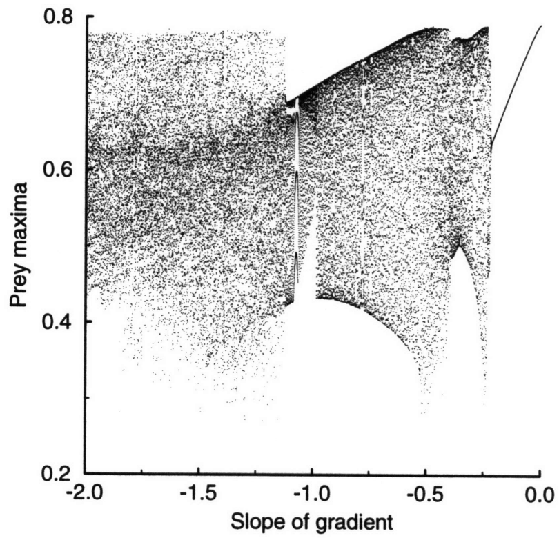
Figure 5-15: Bifurcation diagram for an increasing slope of the gradient. Prey maxima at a fixed location in space ( x = 0.85 ) are plotted for different values of the slope of the gradient
