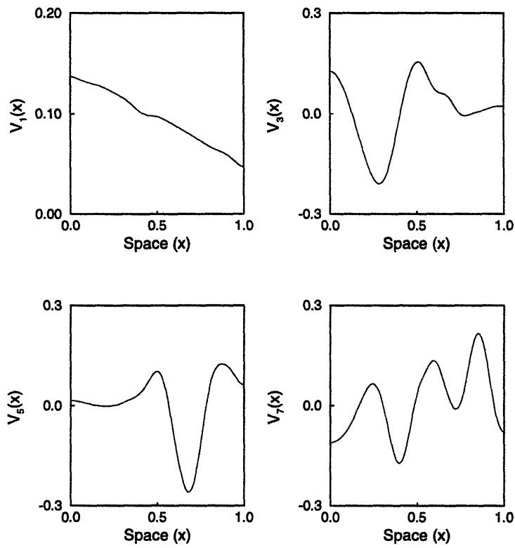
Figure 5-9: Orthogonal spatial functions for chaotic predator solutions ( d = 10^{-4} ). Only four of the seven functions used in the approximation of figure 5-8 are shown. See text for details.
