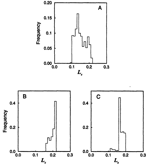
Figure 5-7: Histograms of characteristic scales for predator patterns with linear trend removed. A: d = 10^{-4} , chaotic dynamics; B: d = 10^{-3} , quasiperiodic dynamics; C: d = 10^{-2} , periodic dynamics.
