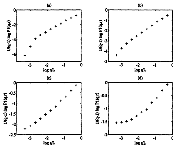
Figure 6-6: Scaling of moments for measure V1. \log P_1(q, r)^{\frac{1}{q-1}} vs. \log r/L for representative values of q : (a): q = -3 , (b): q = -1 , (c): q = +1.25 , and (d): q = +3 .
