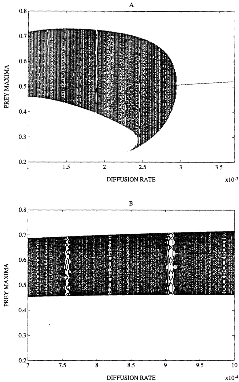
Figure 4-4: Bifurcation diagrams. Successive maxima of prey density at x = 0.85 are plotted for increasing values of the diffusion rate after transients have died out. (In (a), values of d differ by 10^{-5} , in (b), by 10^{-6} .)
