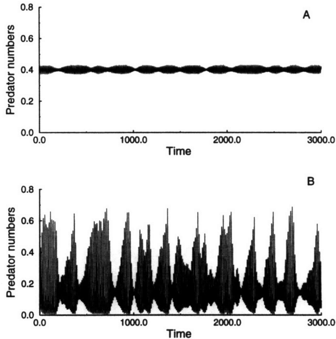
Figure 5-14: Temporal behavior of predator numbers. Two spatial locations in figure 5-13 are chosen to illustrate the long-term temporal dynamics of the system (A: x = 0.95 ; B: x = 0.15 ). Predator patterns are irregular at both locations but appear strongly damped in amplitude at the end of the gradient where diffusion couples equilibria.
