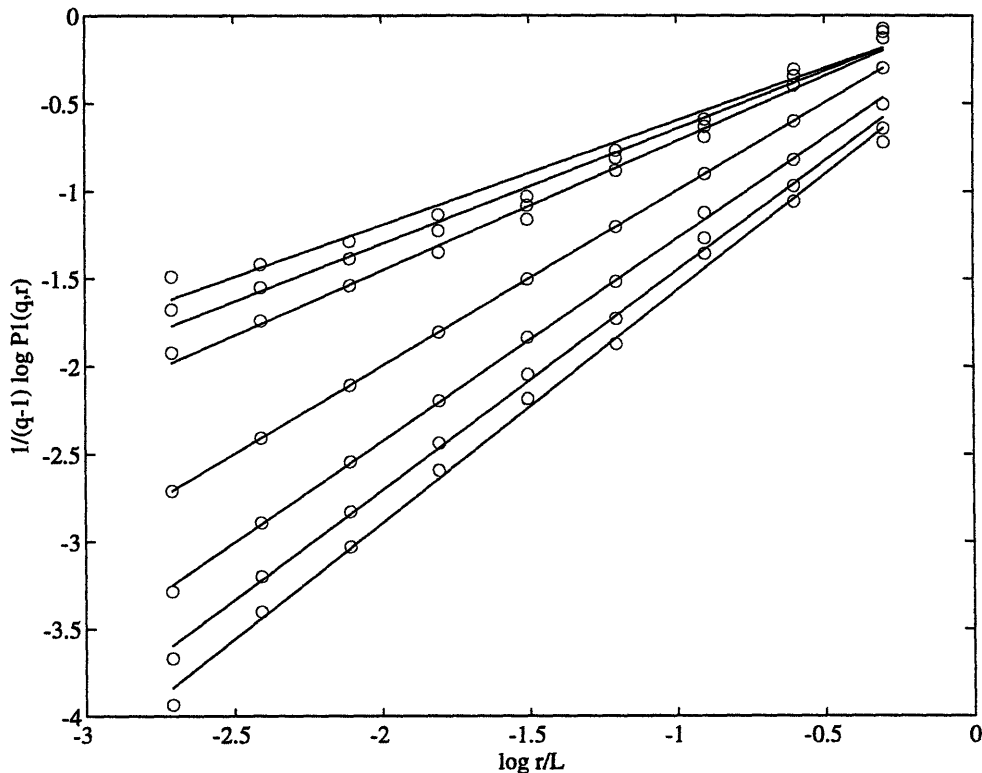
Figure 6-8: Scaling region for moments of V_1 . The lines are the least-square fit through the data points. From bottom to top q values are -3, -2, -1, 0, +1.25, +2, +3 .
