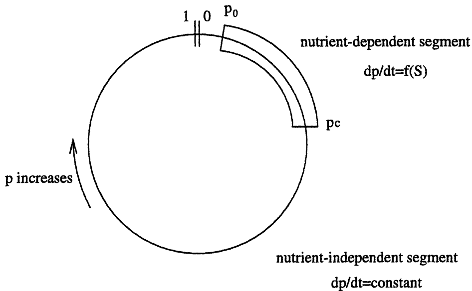
Figure 2-2: Conceptual representation of the cell cycle. In the model, a variable p indicates the position of a cell along the cell cycle. The interval [p_0, p_c] is a nutrient-dependent segment during which progression of a cell through the cycle depends on nutrient levels. In the rest of the cycle, cells progress at a constant rate. Thus, once a cell reaches p_c , it proceeds towards division regardless of nutrient conditions.
