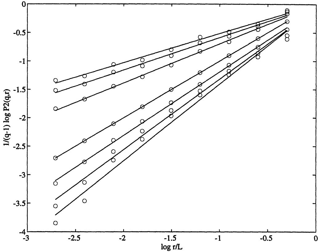
Figure 6-9: Scaling region for moments of V_2 . The lines are the least-square fit through the data points. From bottom to top q values are -3, -2, -1, 0, +1.25, +2, +3 .
