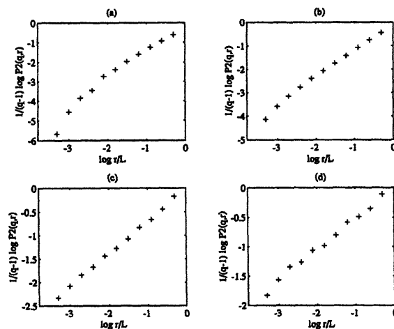
Figure 6-7: Scaling of moments for measure V2. \log P_2(q, r)^{\frac{1}{q-1}} vs. \log r/L for representative values of q : (a): q = -3 , (b): q = -1 , (c): q = +1.25 , and (d): q = +3 .
