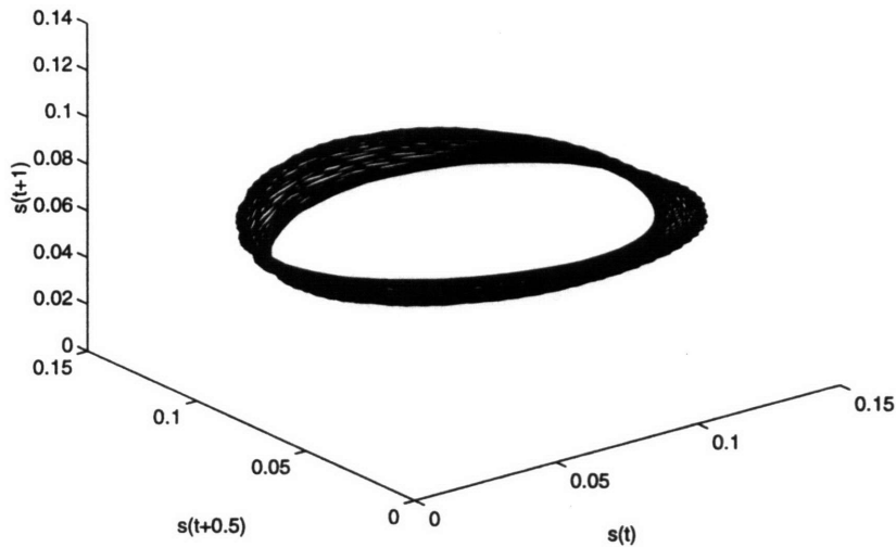
Figure 2-10: Torus attractor. The attractor of the system is reconstructed by plotting one of the variables, the ambient nutrient s , against itself at lagged intervals of time after transients have died out. The trajectory moves on the surface of a torus. ( s_i = 5 , v = 1 , [p_0, p_c] = [0.1, 0.5] , d = 0.3 , \epsilon = 0.9 , \omega = 4.5 ).
