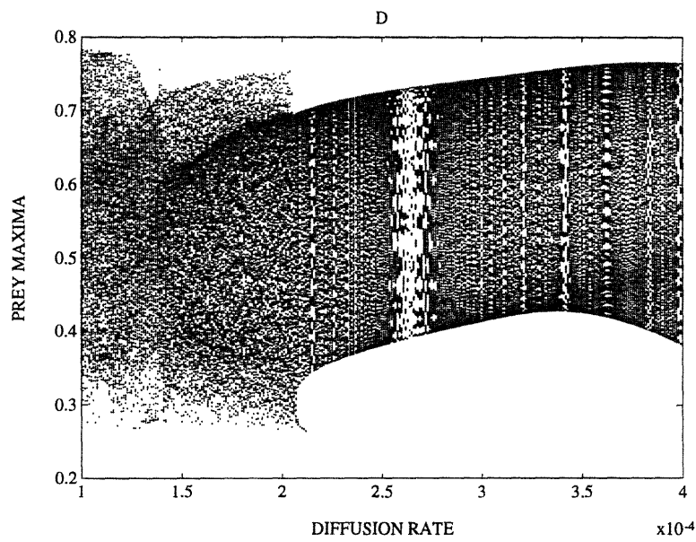
Figure 4-5: Bifurcation diagrams (cont.). Successive maxima of prey density at x = 0.85 are plotted for increasing values of the diffusion rate after transients have died out. (Values of d differ by 10^{-6} )
