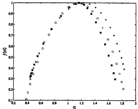
Figure 6-12: Comparison of the curve f(\alpha) for V_2 in three different data sets: (+), time series A, (o), time series B, and (*), time series C.
