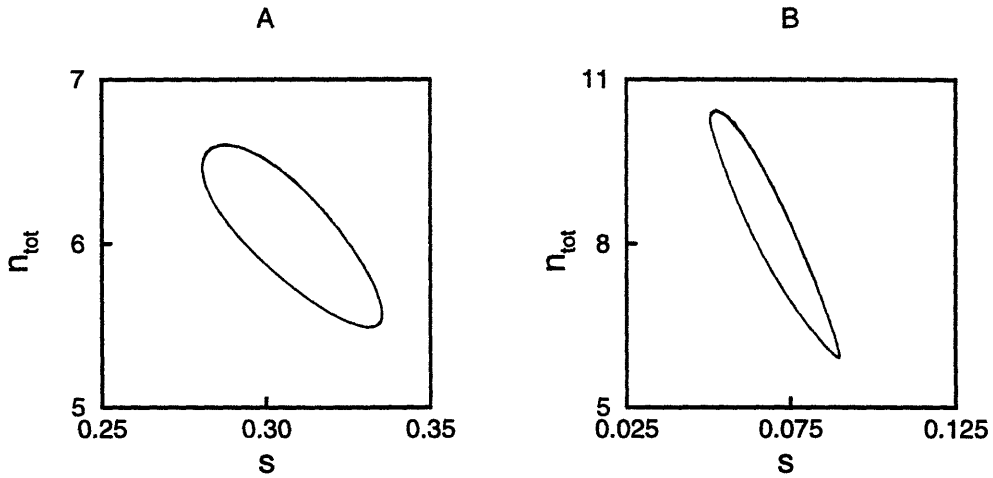
Figure 2-5: Limit cycles. Total cell numbers vs. ambient nutrient levels after transients have died out. In (A), d = 0.3 ; in (B), d = 0.1 . ( s_i = 5 , v = 1 , [p_0, p_c] = [0.1, 0.5] ).
