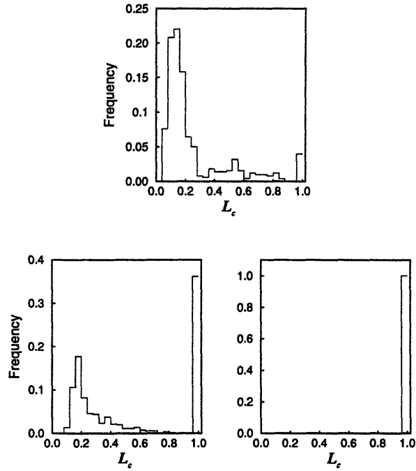
Figure 5-5: Histograms of characteristic scales for predator patterns. A: d = 10^{-4} , chaotic dynamics; B: d = 10^{-3} , quasiperiodic dynamics; C: d = 10^{-2} , periodic dynamics.
