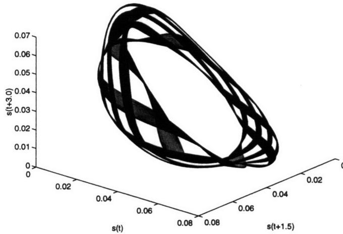
Figure 2-23: Torus attractor. The attractor of the system can be reconstructed by plotting one of the variables, the ambient nutrient s , against itself at lagged intervals of time after transients have been removed. Three dimensions ( s(\tau) , s(\tau + 1.5) and s(\tau + 3) ) suffice to reconstruct the attractor since trajectories move on the surface of a torus. ( v = 1 , U = 10 , s_i = 5 , d = 0.2 , [p_0, p_c] = [0.1, 0.4] , \epsilon = 0.9 , \omega = 1 ).
