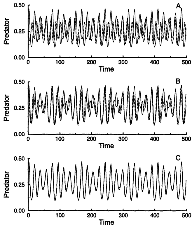
Figure 5-10: Approximation to quasiperiodic solutions. Temporal solutions for predator numbers are shown at a fixed location in space, x = 0.85 , for d = 10^{-3} (continuous line). Approximations (dotted line) use an increasing number of modes from top to bottom (A: one mode; B: two modes; C: three modes).
