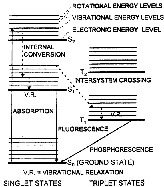
Figure 1.5- Jablonski diagram
