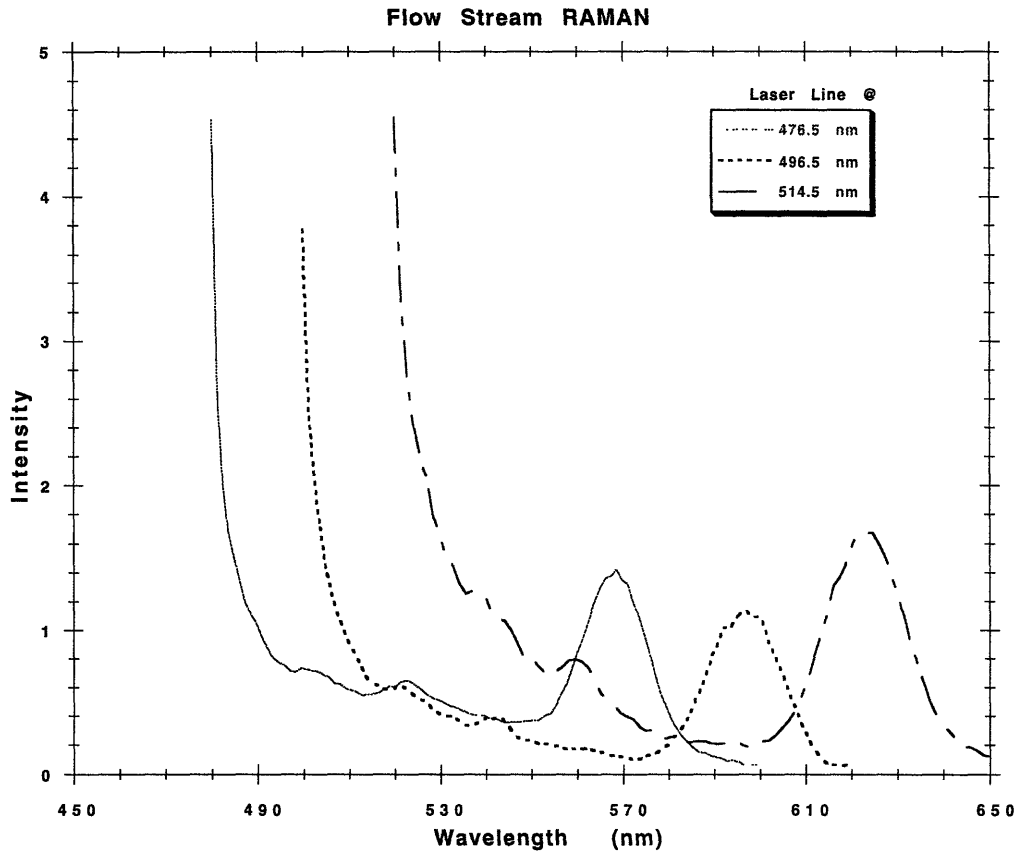
Figure 4.2- Wavelength scans for Raman scattering of water
