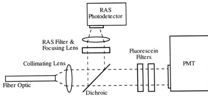
Figure 2.2 - Optics package schematic
