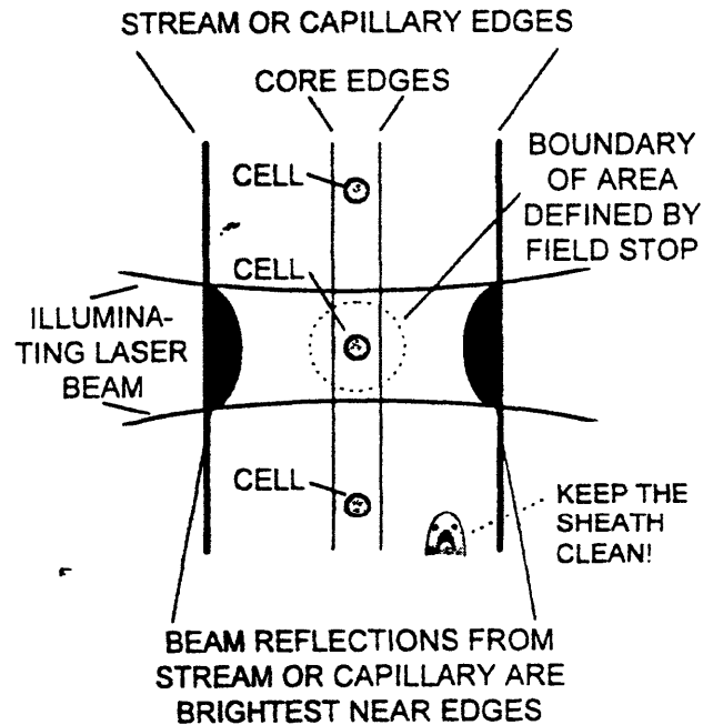
Figure 1.7- Observation point
