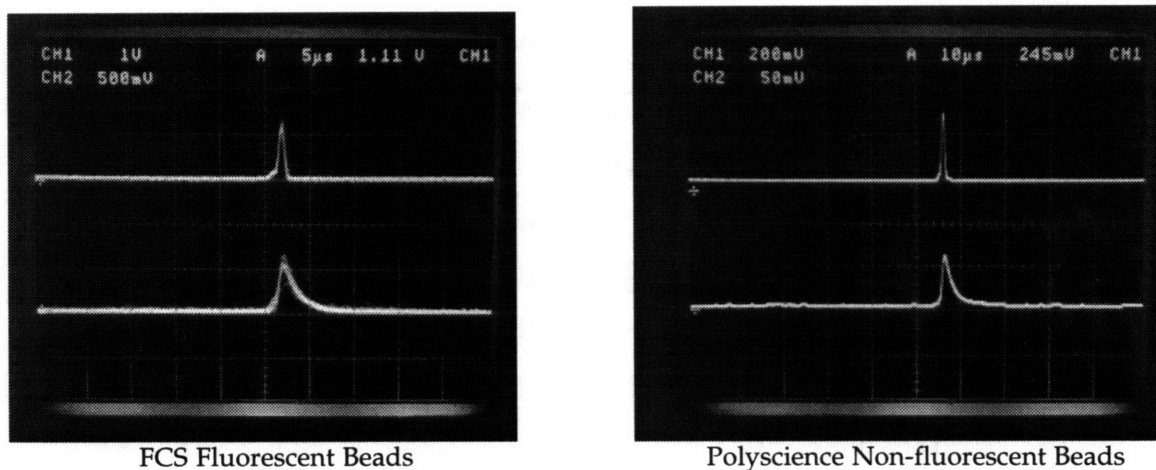
Figure 4.12 - Oscilloscope signals of FCS fluorescent and Polyscience non-fluorescent beads with 13” fiber optic
