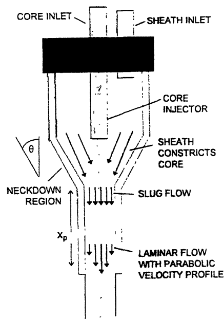
Figure 1.8 - Flow nozzle
