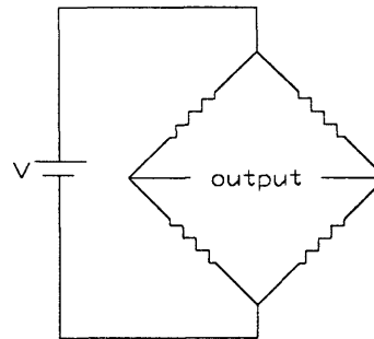
Fig 5.6 Wheatstone Bridge
