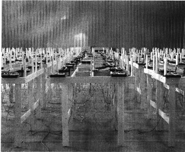
Figure 4-1: Kansei is a testbed of 210 Extreme Scale Motes (XSM) hooked individually onto 210 Extreme Scale Stargates (XSS). This provides a test bed infrastructure to conduct experiments with 802.11b networking and XSMs. The picture is taken from Kansei's homepage http://ceti.cse.ohio-state.edu/kansei/
