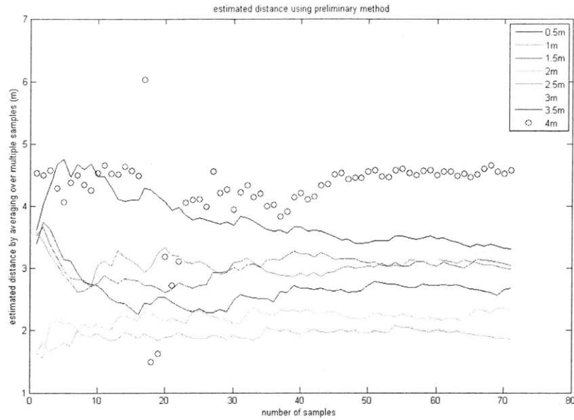
Figure 5-1: The estimated pair-wise distance average over many samples using preliminary methods which were ruled out for its poor performance. x -axis represents number of samples taken and y -axis represents the estimated distance in m .
