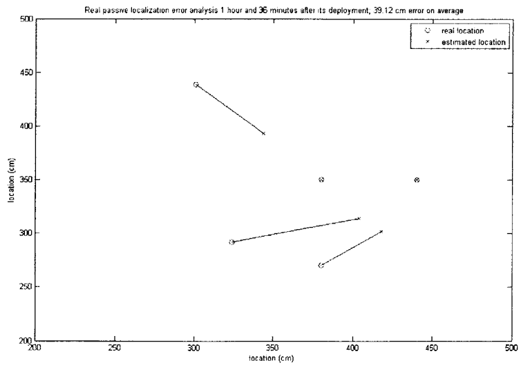
Figure 6-11: Error analysis for passive localiton 1 hour and 36 minutes after the PLUGs have been deployed. It has 39.12cm error on average.
