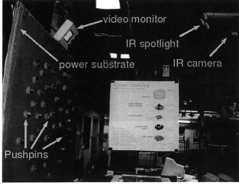
Figure 3-2: Pushpin experimental setup. This includes an IR spotlight for synchronization and parallel programming. An IR sensitive camera and video monitor are used to display the IR communication path. This picture is excerpted from Broxton's thesis [8].
