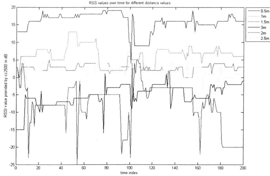
Figure 5-8: RSS values for different pair-wise distance values when a cellular phone is nearby. The noisy RSSI values most probably result from other radio signals and multipath effects.
