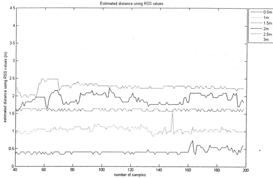
Figure 5-7: Estimated distance using Equation 5.2 and RSS values for different pair-wise distance values in relative radio silence.
