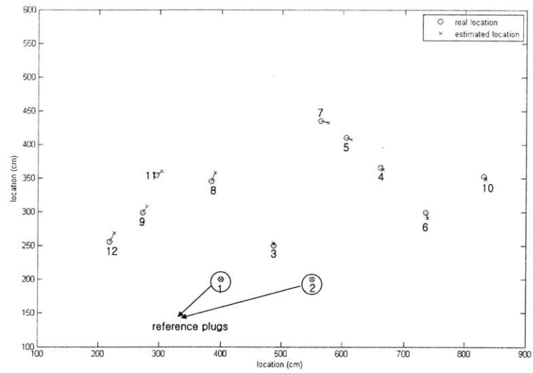
Figure 6-6: Error analysis plot for simulated active localization. The error is 7.97cm on average.
