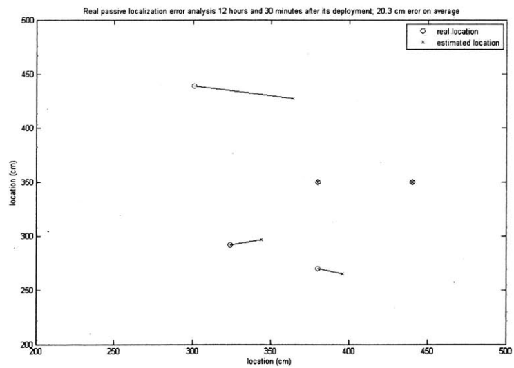
Figure 6-12: Error analysis for passive location 12 hours and 30 minutes after the PLUGs have been deployed. It has 20.3cm error on average.
