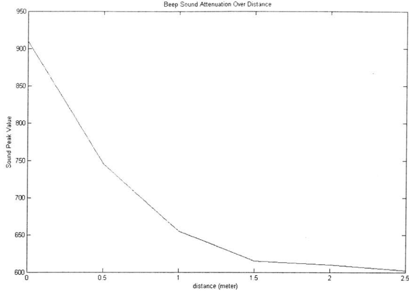
Figure 5-11: Sound Peak value vs pair-wise distance
