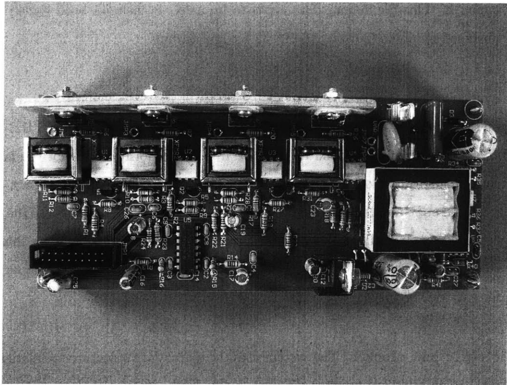
Figure 4-4: High-Voltage Part for PLUG
