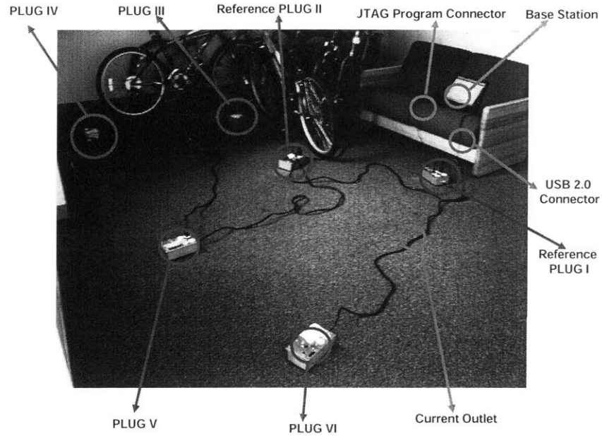
Figure 6-8: Deployment for active and passive localization test. This figure is annotated with base station, 2.0 USB connector for data collection, and 6 PLUGs connected each other for power. The PLUG5 was unlocalized due to its hardware failure.
