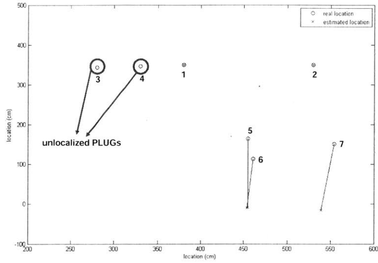
(a) Localization using RSS
