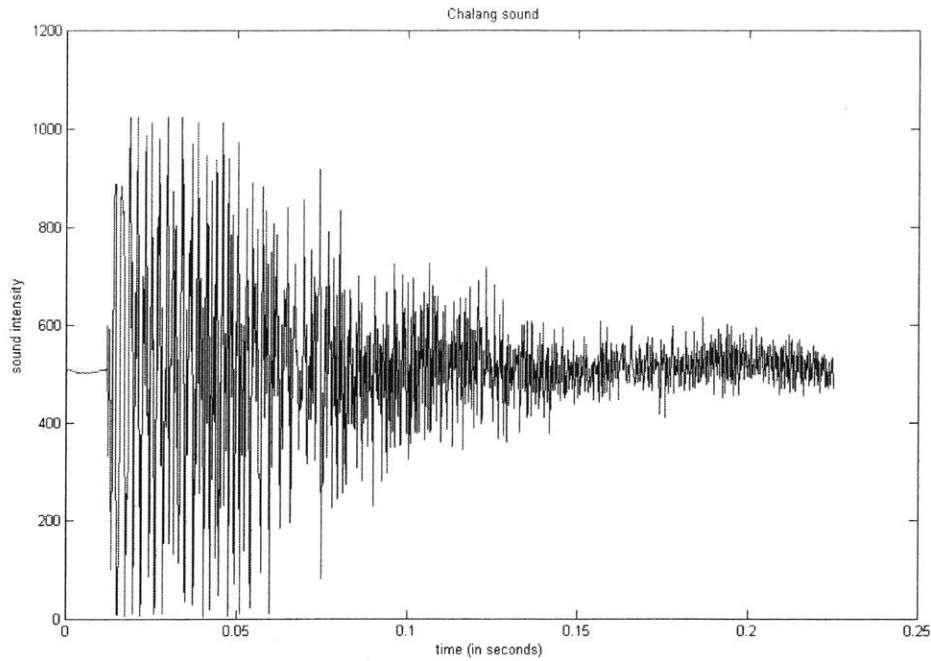
Figure 5-5: “chalang” sound when two glasses touch
