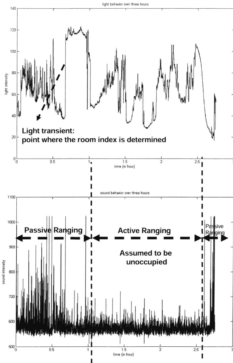
Figure 5-3: Light and Sound behavior over three hours: As explained in Section 5.6.2, the room index is determined when the light transient happens. ranging scheme alternates between active and passive depending on whether the surrounding is silent or not.
