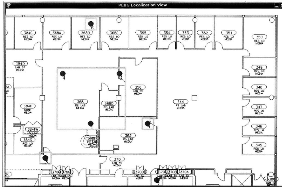
Figure 6-3: PLUG 1, 3, and 4 are determined to be in the same room. PLUG 2, 5, 6, and 7 are determined to be in the different room.
