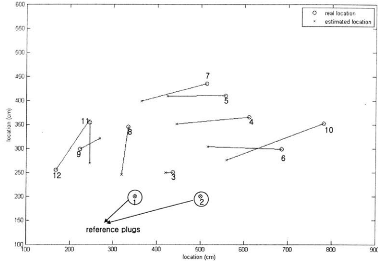
Figure 6-7: Error analysis plot for simulated passive localization. The error is 103.06cm on average.
