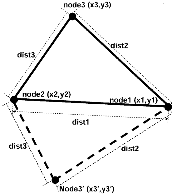
Figure 5-12: For easy illustration of linear localization algorithm
