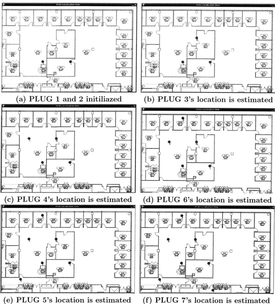
Figure 6-5: Steps for simulated active localization: (a) PLUG 1 and PLUG 2 are reference points. Thus, these two points are already given even before the localization algorithm starts. (b) Based on the positions of PLUG 1 and 2 and received distance information, PLUG 3's location is calculated. (c) Based on the positions of PLUG 1 and 3 and received distance information, PLUG 4's location is calculated. (d) Based on the positions of PLUG 3 and 4 and received distance information, PLUG 6's location is calculated. (e) Based on the positions of PLUG 1 and 4 and received distance information, PLUG 5's location is calculated. (f) Based on the positions of PLUG 2 and 5 and received distance information, PLUG 7's location is calculated.
