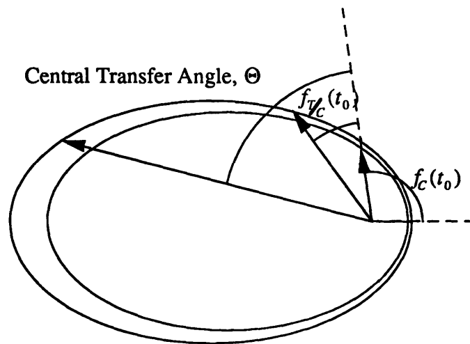
Figure 3.9 True Anomaly and Central Transfer Angle for Elliptic Orbits
