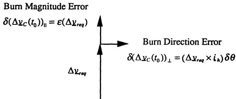
Figure 3.1 Burn Magnitude and Direction Errors
