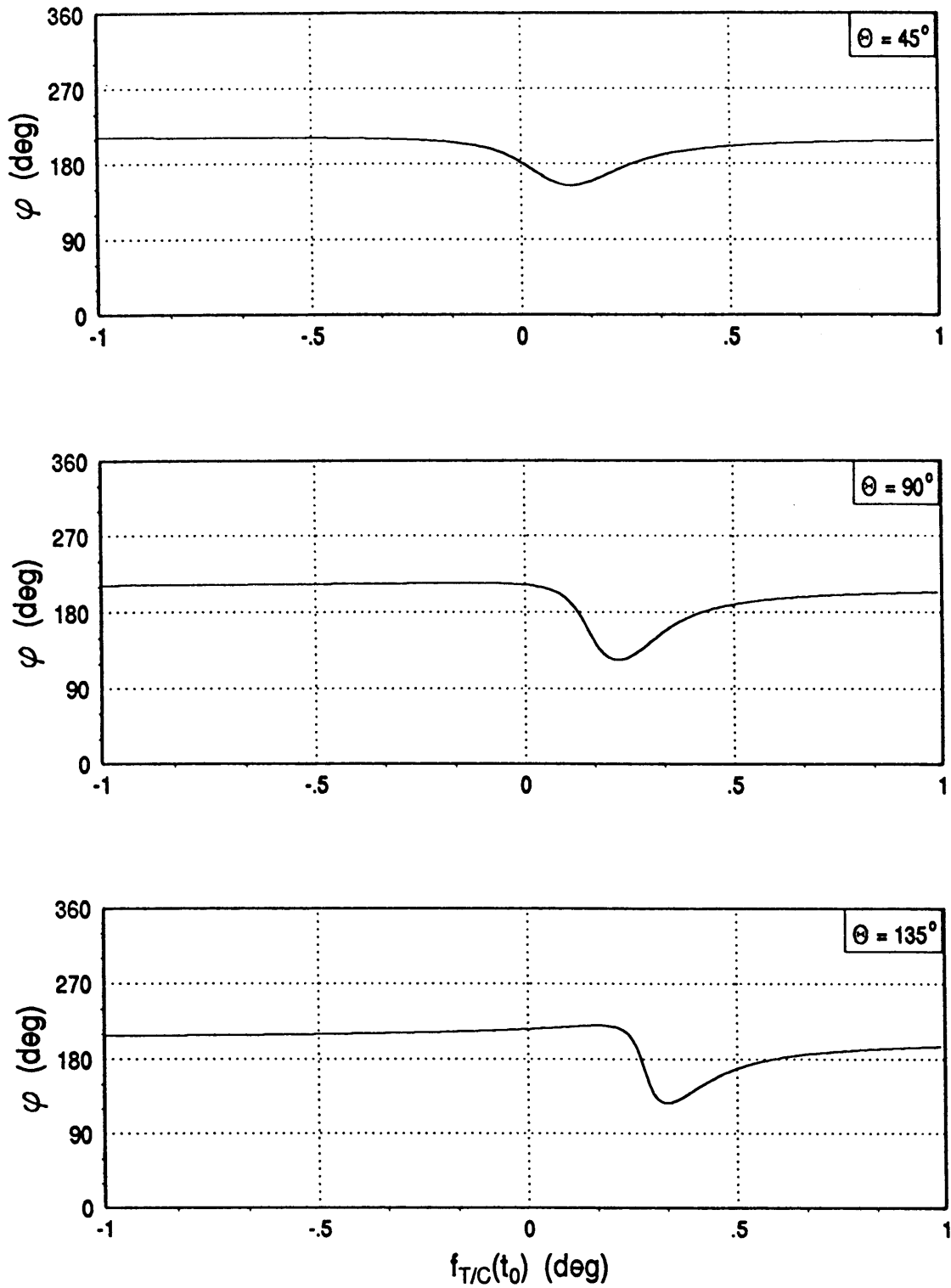
Figure 3.11 Variation in \phi --Burn Magnitude and Direction Error, Scaled Elliptic Staging Orbit
