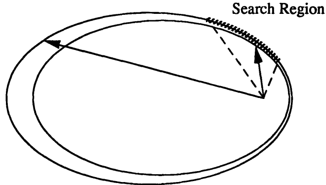
Figure 3.10 Search Region for Elliptic Orbits
