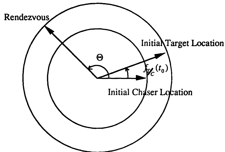
Figure 3.2 True Anomaly and Central Transfer Angle
