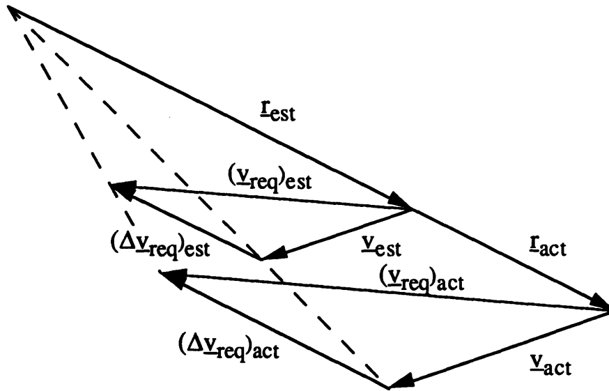
Figure 4.5 Scaled Relative Geometry Error Results in Burn Magnitude Error
