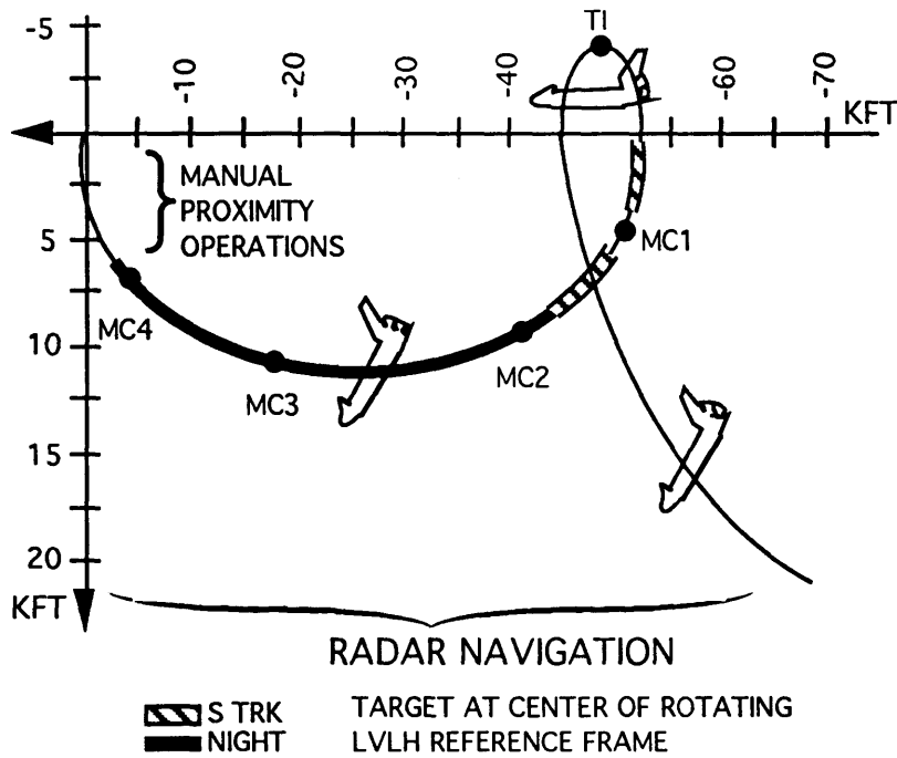
Figure 1.2 Shuttle Rendezvous Profile
