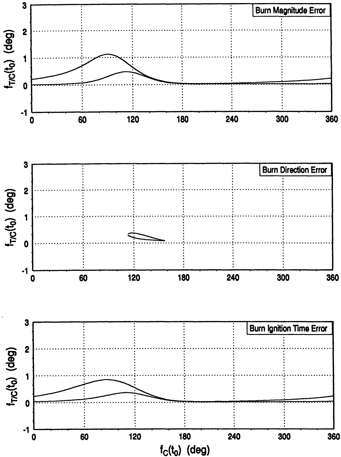
Figure C.1 Maneuver Points Providing Burn Execution Error Tolerance for Scaled Elliptic Staging Orbit and 90° Central Transfer Angle
