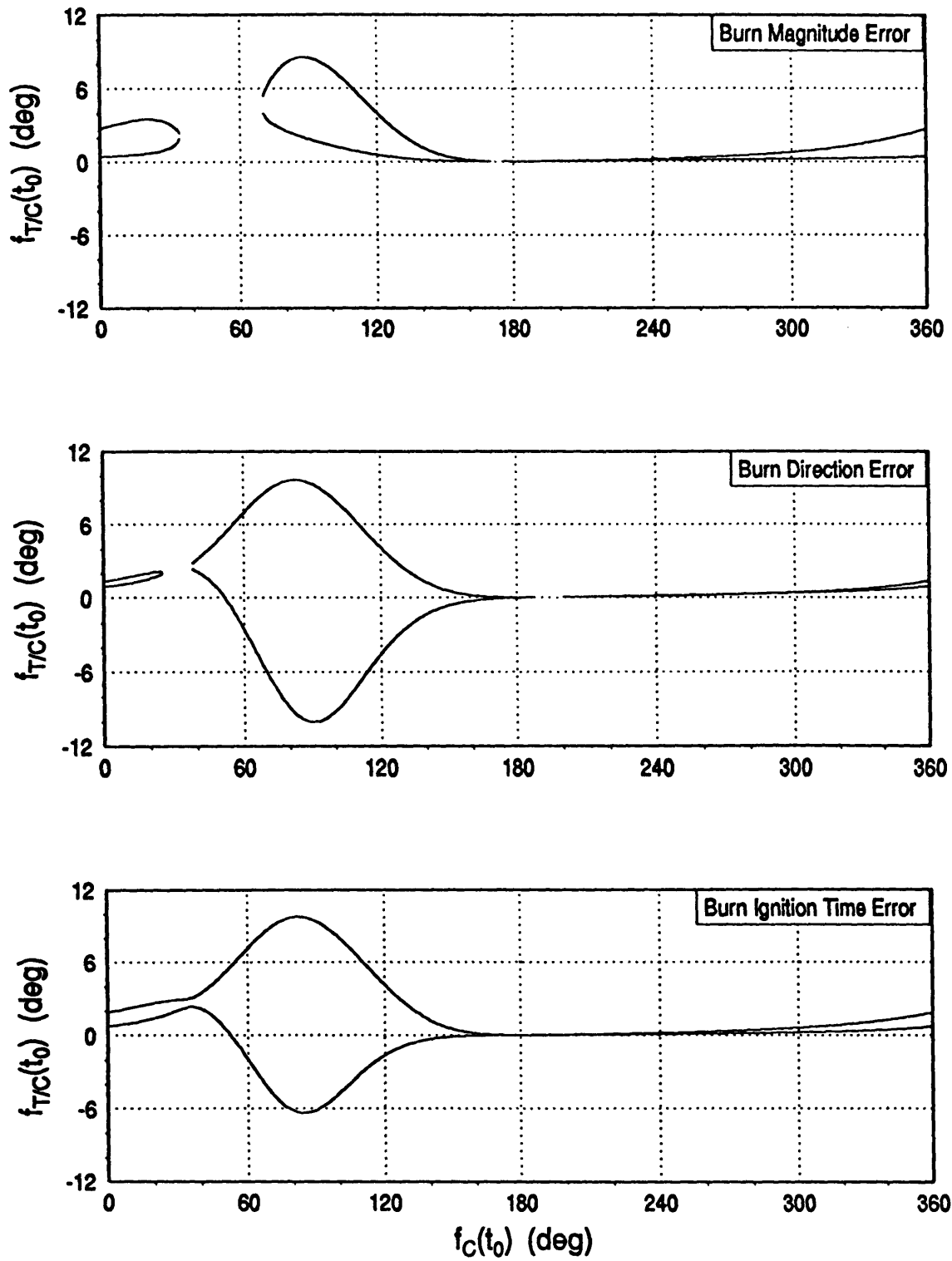
Figure 3.14 Burn Execution Error Tolerant Maneuver Points for Coelliptic Staging Orbit and 135° Central Transfer Angle
