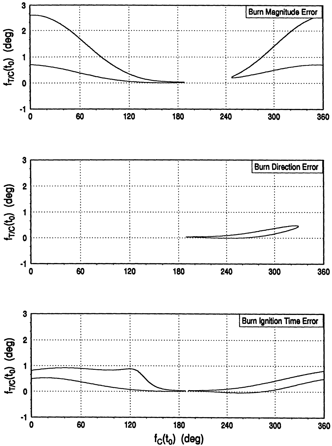
Figure C.2 Maneuver Points Providing Burn Execution Error Tolerance for Scaled Elliptic Staging Orbit and Transfer Time = 3/8 P_T
