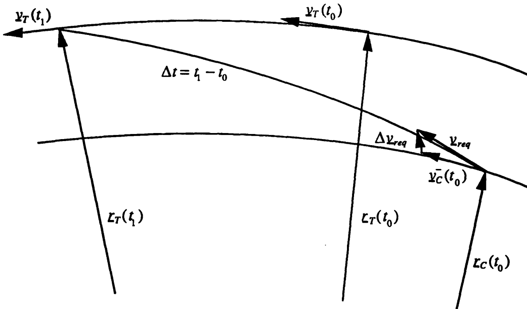
Figure 2.1 Rendezvous in Inertial Coordinates
