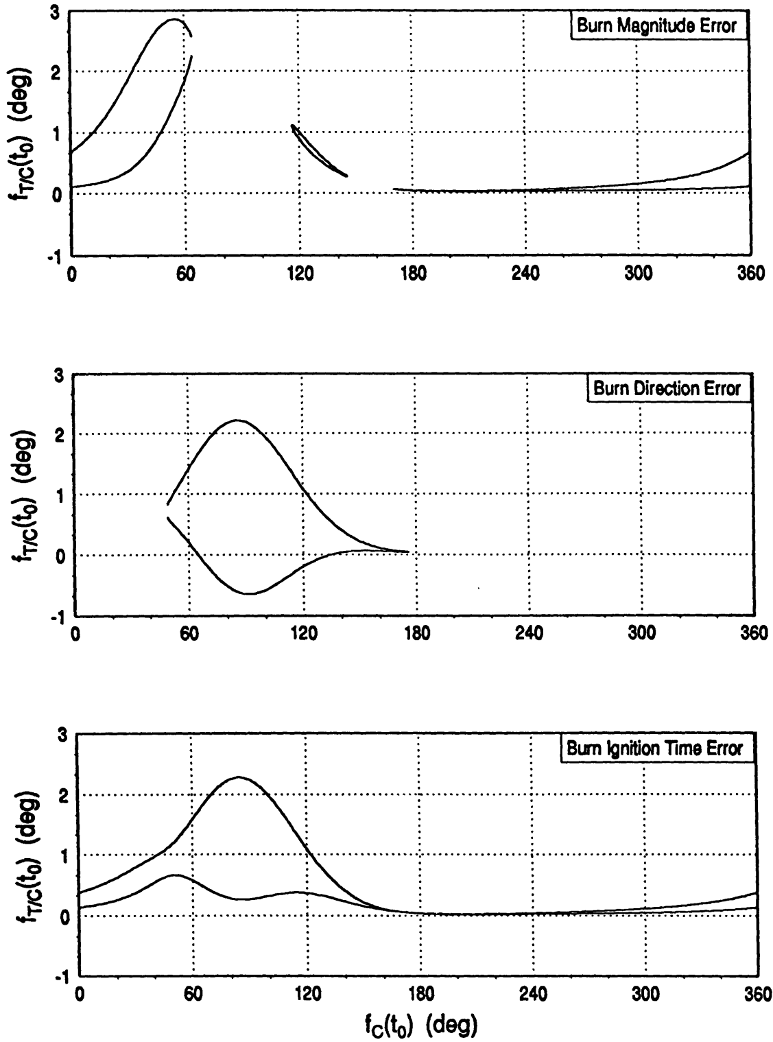
Figure 3.12 Burn Execution Error Tolerant Maneuver Points for Scaled Elliptic Staging Orbit and 135° Central Transfer Angle
