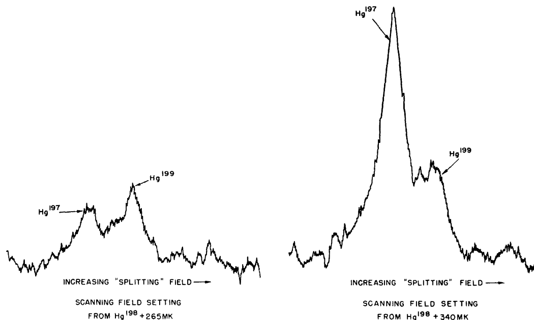
FIG. 3. The F = \frac{3}{2} , m = +\frac{1}{2} \rightarrow m = +\frac{3}{2} resonance of \text{Hg}^{197} and \text{Hg}^{199} . Scanning field set at +265 mK and at +340 mK.
