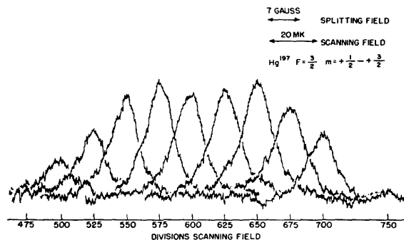
FIG. 4. Superposition of double resonance signals from the F = \frac{3}{2} , m = +\frac{1}{2} \rightarrow m = +\frac{3}{2} transition, to show the construction of the scanning curve for the F = \frac{3}{2} , m = +\frac{1}{2} sublevel.
