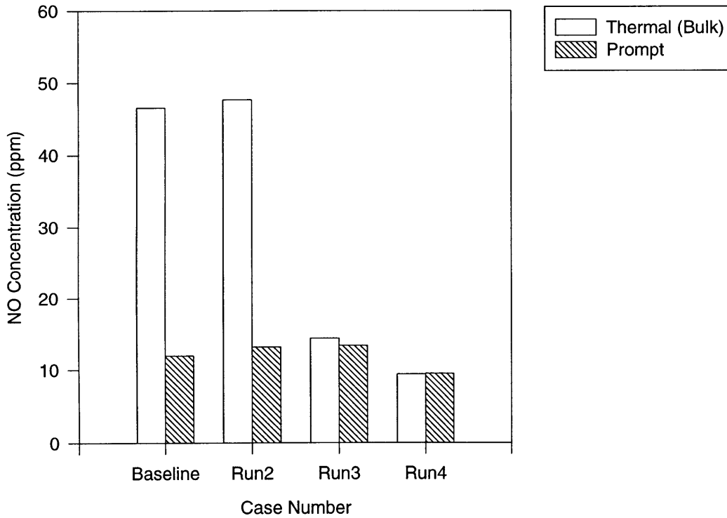
Figure 5-9: Relative Contribution of Prompt NO Mechanism
