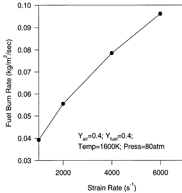
Figure 3-3: Variation of Burning Rate with Strain
