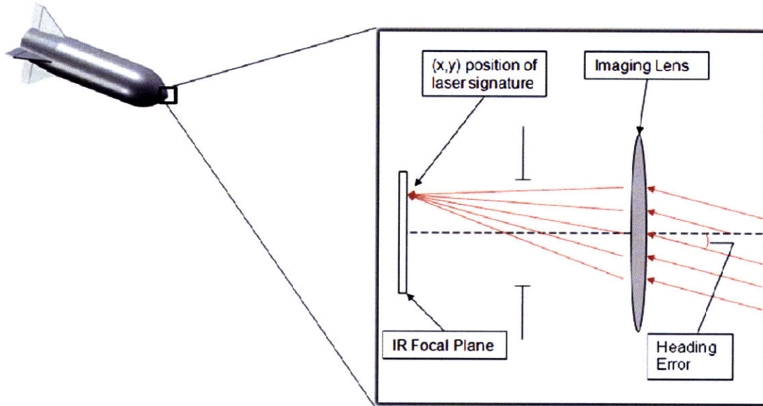
Figure 2.1.3 Expanded View of Seeker Optics
