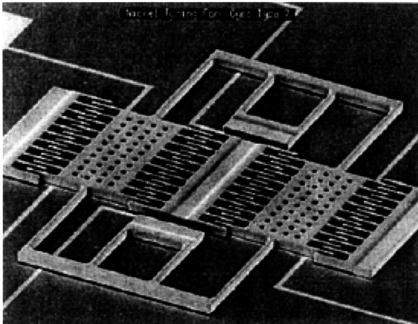
Figure 2.2.5 Draper Lab's first comb drive tuning fork gyroscope
