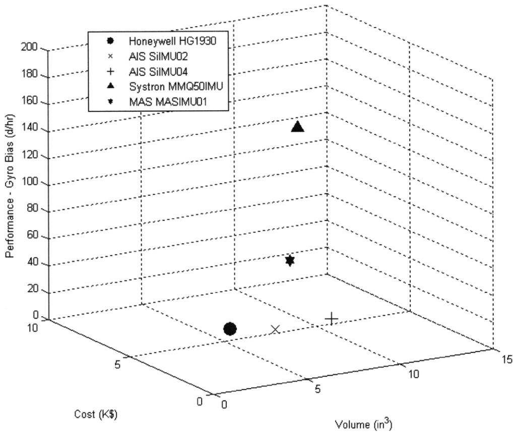
Figure 3.3.3 Final Five IMU Candidates
