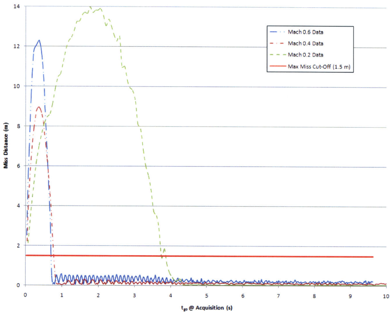
Figure 4.4.2 Estimated Miss Distances For A Given Illumination Time (15° HE assumed)
