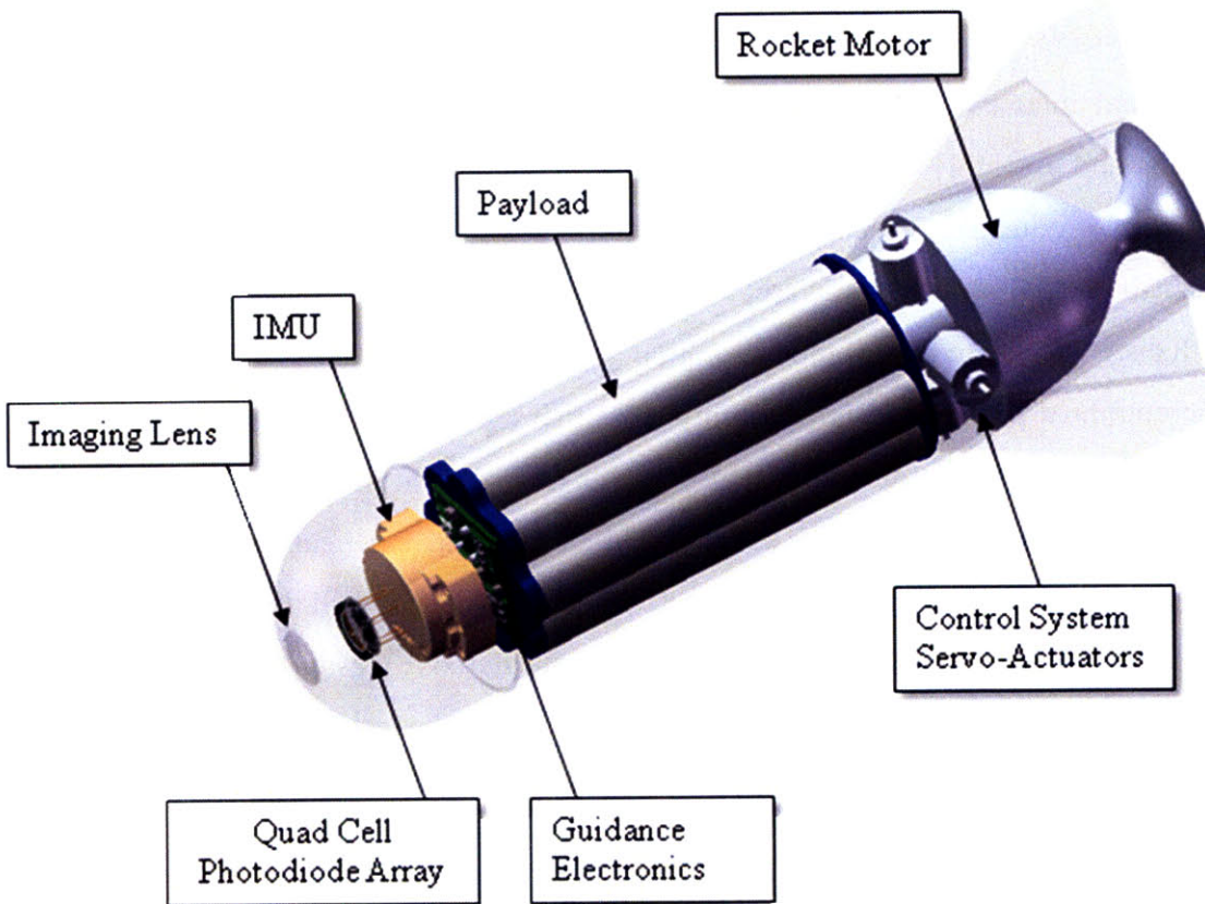
Figure 5.3.1 Proposed Seeker System Configuration - CAD Cartoon
