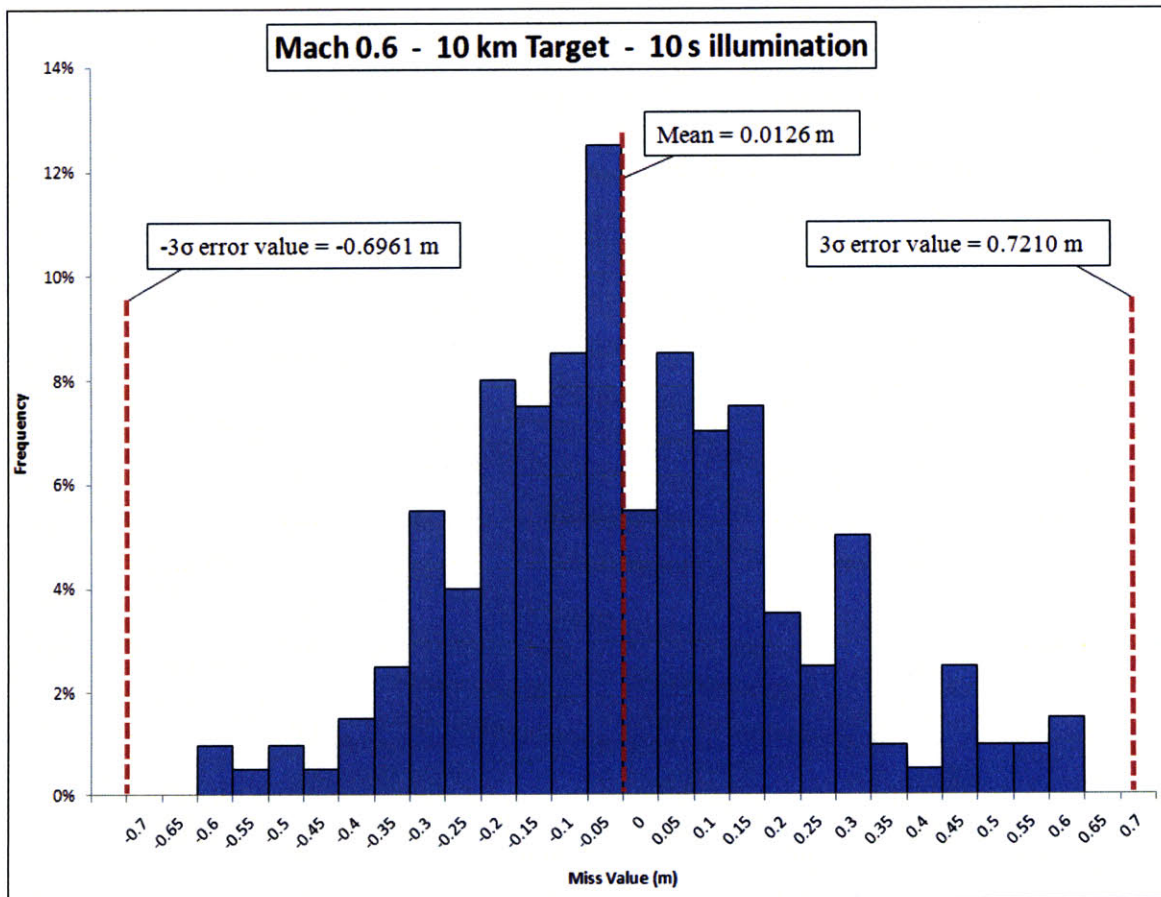
Figure 5.2.3 Histogram of Sample System Simulation Results
