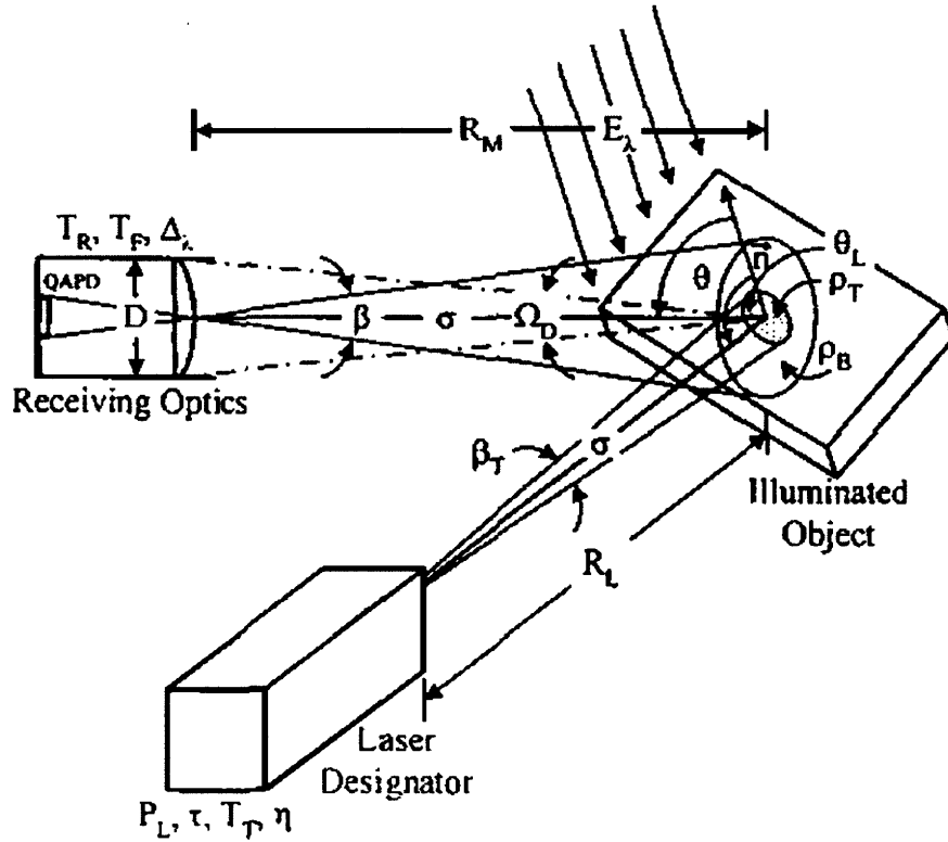
Figure 3.2.1 Simplified Laser Signal Transmission to Detector
