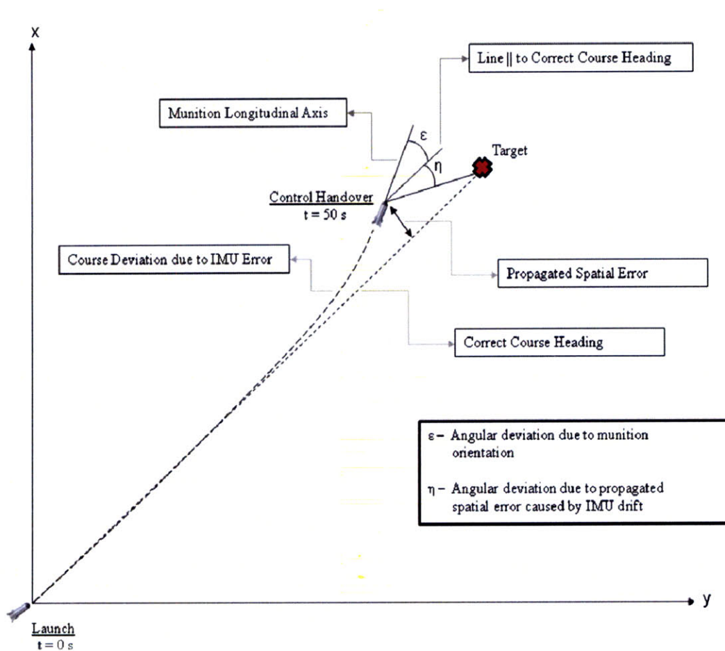
Figure 3.3.1 Allowable Drift Scenario Depiction
