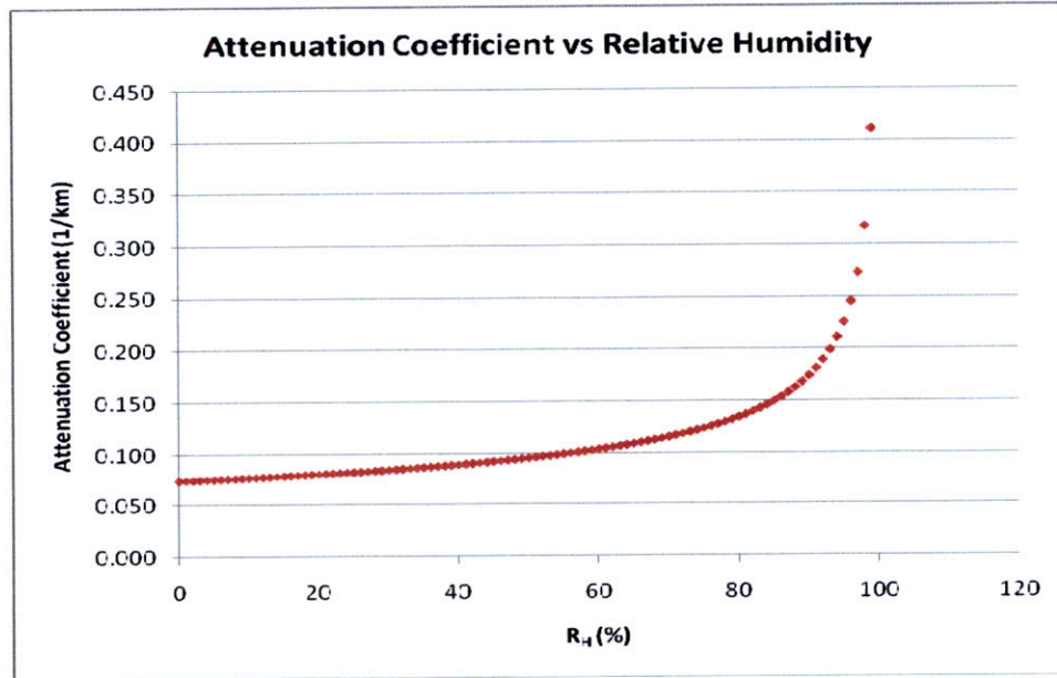
Figure 3.2.2 Relative Humidity vs Attenuation Coefficient at 1.064 \mu\text{m}
