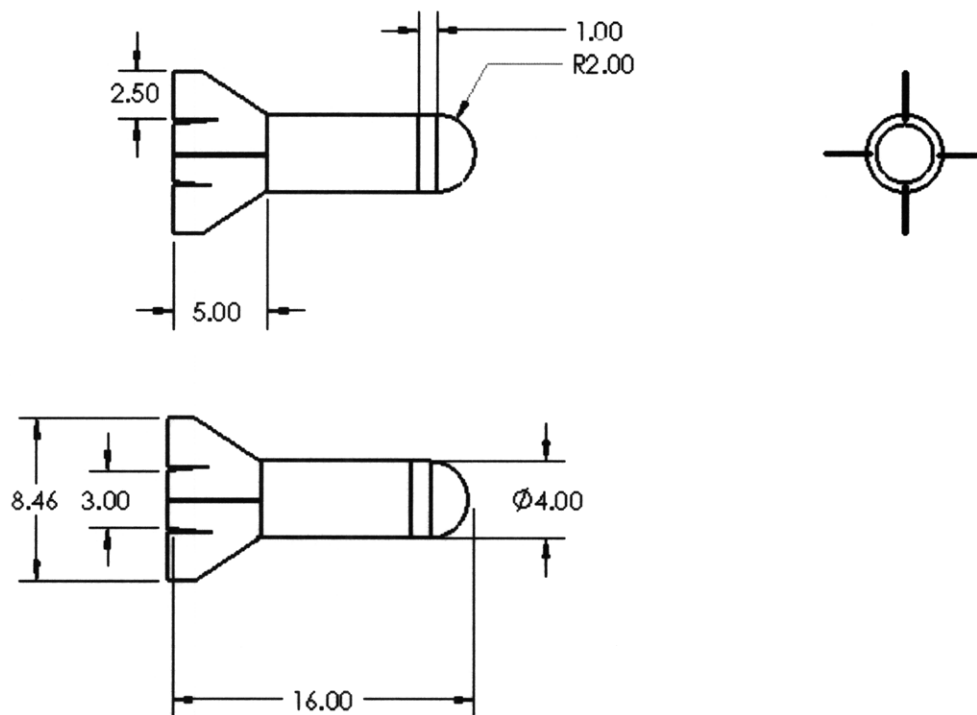
Figure 3.4.2 Standard Three View Drawing of Projectile with Dimensions (in)
