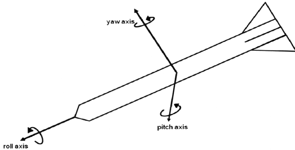
Figure 2.2.1 Body Fixed Axes for Missile Applications
