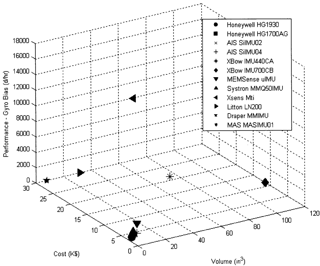
Figure 3.3.2 IMU Trade-Off Parameters Depicted in a 3-D Setting
