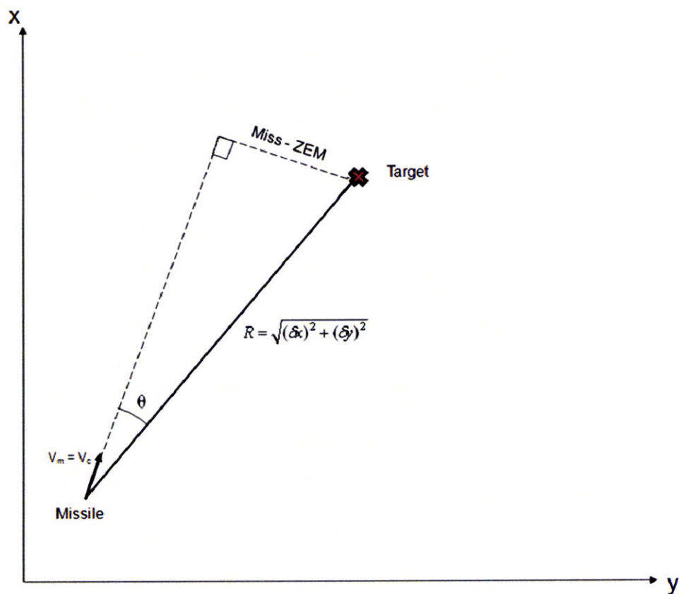
Figure 3.4.6 Miss Distance Geometry
