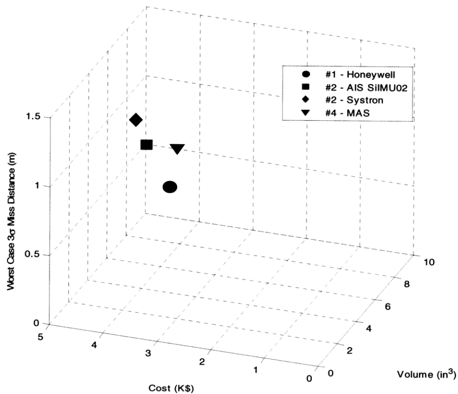
Figure 4.3.2 3-D Design Trade Plot of Candidate Seeker Systems
