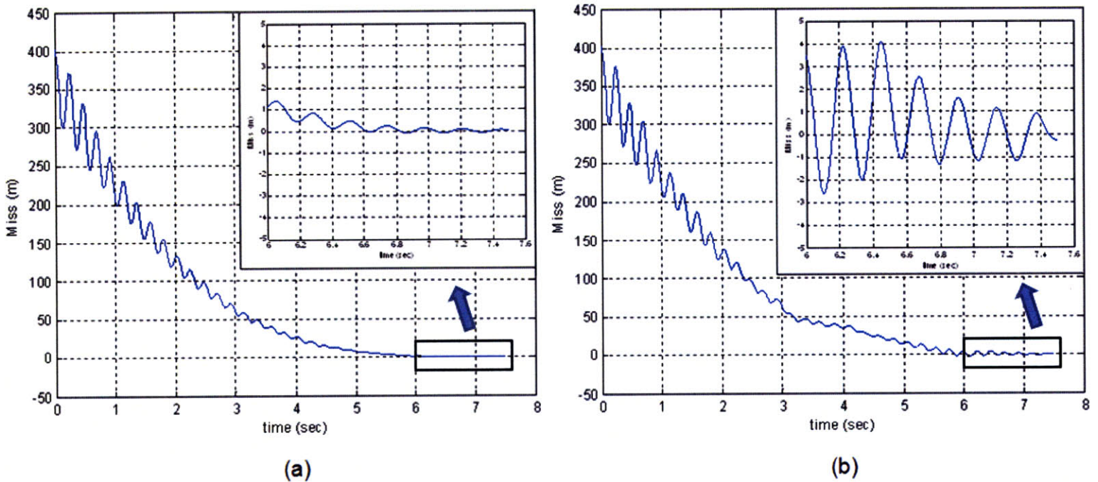
Figure 3.4.10 ZEM as a function of time (a) without LOS rate error, (b) with LOS rate error
