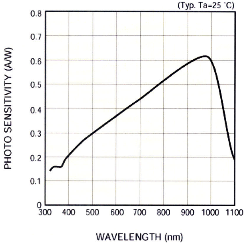
Figure 2.1.4 Photosensitivity Curve for a Hamamatsu Photodiode Array
