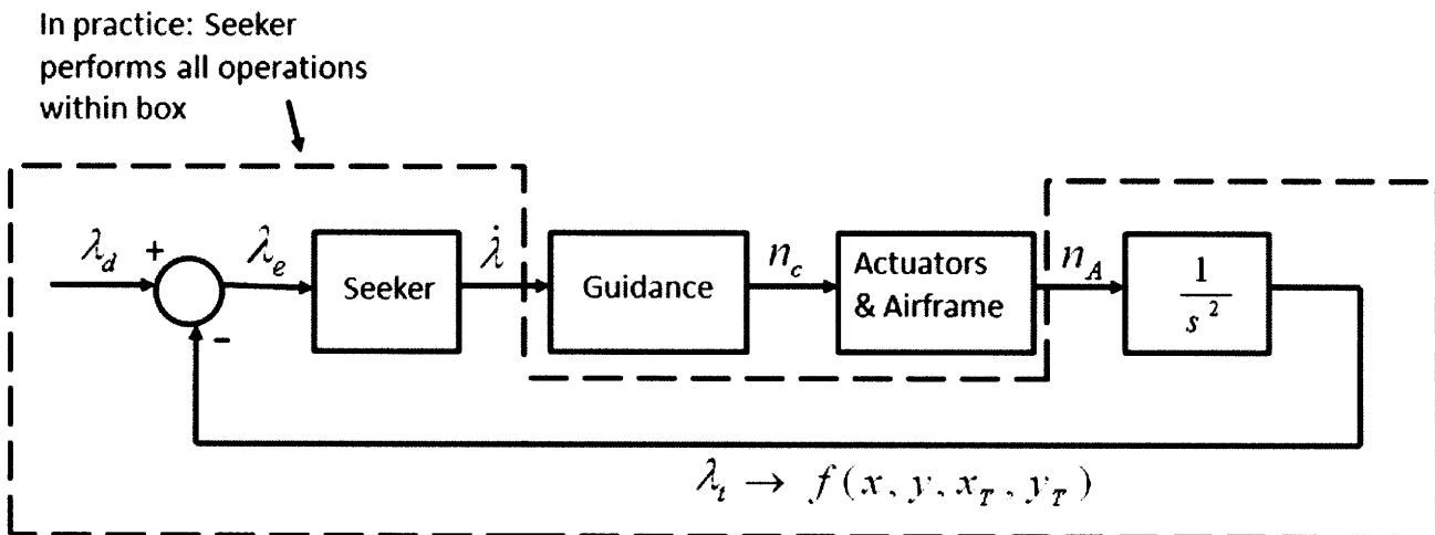
Figure 3.4.7 Simplified Proportional Navigation Guidance Loop
