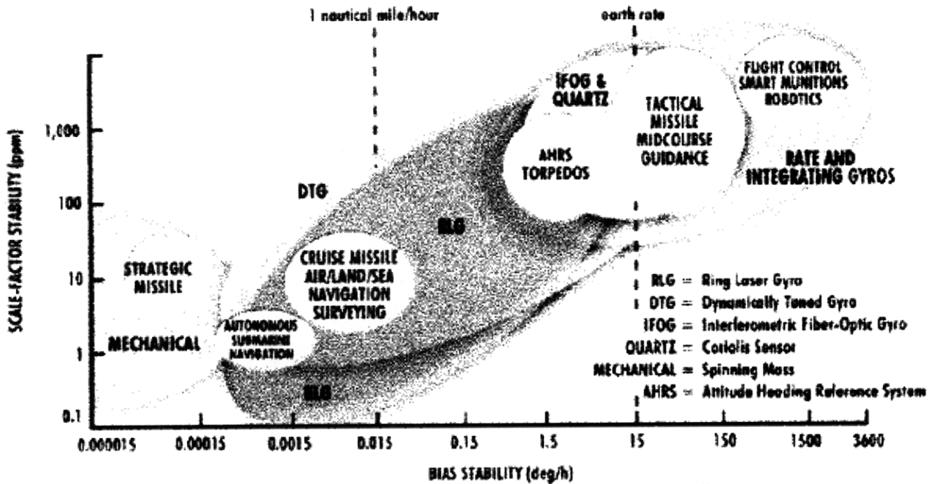
Figure 2.2.6 Gyroscope (IMU) accuracy mapped with accompanying applications
