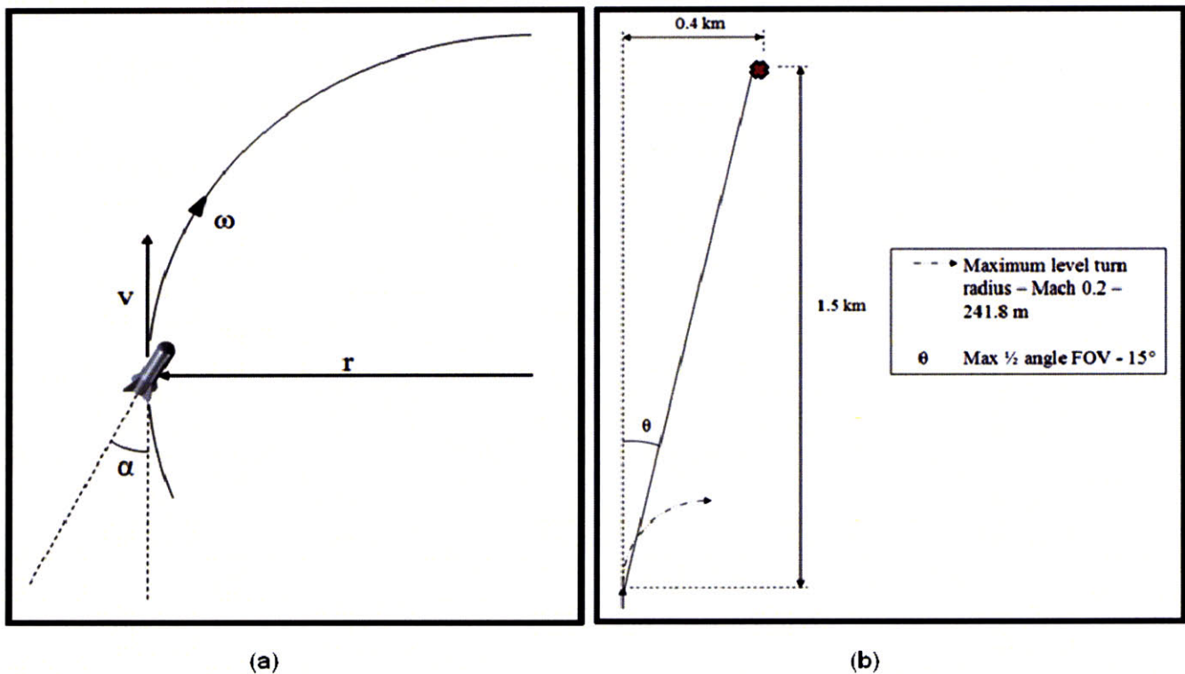
Figure 3.4.4 (a) Maneuverability Parameters, (b) Diagram Demonstrating Initial Turn Capability
