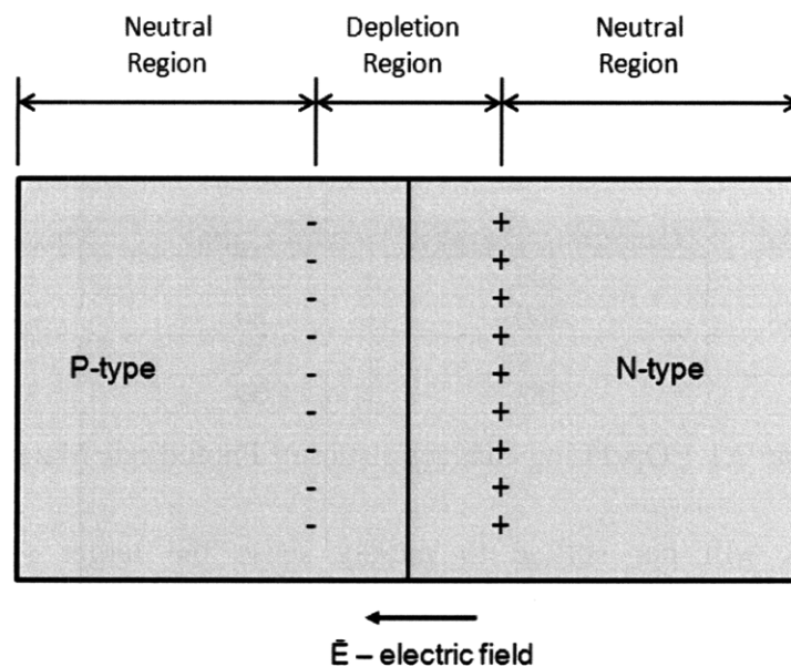
Figure 2.1.1 P-N Junction Illustration
