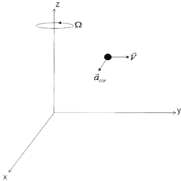
Figure 2.2.4 Apparent Coriolis Acceleration Generated in a Rotating Reference Frame
