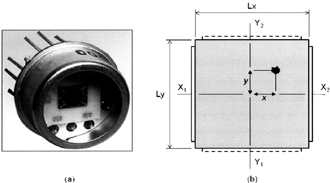
Figure 2.1.2 (a) Quadrant Detector Assembly, (b) Division of Active Area
