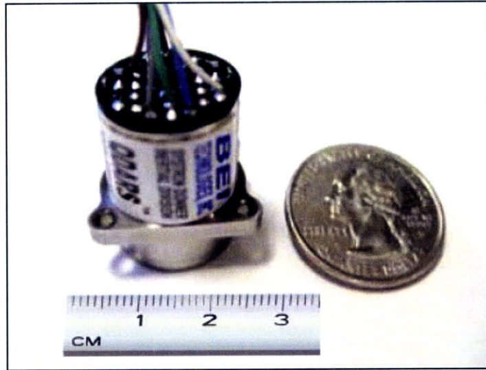
Figure 3.3.4 Systron Donner Quartz Dual Axis Rate Sensor (QDARS)
