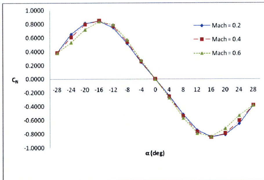
Figure 3.4.3 Pitching Moment vs Angle of Attack
