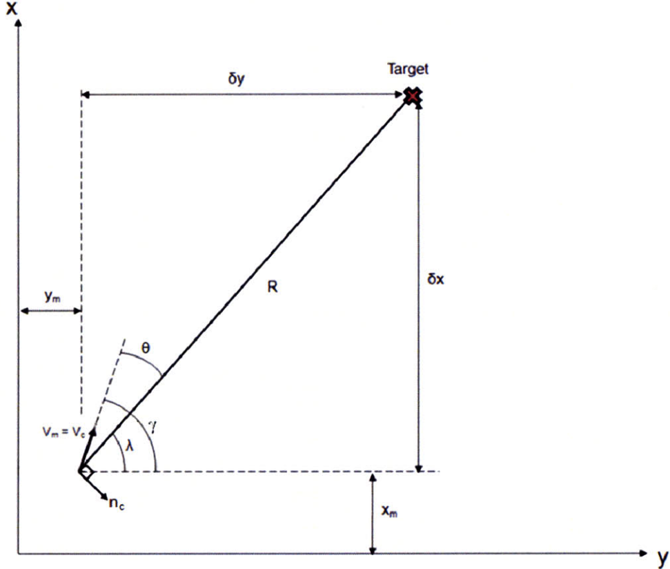
Figure 3.4.5 Two-Dimensional Simulation Geometry with Stationary Target
