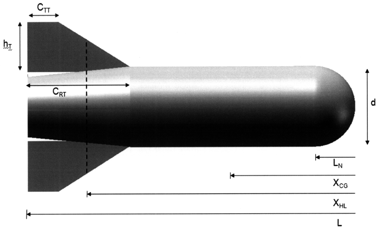
Figure E.1 Designer defined geometry and terms for airframe transfer function
