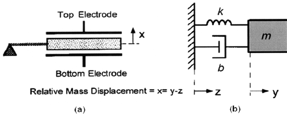
Figure 2.2.2 (a) Generic Accelerometer Structure, (b) Equivalent Mechanical Model
