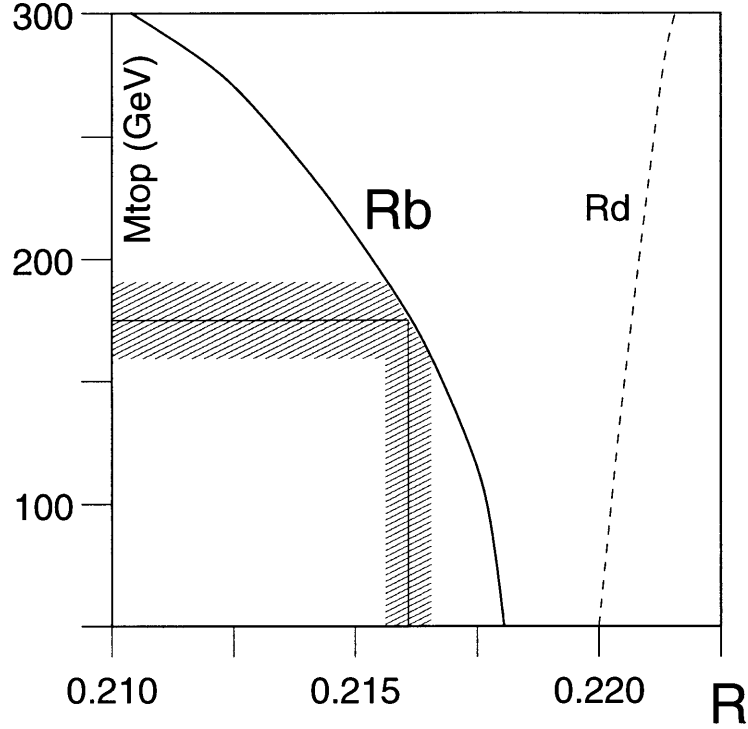
Figure 6: Standard Model predictions for the variation of R_b with the mass of the top quark. The curve is taken from the ZFITTER program [8]. The value of R_b for the first Fermilab measured value of m_{\text{top}} = 174 \pm 16 GeV [5] is highlighted. The effect on the curves of varying the Higgs mass between 60 and 1000 GeV is smaller than the resolution of the lines. The dashed line shows the equivalent curve for R_d , the corresponding ratio for d quarks.
