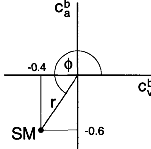
Figure 8: Coordinate system with the vector ( c_v^b ) and axial-vector ( c_a^b ) Z-b couplings as axes. Each point ( r\phi ) in the plane represents a different coupling: r is interpreted as the strength, \phi the degree of parity violation. The point shown is for the Standard Model with \sin^2 \theta_w = 0.23
