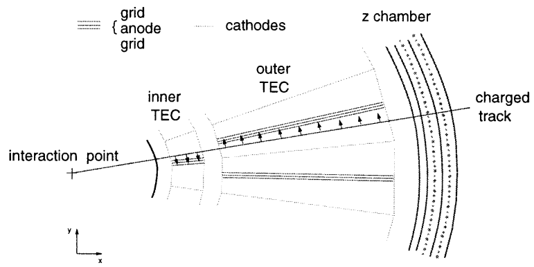
Figure 19: One inner/two outer TEC sectors, r\phi view.
