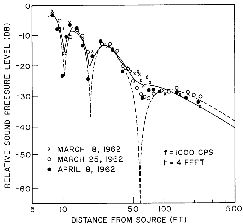
Fig. XI-2. Mean-square sound-pressure level in a turbulent atmosphere over a plane reflecting boundary as a function of distance from the source (frequency, 1000 cps). Dashed curve refers to the calculated distribution in a homogeneous atmosphere; solid curve, the calculated distribution for a turbulent atmosphere.
