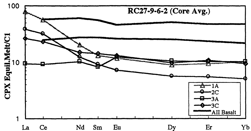
Fig. 14: Calculated equilibrium liquid compositions for diopsides from RC 27-9-6-2. Also shown for comparison is the field of basalt compositions from the Atlantis II Fracture Zone from Johnson and Dick (1992). Cpx partition coefficients are from Kelemen et al. (1993).
