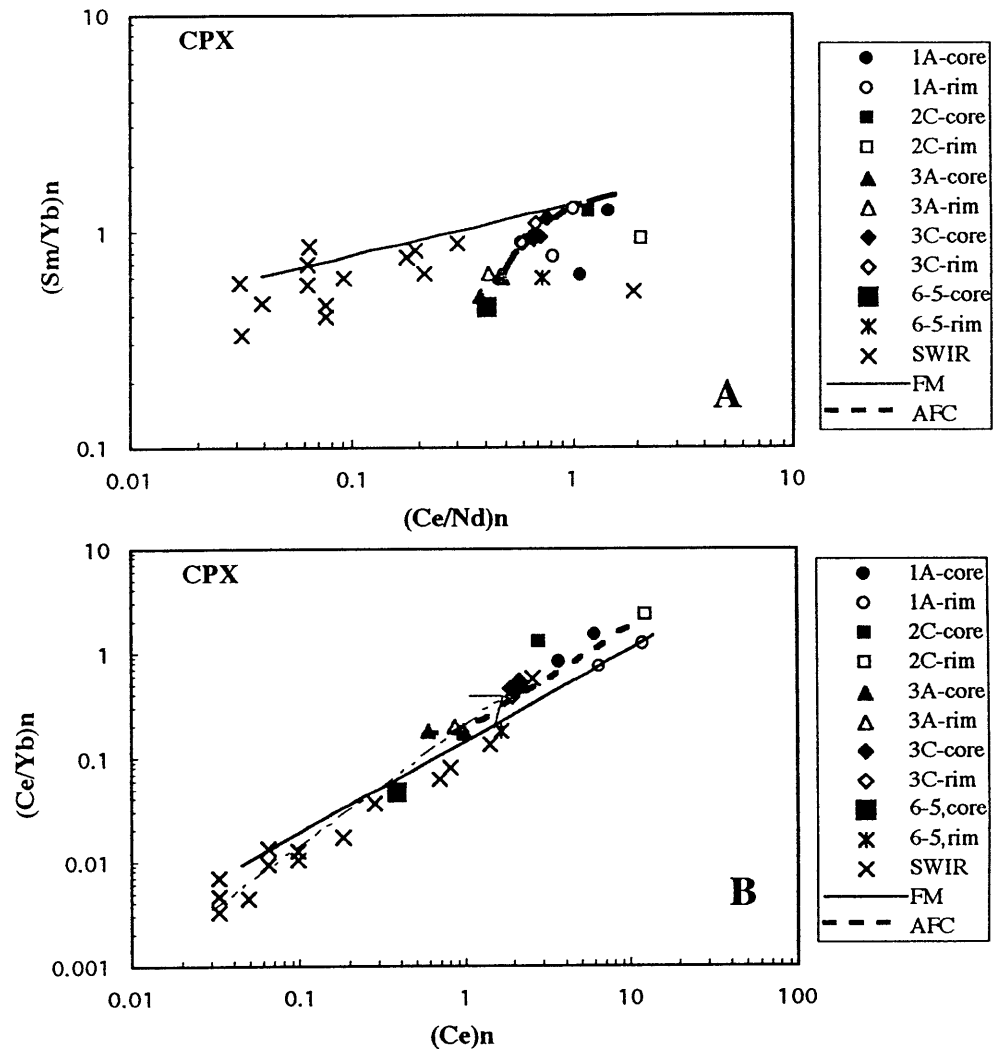
Fig.17: A. (Sm/Yb)_n vs. (Ce/Nd)_n and B. (Ce/Yb)_n vs. (Ce)_n for diopsides from RC 27-9-6-2 and RC 27-9-6-5. SWIR data, FM and AFC model trends are as in Fig.15. Also shown in dashed arrow is the refertilization model trend from Elthon (1992).
