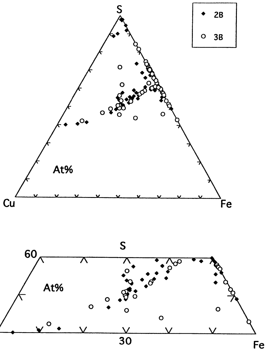
Fig.23: Sulfide compositions from thin sections 2B and 3B of RC 27-9-6-2 plotted in the S-Cu-Fe phase diagrams in atomic percent. An enlarged portion of the central region is shown at the bottom of the figure.
