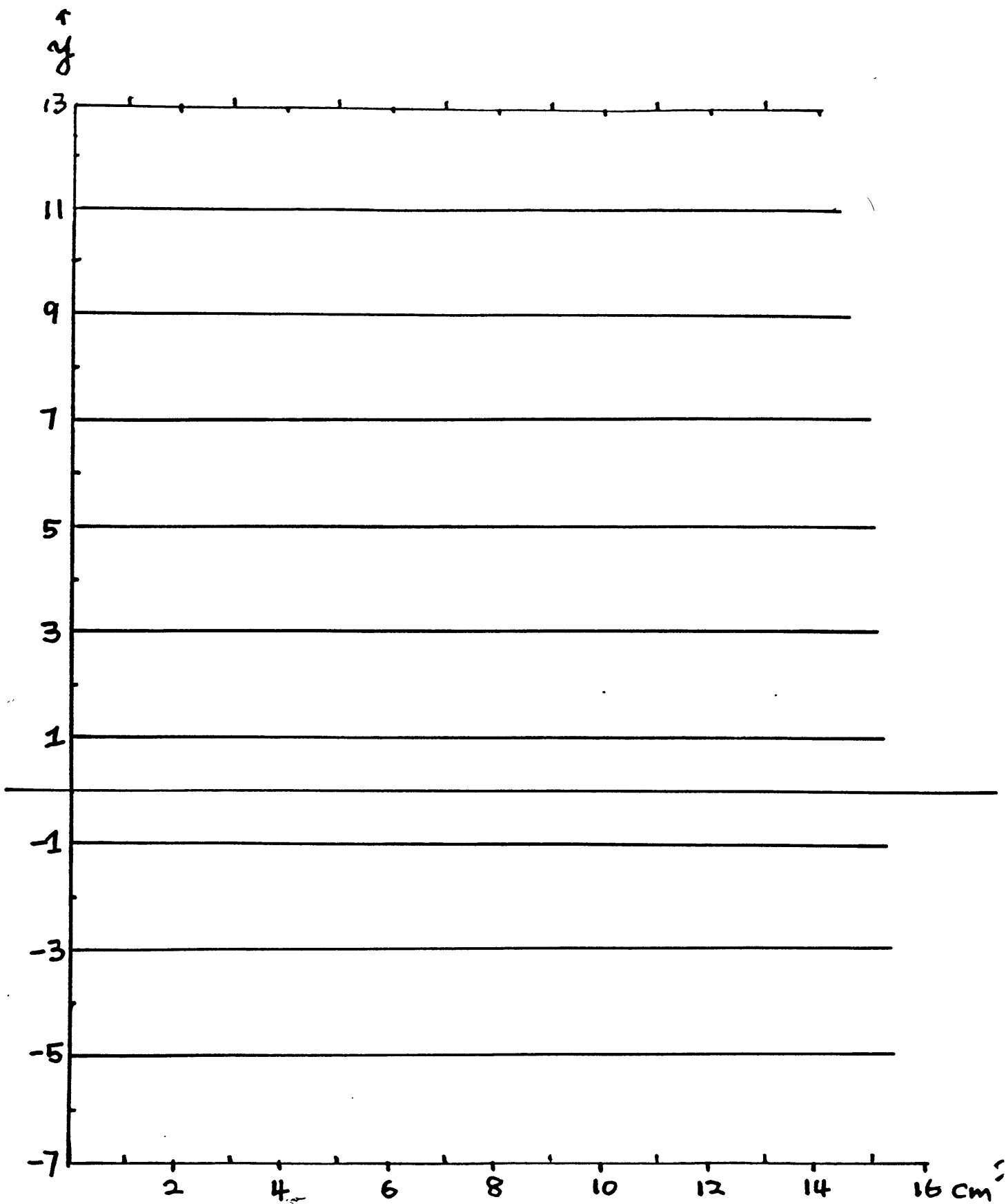
Plate 2: The reference coordinates for the sample slab relative to the clinopyroxenite vein. The coordinates are mainly based on the position of the vein in slab 2 (the thin section slab).
