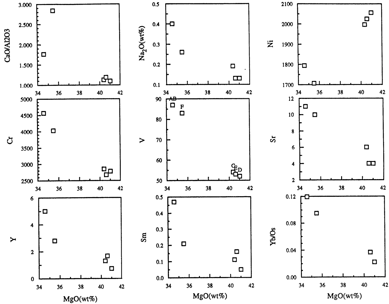
Fig.19: Major and trace element contents vs. MgO (wt%) in bulk samples from abyssal peridotite RC 27-9-6-2. Trace element concentrations are in ppm. Both the major and trace elements data are from Slab 3.
