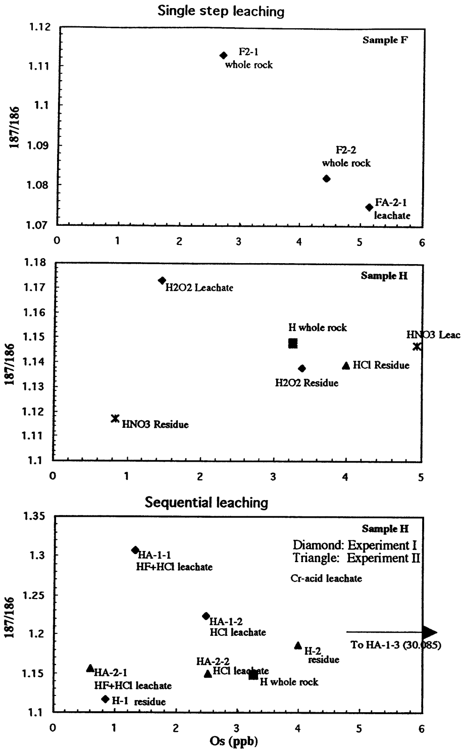
Fig.3: ^{187}\text{Os}/^{186}\text{Os} vs. Os concentration in the leached abyssal peridotite RC27-9-6-2 and its leachates. Leaching experiments were conducted on samples H and F only. For procedures for single and sequential leaching, see the 'Analytical Procedures' in text.
