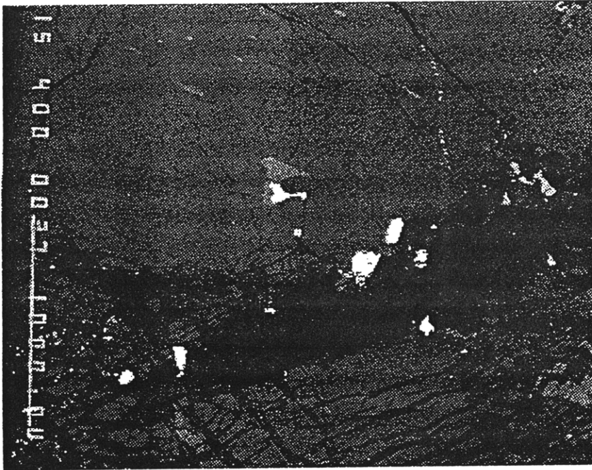
Plate 11: Type III sulfides in the serpentine vein (black area)
