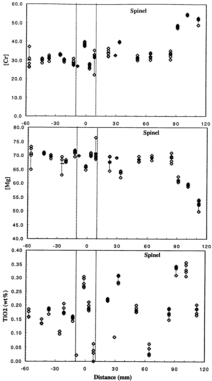
Fig.10: Compositional variation of spinel with distance for sample RC 27-9-6-2. Each separate point of analysis of a single grain is plotted and connected with a tie line. The average for each single grain is shown by the horizontal dotted line. The clinopyroxene vein is located at the center, at 0 mm. Possible regions affected by the pyroxenite vein are indicated by the dash lines.
