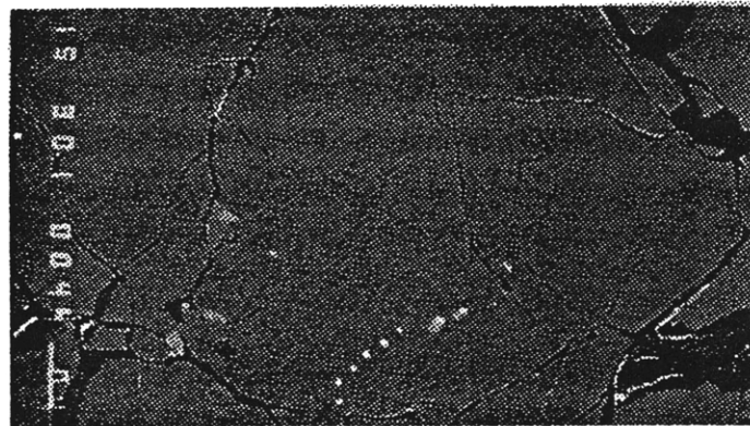
Plate 10: Type II-2 sulfides as inclusions in pyroxene grains.
