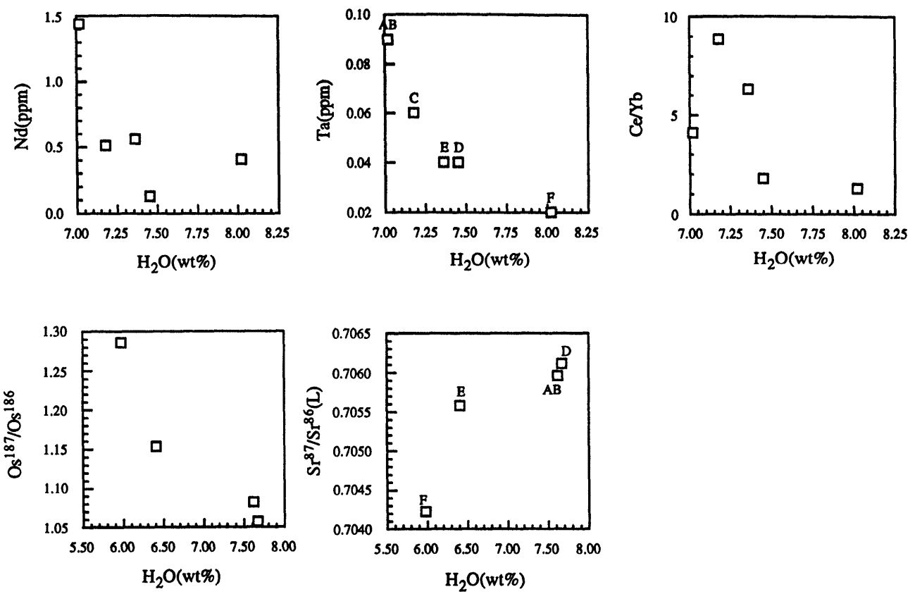
Fig.18 (Con'd) Trace element concentrations and isotopic ratios vs. water contents in bulk samples from abyssal peridotite RC 27-9-6-2. Water contents in the isotopic ratio plots are from Slab 1.
