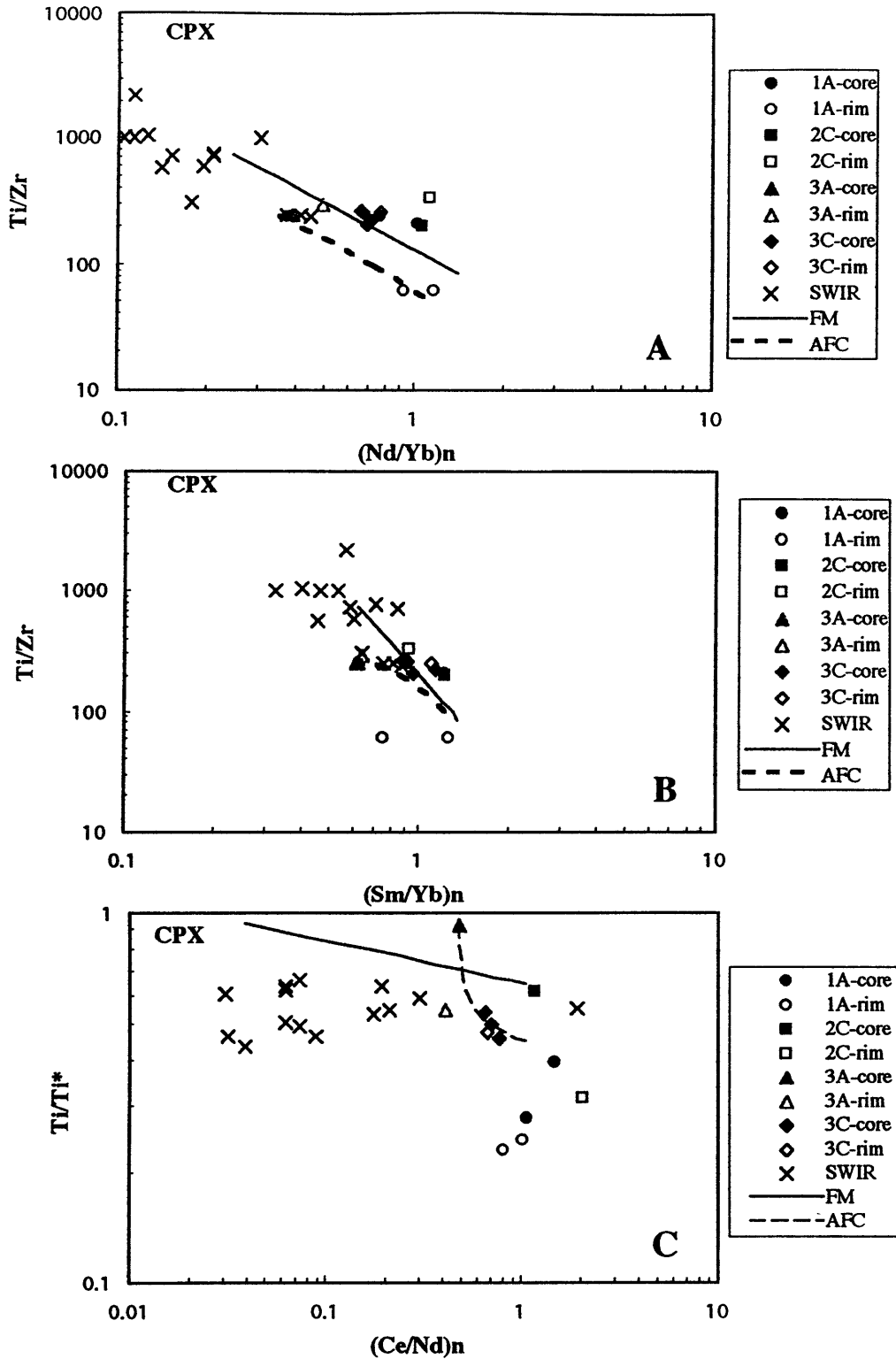
Fig.16: A. Ti/Zr vs. (Nd/Yb) n and B. (Sm/Yb) n and C. Ti/Ti* vs. (Ce/Nd) n for diopsides from RC 27-9-6-2 and RC 27-9-6-5. Also shown for comparison are data of Southwest Indian Ridge harzburgite Cpxs from Johnson et al. (1990). The solid line is a fractional melting model trend based on Johnson et al. (1990). The thick, dash line is an AFC model curve calculated using the parameters listed in Table 10.
