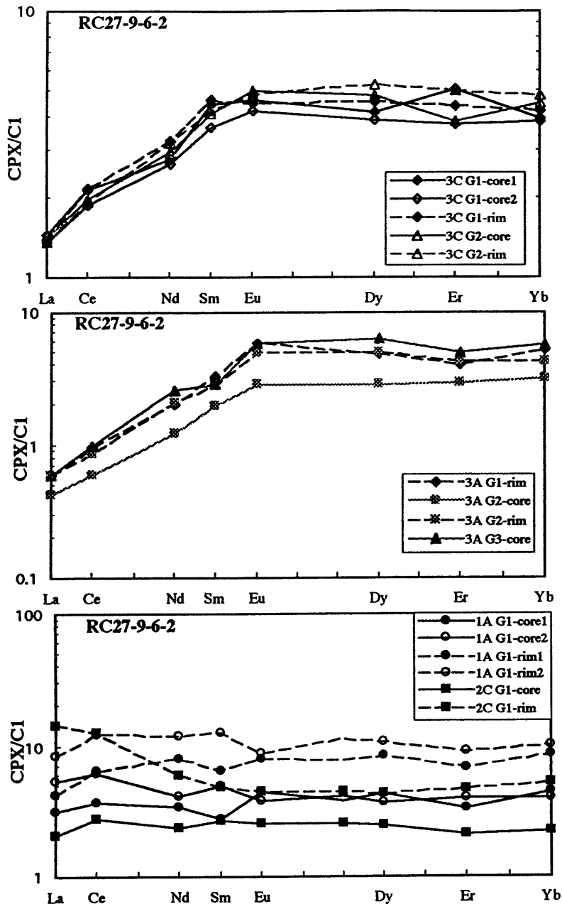
Fig. 12: REE in diopsides from RC 27-9-6-2. All REE concentrations are normalized to C1 chondrites (Anders and Grevesse, 1989).
