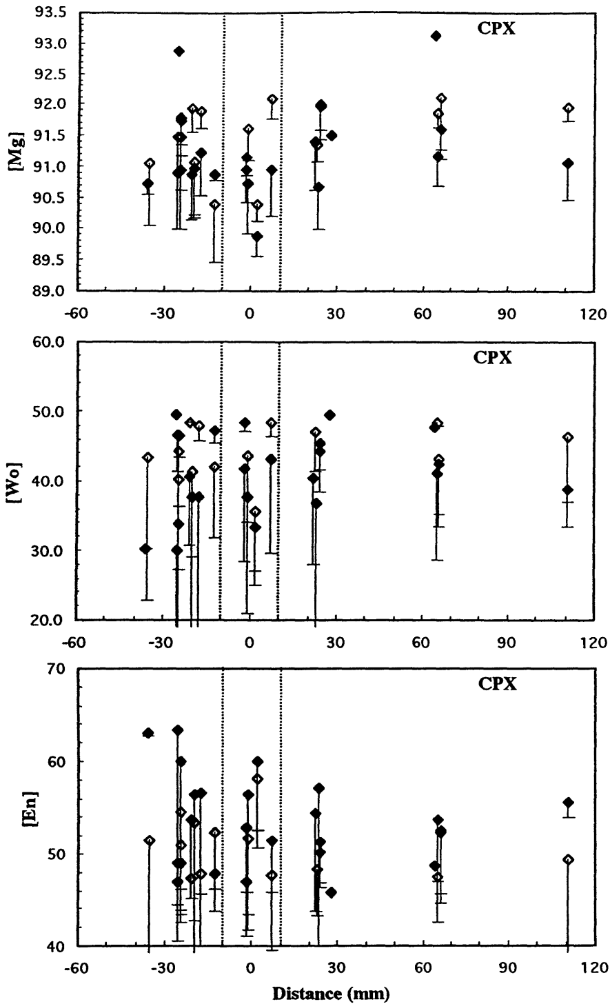
Fig.6: Compositional variation of clinopyroxenes with distance for sample RC27-9-6-2. Errors are plotted as standard deviations for averaged analyses. Core and rim data for each clinopyroxene grain are separated by solid and open symbols. The clinopyroxene vein is located at the center at 0 mm. Possible affected regions of the pyroxenite vein are indicated by the dashed lines.
