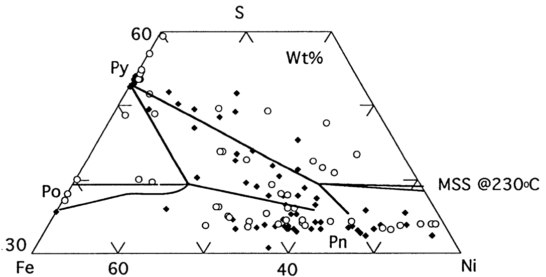
Fig.22: Sulfide compositions from thin sections 2B and 3B of RC 27-9-6-2 plotted in the S-Fe-Ni phase diagram in wt%. A blow-up of the MSS (monosulfide solid solution) field at 230°C is shown in the bottom of the figure. The 230°C S-Fe-Ni system is from Craig (1973) and Misra and Fleet (1973). Common sulfide phases are also shown for comparison. Py: pyrite; Po: pyrrhotite; Pn: pentlandite.
