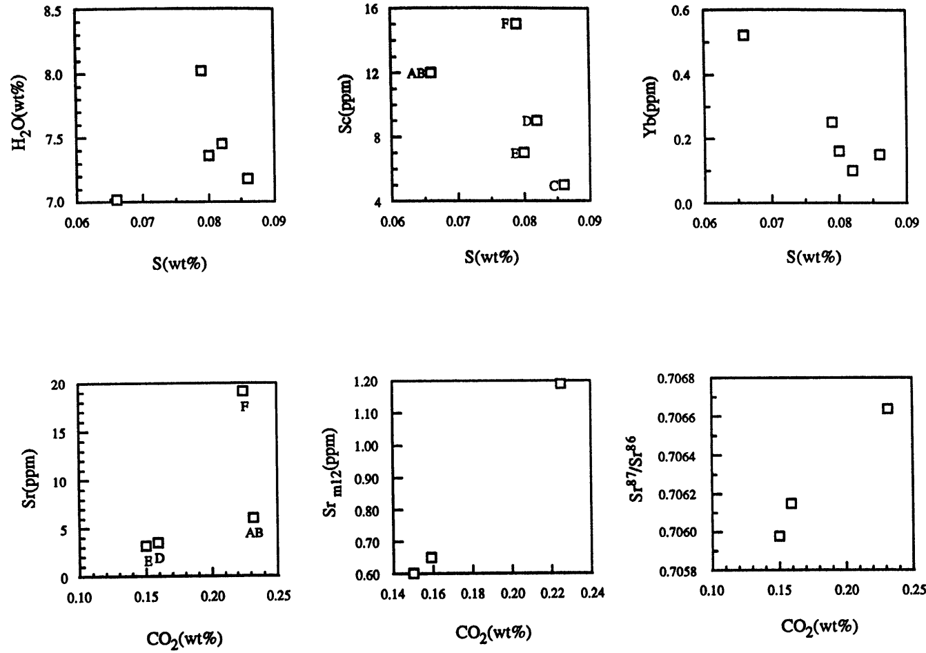
Fig 21: Elemental variation diagrams for sulfur (S, wt%) and CO 2 (wt%) contents in whole rock analyses from RC 27-9-6-2. Data in the sulfur variation diagrams are from Slab 3, while the data in the CO 2 variation diagrams are from Slab 1. Sr(m12) represents the Sr concentration in magnetic separation from 157 to 286 \mu m. Both Sr and Sr(m12) concentrations are from isotope dilution analysis.
