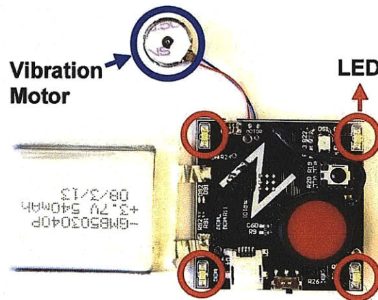
Figure 4.9 Output devices on the badge.
