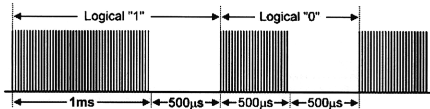
Figure 4.11 Pulse width encoding protocol for IR digital signal transmission.
