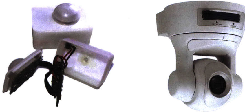
Figure 2.1 Left: a MERL motion detector node [8]. Right: the pan-tilt-zoom camera system the MERL team used to compare with the motion detection system.
