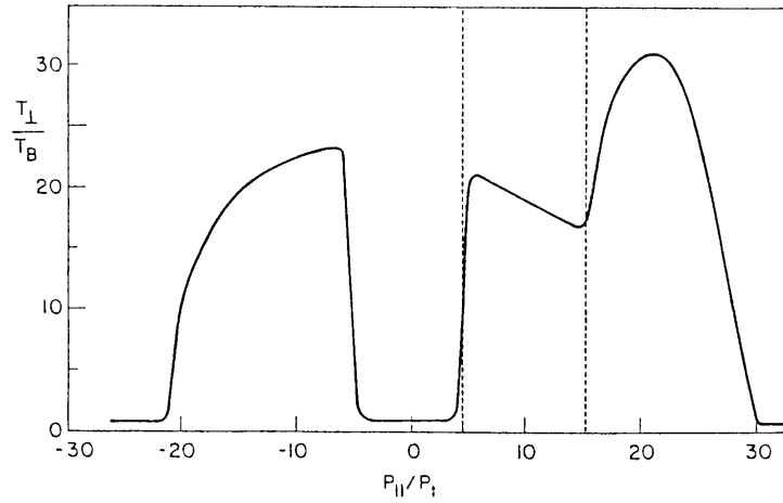
Figure 22-1: The perpendicular energy moment, normalized to the bulk temperature ( T_{\perp} / T_B ) as a function of the normalized momentum ( p_{\parallel} / P_i, p_i, v_t = m v_t ). The spectrum is located between n_{\parallel} = 1.8 and 4.5. D_o = 20 and Z_i = 1 are assumed. The interval in p_{\parallel} between the dotted lines corresponds to the resonant region.
