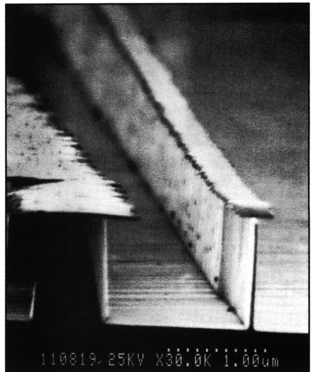
Figure 2. Nanowall ( 500\text{\AA} ) structure (on right) etched into Si<110> wafer. Note scale at bottom of figure.
