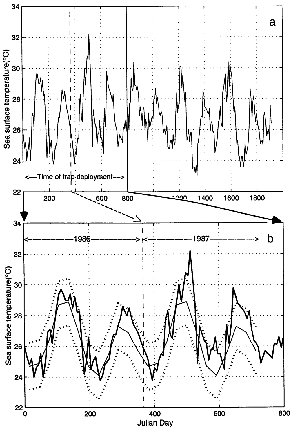
Figure 2 a) AVHRR sea surface temperatures in the western Arabian Sea beginning January 1, 1986 that show the seasonal cycles during a period of > 5 years. The steep drops in temperature (~4°C) indicate the onset of the southwest monsoon. b) Enlarged section of (a) showing the temperature record (bold line) during the time of the trap deployment. The dashed lines represent two standard deviations from the ten-year average (light line). The 1987 monsoon season has significantly warmer temperatures than the multi-year record (a) and the ten-year average.
