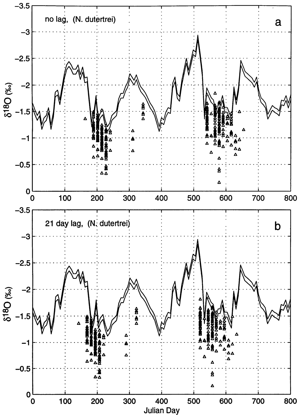
Figure 10 Time series oxygen isotopic composition for N. dutertrei plotted with a band of equilibrium calcite SST values. Data presented with a) no lag, and b) 21 day lag to account for varying settling rates. When the lag is taken into account, all the values fall within equilibrium.
