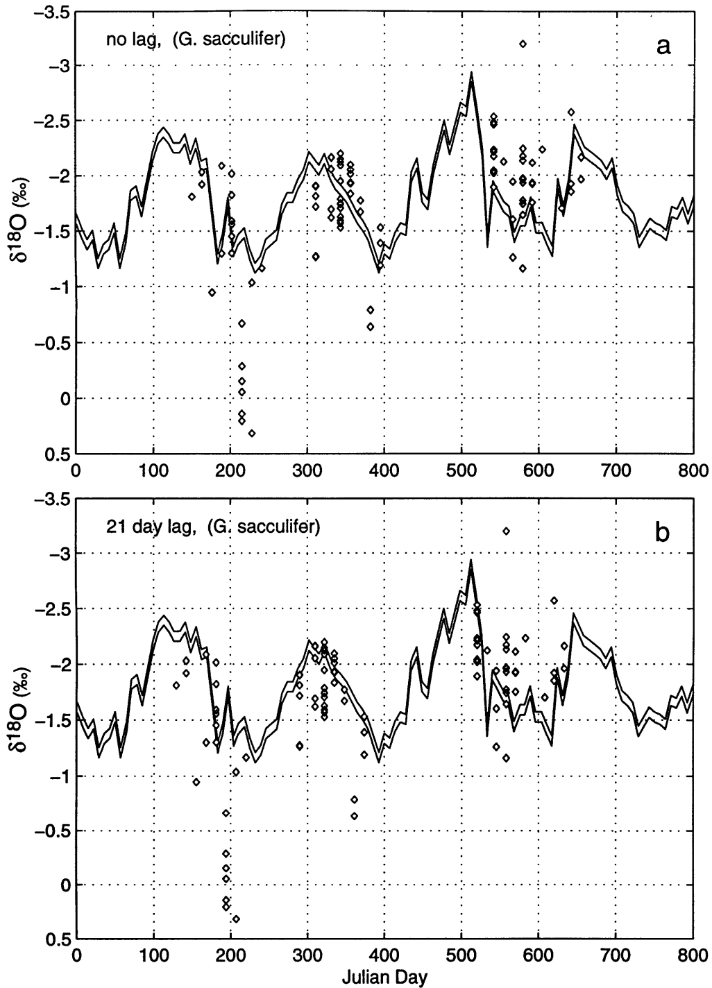
Figure 11 Time series oxygen isotopic composition for G. sacculifer plotted with a band of equilibrium calcite SST values. Data presented with a) no lag, and b) 21 day lag to account for varying settling rates. Even when a lag is applied, almost half of the values remain out of equilibrium, especially the individuals from the 1987 southwest monsoon.
