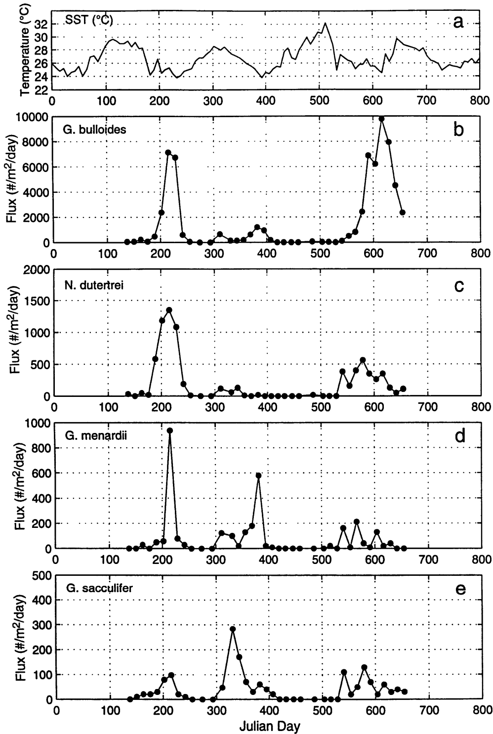
Figure 6 Flux ( \#/m^2/day ) time series for all four species, showing increased production during both monsoon periods, especially the southwest monsoon (around Julian Days 200 and 570). The a) AVHRR sea surface temperature, b) G. bulloides , the most abundant species used as an upwelling indicator, c) N. dutertrei , d) G. menardii , e) G. sacculifer . Note the different vertical scales.
