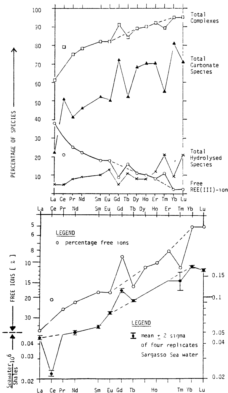
Figure 6.3. ABOVE: Percentages of various species of REE(III) in seawater as predicted by the model of TURNER, WHITFIELD & DICKSON (1931). Note the strong Gd excursions.
