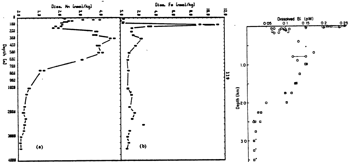
Vertical profile of dissolved bismuth at North Pacific Ocean (17° 30' N, 109° 00' W; water depth, 3550 m) on Nov 1981: O, collected by J. Martin; □, collected by K. W. Bruland.
