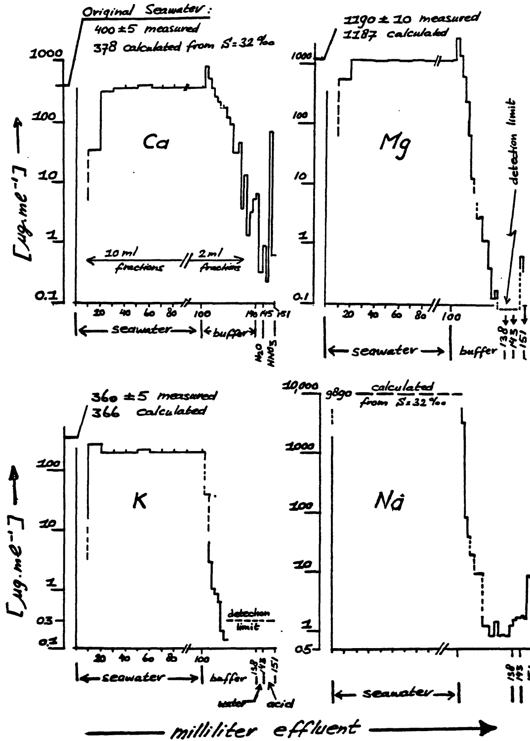
Figure 2.6.5 CHELEX-100 chromatography of Na, K, Mg and Ca along with the ^{54}\text{Mn} radiotracer experiment. Note dropoff during washing stages and distinct peak for all elements in nitric acid fraction.
