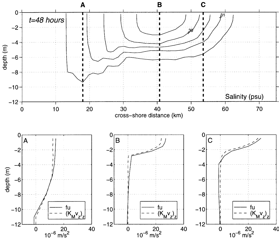
Figure 4.6: Profiles of Coriolis and stress divergence terms of the alongshore momentum balance (Ekman terms) at t=48 hours for the shoreward front (A), plume core (B), and seaward front (C). Other terms are significantly smaller (see text for discussion and Figure 4.7 for more details). K_M is the turbulent diffusivity of momentum.
