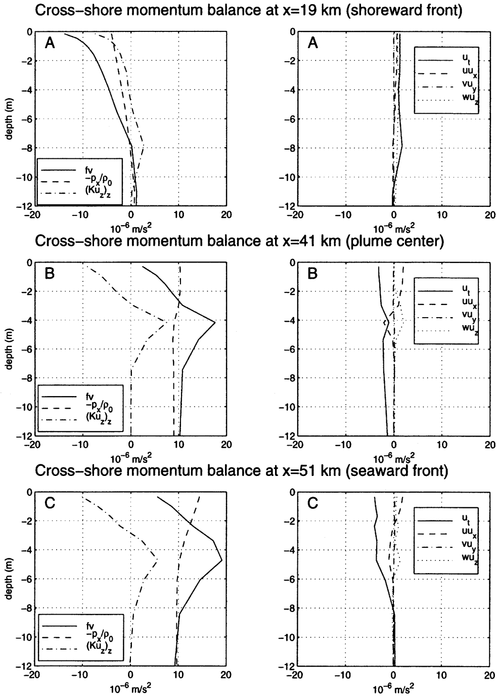
Figure 4.8: Cross-shore momentum balance at the shoreward front (A), plume center (B), and seaward front (C) at t=48 hours (for locations of profiles A, B, and C, see Figure 4.6). The horizontal diffusion terms (not shown) are approximately an order of magnitude smaller than the advective terms.
