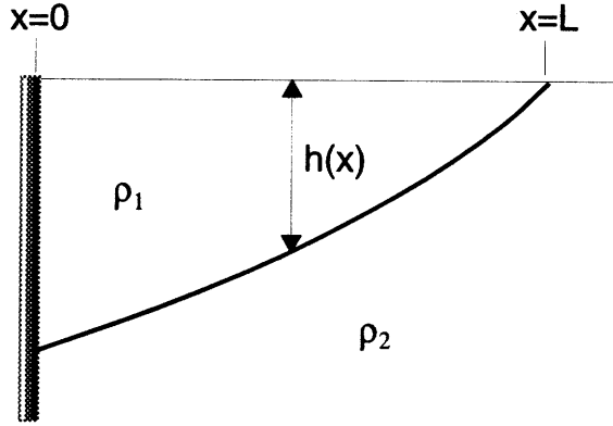
Figure 2.8: Idealized Margules front representation of the coastal current.
