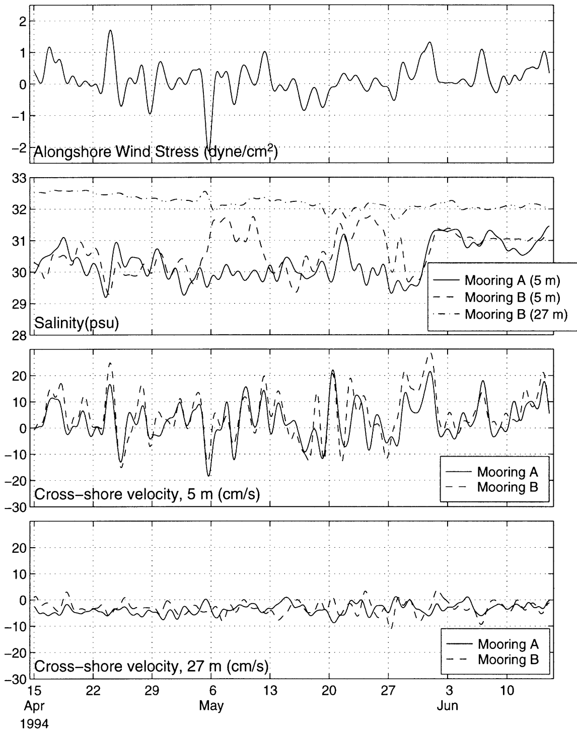
Figure 3.5: Time series of alongshore wind stress, salinity and cross-shore velocities measured at Cape Porpoise in 1994.
