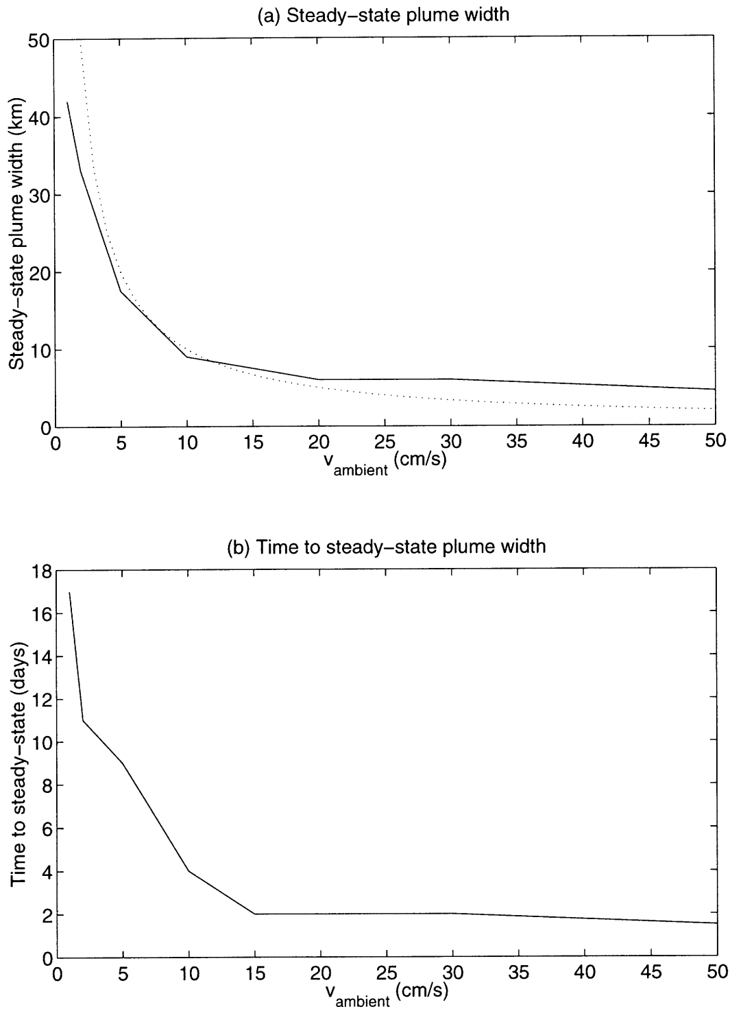
Figure 2.18: Steady state plume width for Base model run with a range of v_{amb} . (a) Steady state plume width (the dotted line indicates a 1/v_{amb} dependence), and (b) Time to reach steady-state plume width as a function of ambient flow strength.
