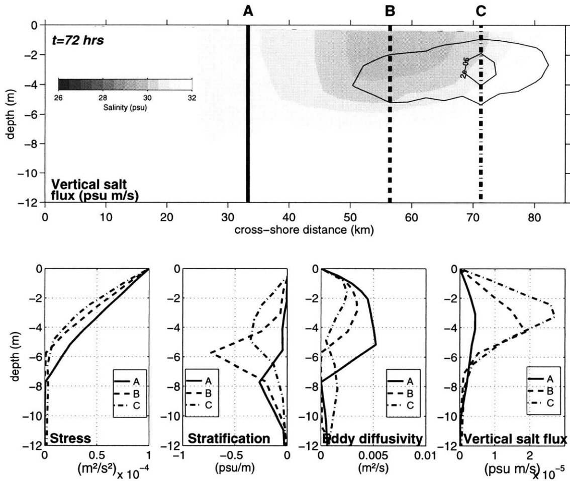
Figure 4.11: Contours of salinity (gray shades) and vertical salt flux are shown in the upper panel at t=72 hours. Profiles of stress, stratification, eddy diffusivities of salt, and vertical salt flux are plotted in the lower panels for the shoreward front (A), plume core (B), and seaward front (C).
