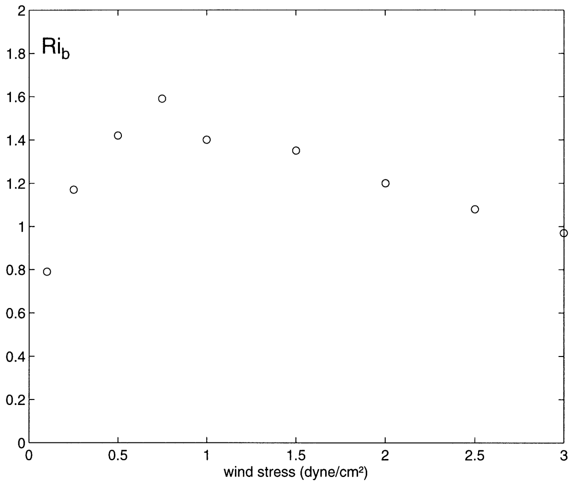
Figure 4.15: Mean bulk Richardson number as a function of wind stress (Runs 1-9).
