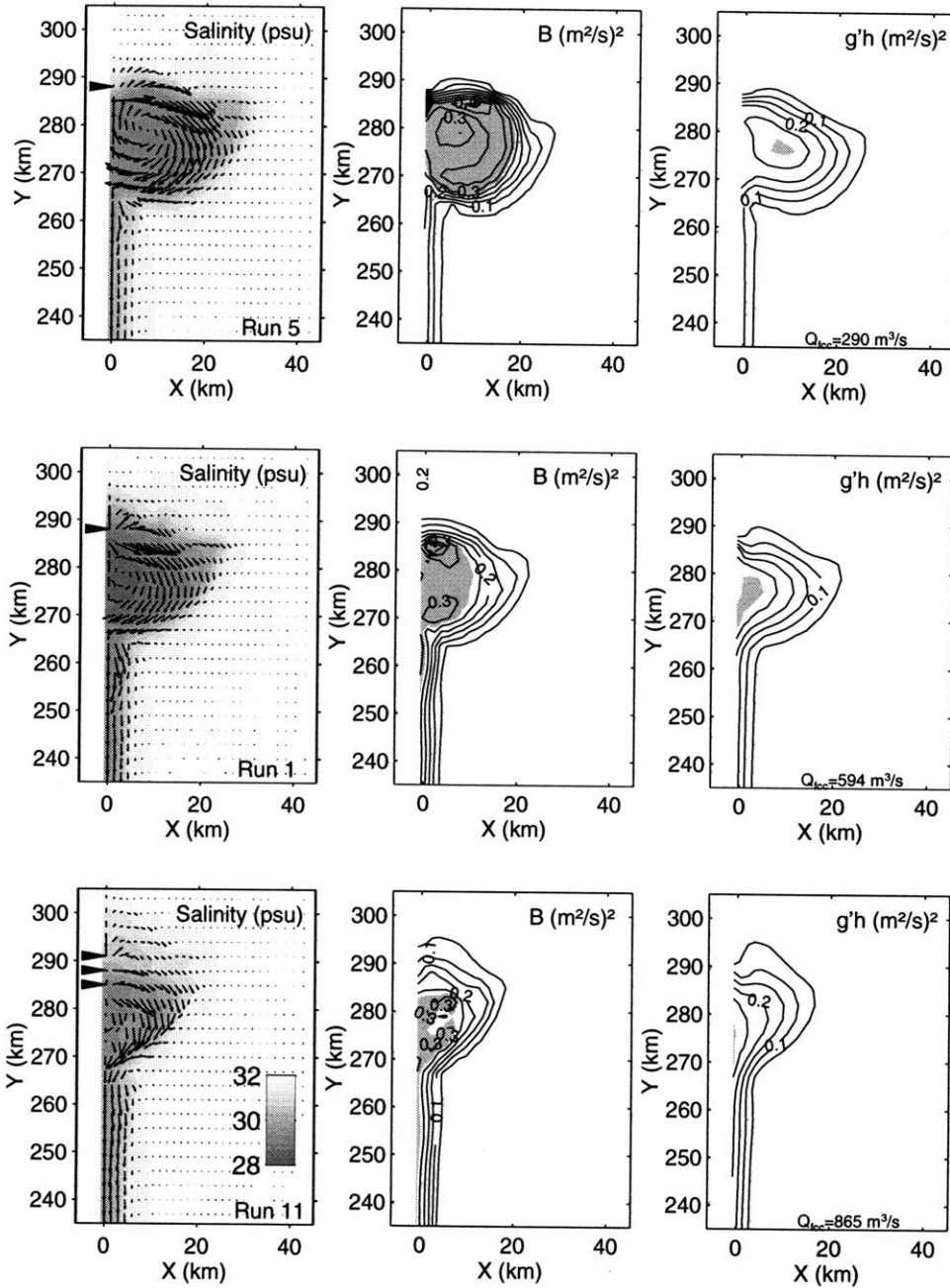
Figure 2.10: Bulge behavior for different Froude number conditions. The surface salinity and velocity; Bernoulli function B ; and potential energy g'h are plotted for Runs 5, 1, and 11. Shaded regions in the panels plotting B and g'h indicate regions of B and g'h > 0.279 \text{ m}^2/\text{s}^2 . Contours of B and g'h are in intervals of 0.05 \text{ m}^2/\text{s}^2 . The coastal current transport at y=252 \text{ km} is shown in the lower-right of the g'h contours.
