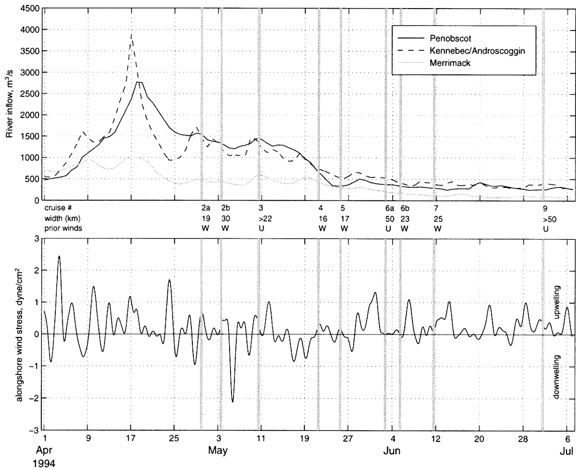
Figure 3.3: 1994 observations in the western Gulf of Maine (as in Figure 3.2).
