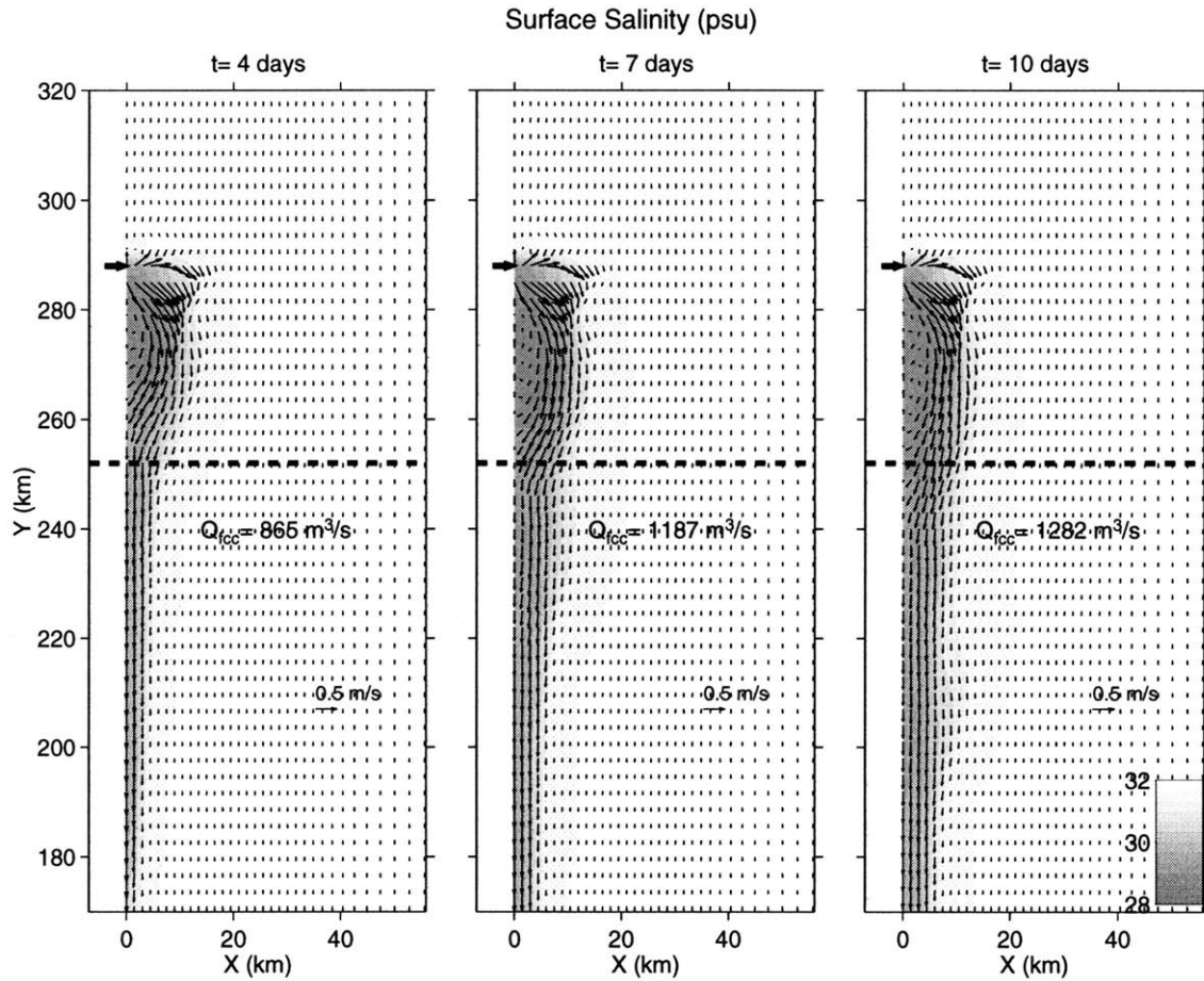
Figure 2.16: Surface salinity (psu) indicated by gray shading for Base Case model run (Run 1) with an ambient current of 10 cm/s ( t = 4, 7, 10 days). Velocity vectors are superimposed to indicate the flow field. Freshwater transport is measured at y = 252 km (indicated by dashed line). River mouth location is indicated by bold arrow.
