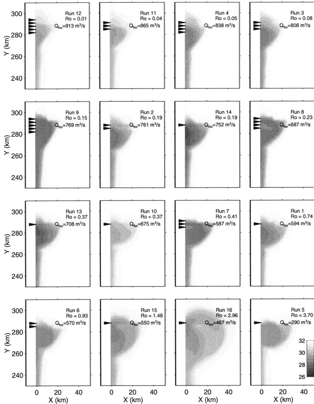
Figure 2.12: Surface salinity at t=5 days for different Rossby number conditions are shown in gray. The location of the river mouth (and river mouth widths) are indicated by the arrows. The width of the river mouth is the number of arrows times 3 km (e.g., the River mouth is 15 km wide for Run 12) The Rossby number and the freshwater transport in the coastal current (at y=252 km for Runs 1-14 and y=232 km for Runs 15 and 16) is shown in each panel.
