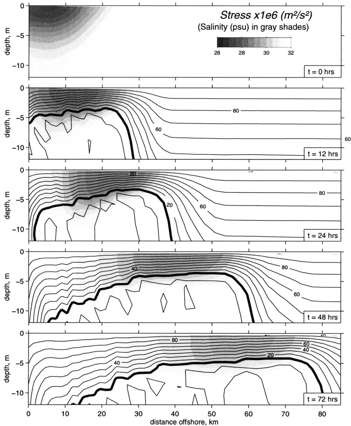
Figure 4.5: Contours of stress and salinity for t = 0, 12, 24, 48, and 72 hours. Gray contours are used to indicate salinity contours in intervals of 0.5 psu. Superimposed on the gray shading are contours of magnitude of the total stress in solid contour lines ( 0.1 dyne/cm 2 intervals). The thick contour line is stress which is 10\% of the applied surface stress.
