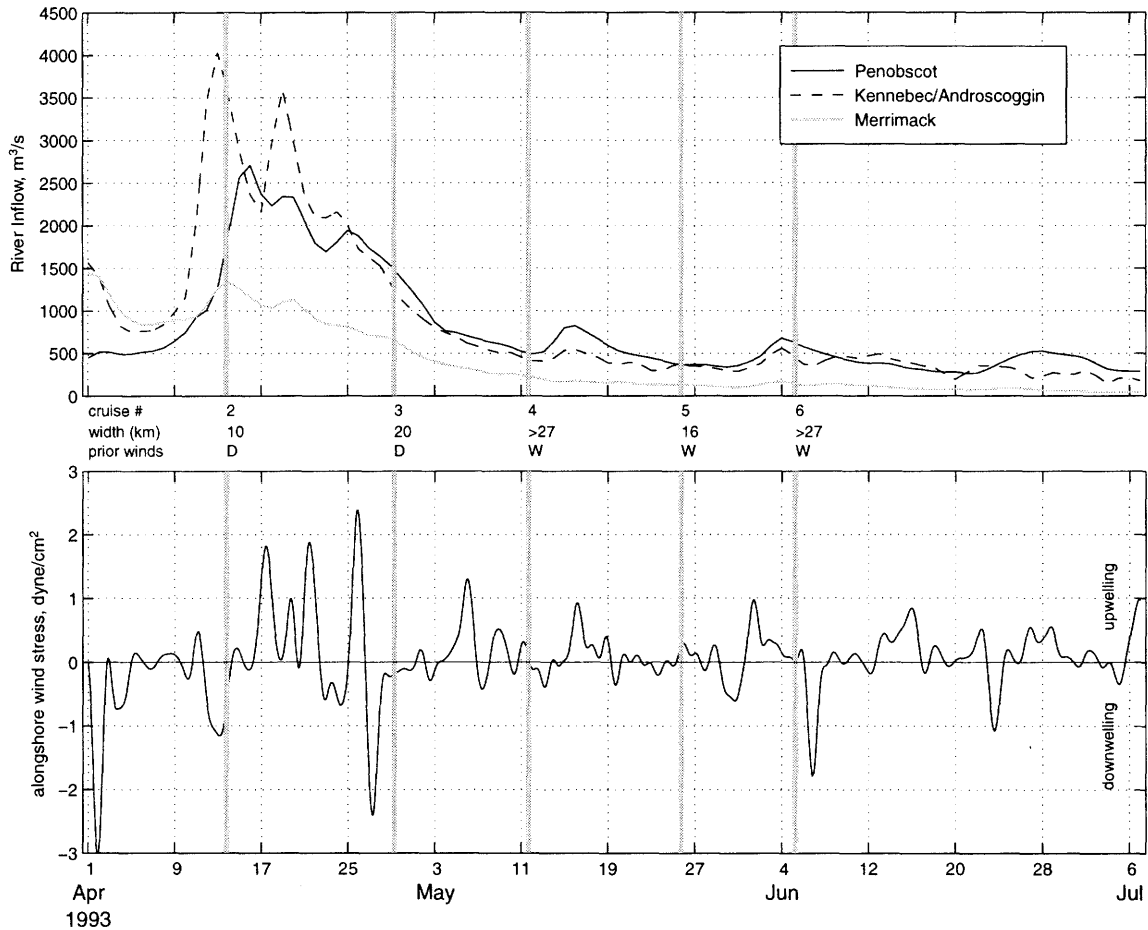
Figure 3.2: 1993 observations in the western Gulf of Maine. Time series of winds measured at the meteorological buoy and freshwater inflow from the Penobscot, Kennebec/Androscoggin, and Merrimack river systems are shown. The timing of hydrographic surveys at the Cape Porpoise transect are indicated by the gray vertical bands. The observed plume width during the surveys are indicated in km with a classification of the winds preceding each survey; D indicates downwelling favorable winds prior to the survey while upwelling favorable winds are labeled with a U; weak winds are denoted by a W.
