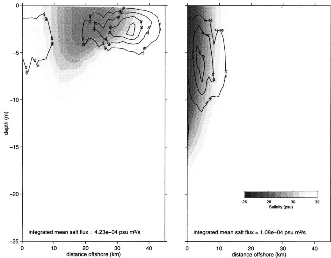
Figure 4.19: Comparison of mixing during upwelling and downwelling. Salinity (in gray shades) and vertical salt flux (lines) are contoured for 1 \text{ dyne/cm}^2 upwelling favorable (left panel) and downwelling favorable (right panel) alongshore wind stress after 24 hours of forcing. The cross-shore integrated mean vertical salt flux is indicated in the lower left corner of each panel.
