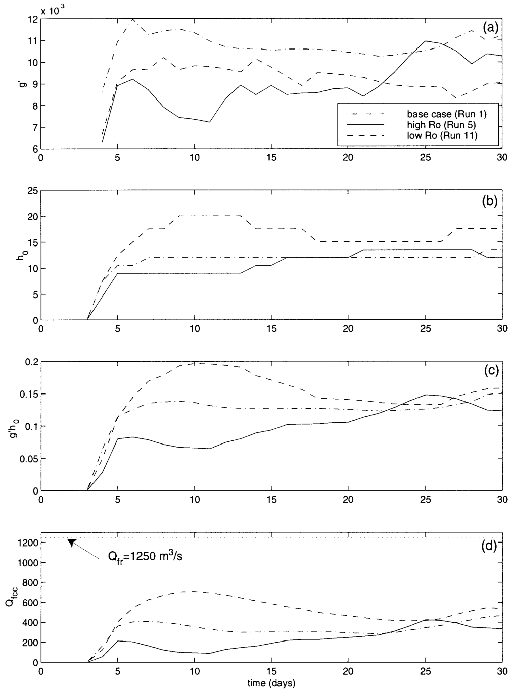
Figure 2.14: Temporal variations in the coastal current at y=230 km. (a) g' , (b) h_0 (c) g'h_0 (d) Q_{fcc} .
