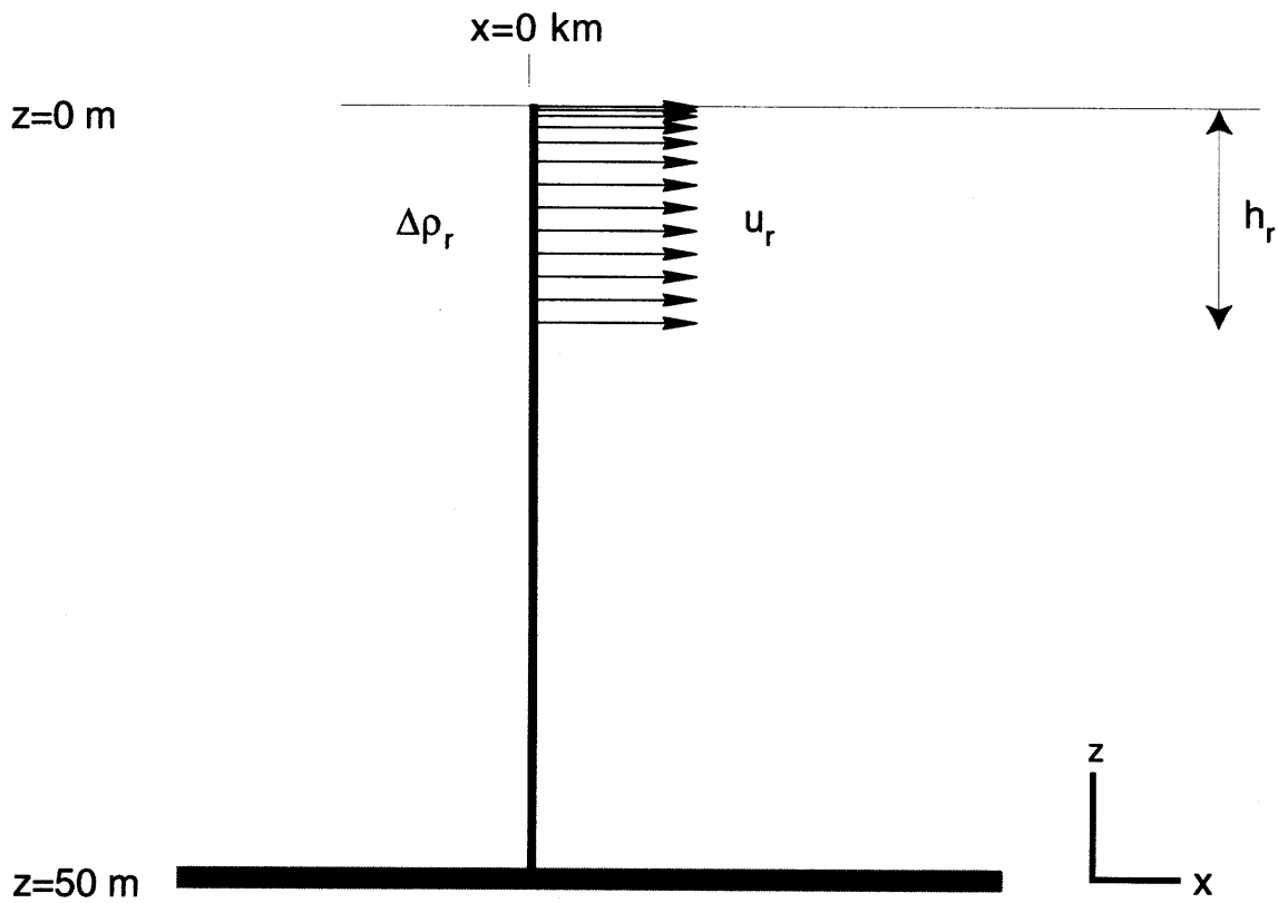
Figure 2.4: Schematic of river mouth forcing conditions. River discharge is accomplished through a uniform river discharge of water which differs in density from the ambient fluid by \Delta\rho_r . Discharge is accomplished through a river mouth of width L_r and depth h_r with velocity u_r .
