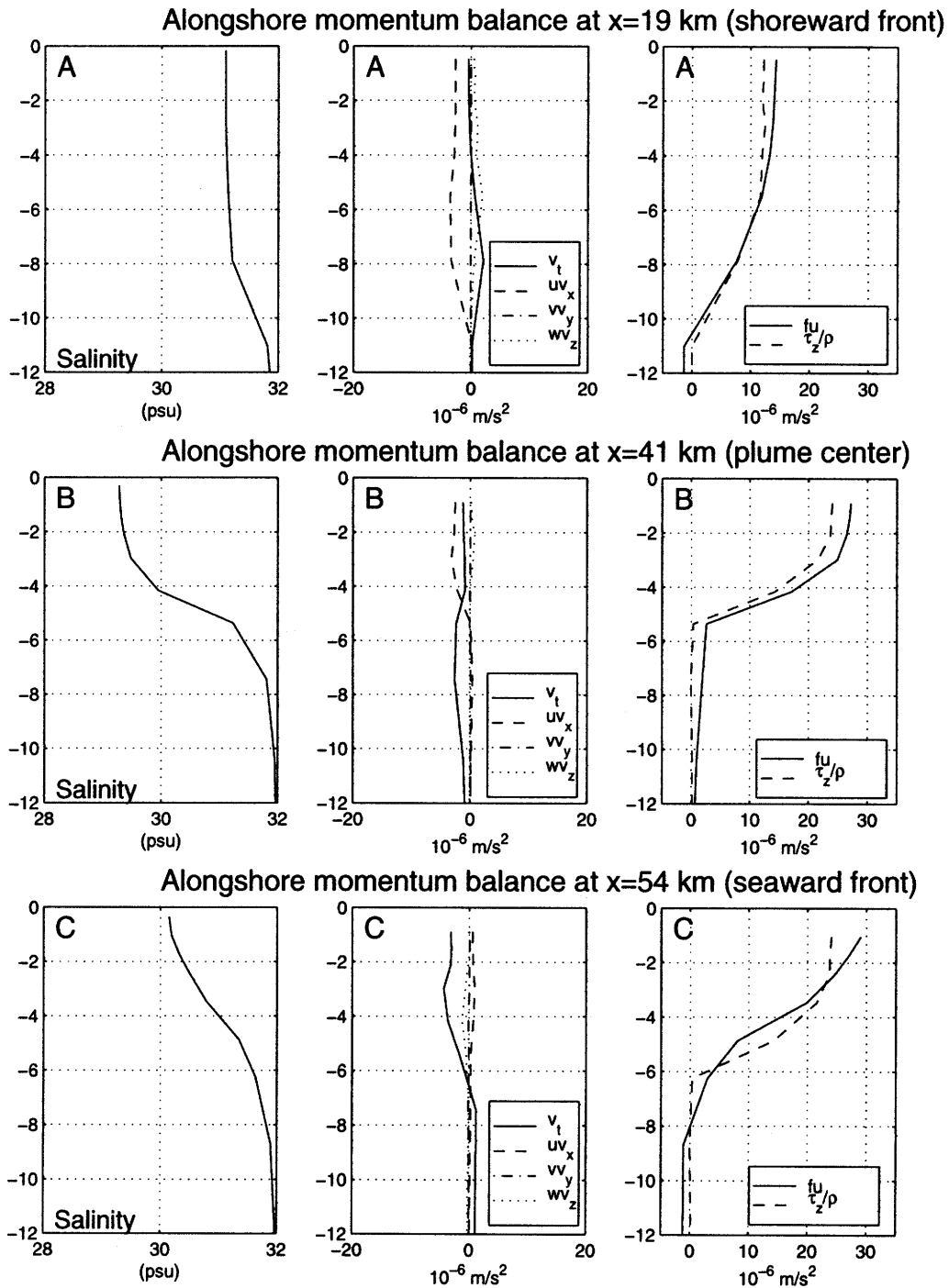
Figure 4.7: Salinity and Alongshore momentum balance terms at shoreward front (A), plume center (B), and seaward front (C) at t=48 hours. (for locations of profiles A, B, and C, see Figure 4.6). As noted in text, alongshore pressure gradient and horizontal diffusion terms are more than two orders of magnitude smaller than the Coriolis and stress divergence terms.
