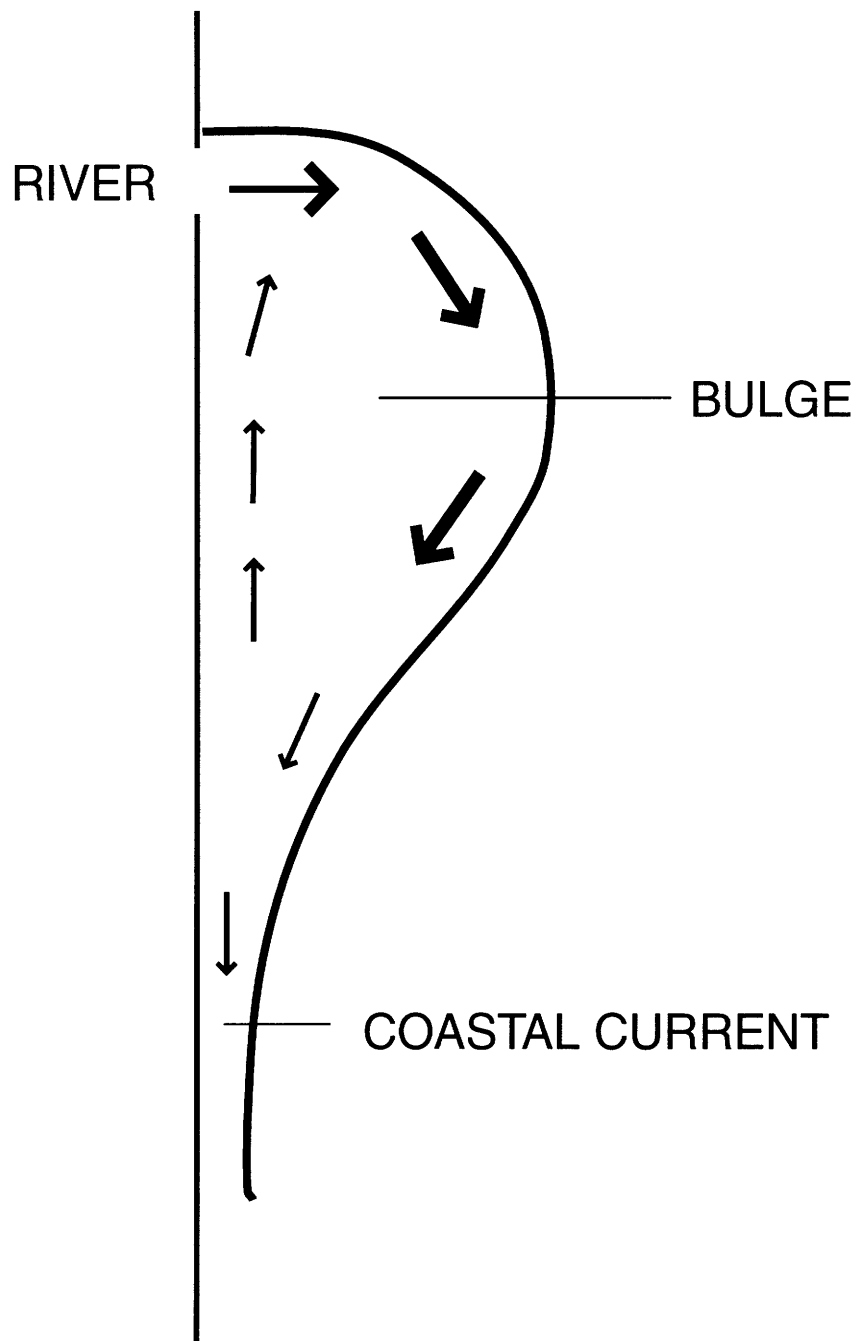
Figure 2.7: Cartoon of circulation within bulge and coastal current. The flow along the seaward side of the bulge transports water which supplies water to both the coastal current and the continually growing recirculation within the bulge.
