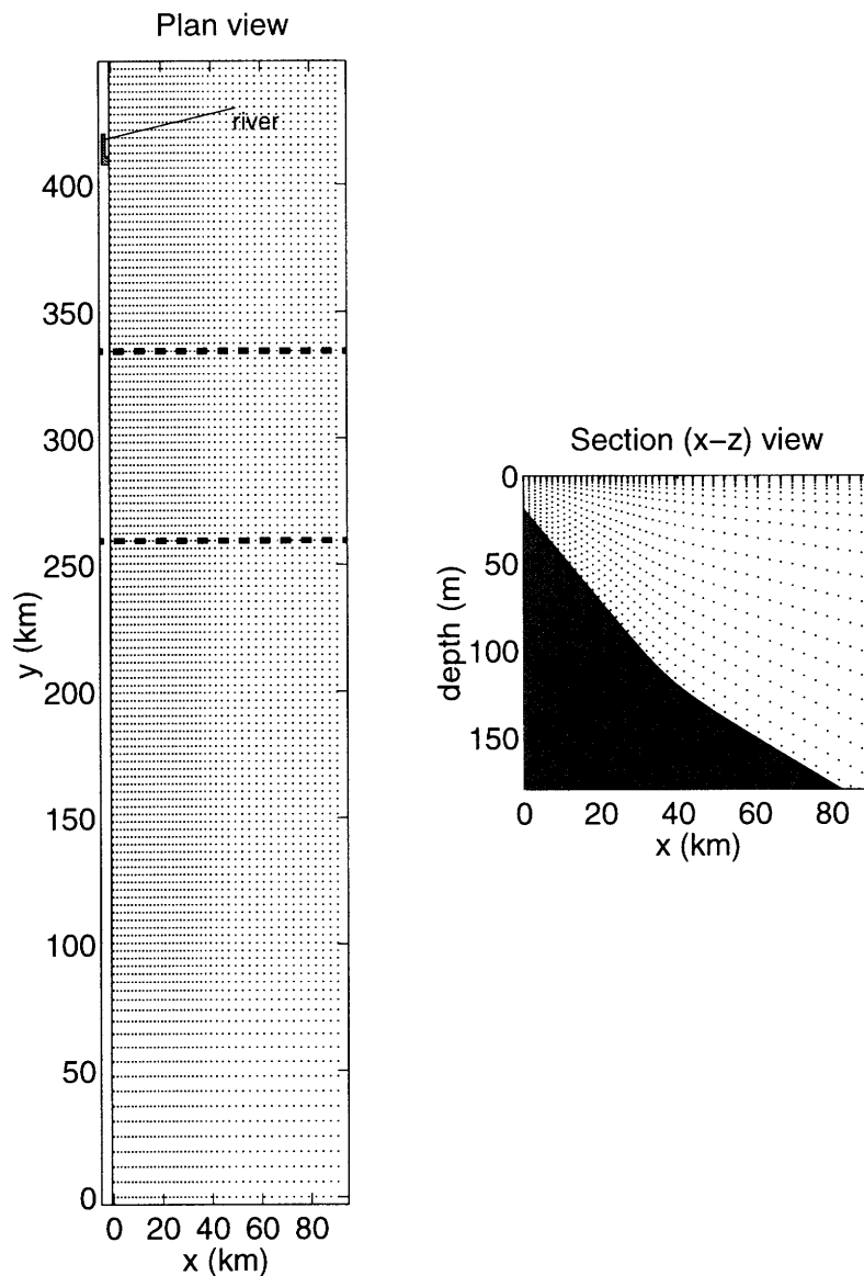
Figure 4.3: Model configuration. Blumberg and Mellor’s Estuarine Coastal Ocean Model-3d (ECOM-3D) is run on a 95 km x 450 km x 200 m grid. Grid resolution is indicated by small dots in both plan and section views. Vertical sigma levels are closely spaced at the surface to resolve the near surface plume behavior. The topography is chosen as an idealized version of a moderately steep continental shelf and is uniform in the alongshore ( y ) direction. Freshwater is discharged at the head of the estuary/river system shaded in gray in the northwestern (upper-left corner of the plan view) of the model basin. Dashed lines indicate the region over which a composite, alongshore-averaged cross-section is constructed to plot different property distributions.
