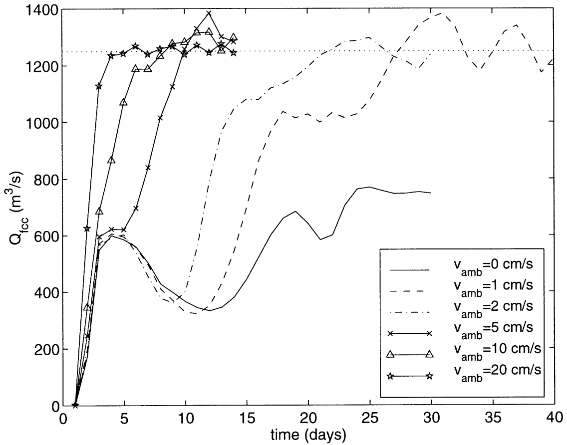
Figure 2.20: Freshwater transport as a function of time for different ambient flows at y=252 km. The dotted line indicates the freshwater discharged by the river: 1250 m 3 /s.
