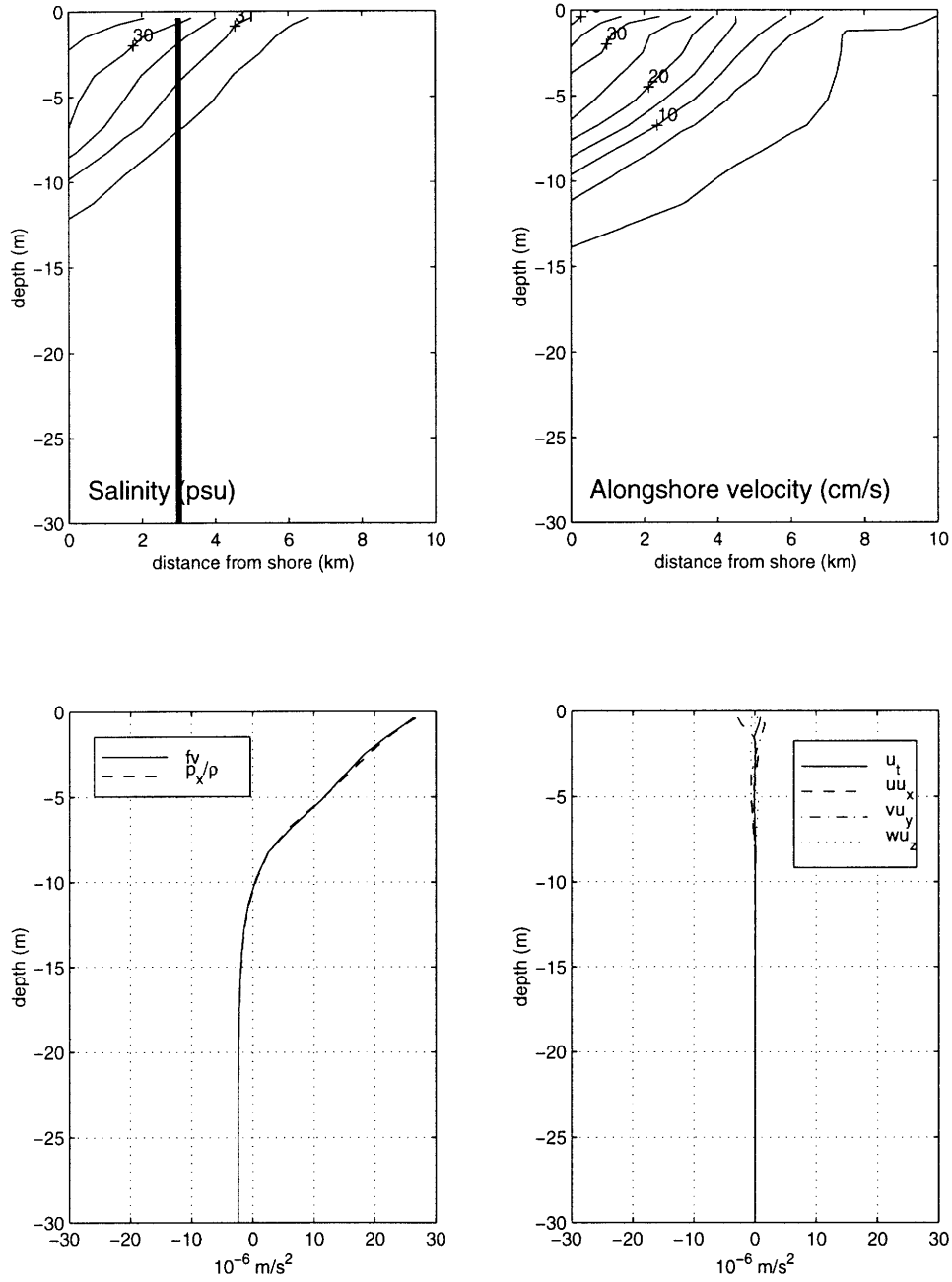
Figure 2.6: Sections of salinity (psu) and alongshore velocity are shown in the upper two panels. Profiles of terms in the cross-shore momentum balance are shown in the lower panels at the location given by the heavy vertical line overlying the salinity contours.
