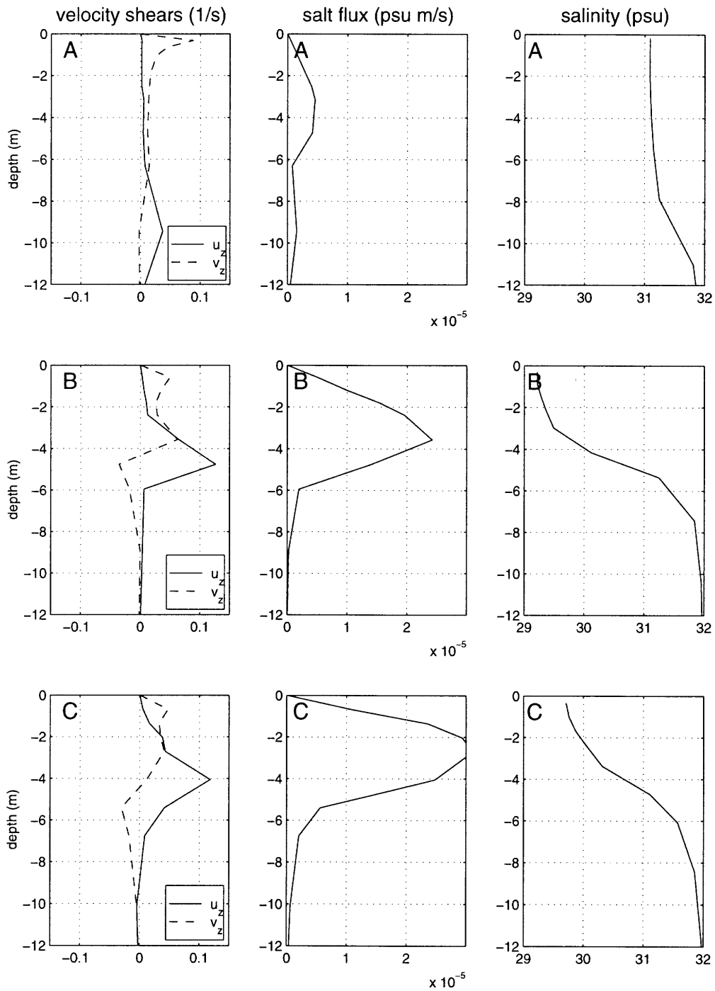
Figure 4.10: Profiles of velocity shears, salt flux, and salinity at the shoreward front (A), plume center (B), and seaward front (C) at t=48 hours (for locations of profiles A, B, and C, see Figure 4.6).
