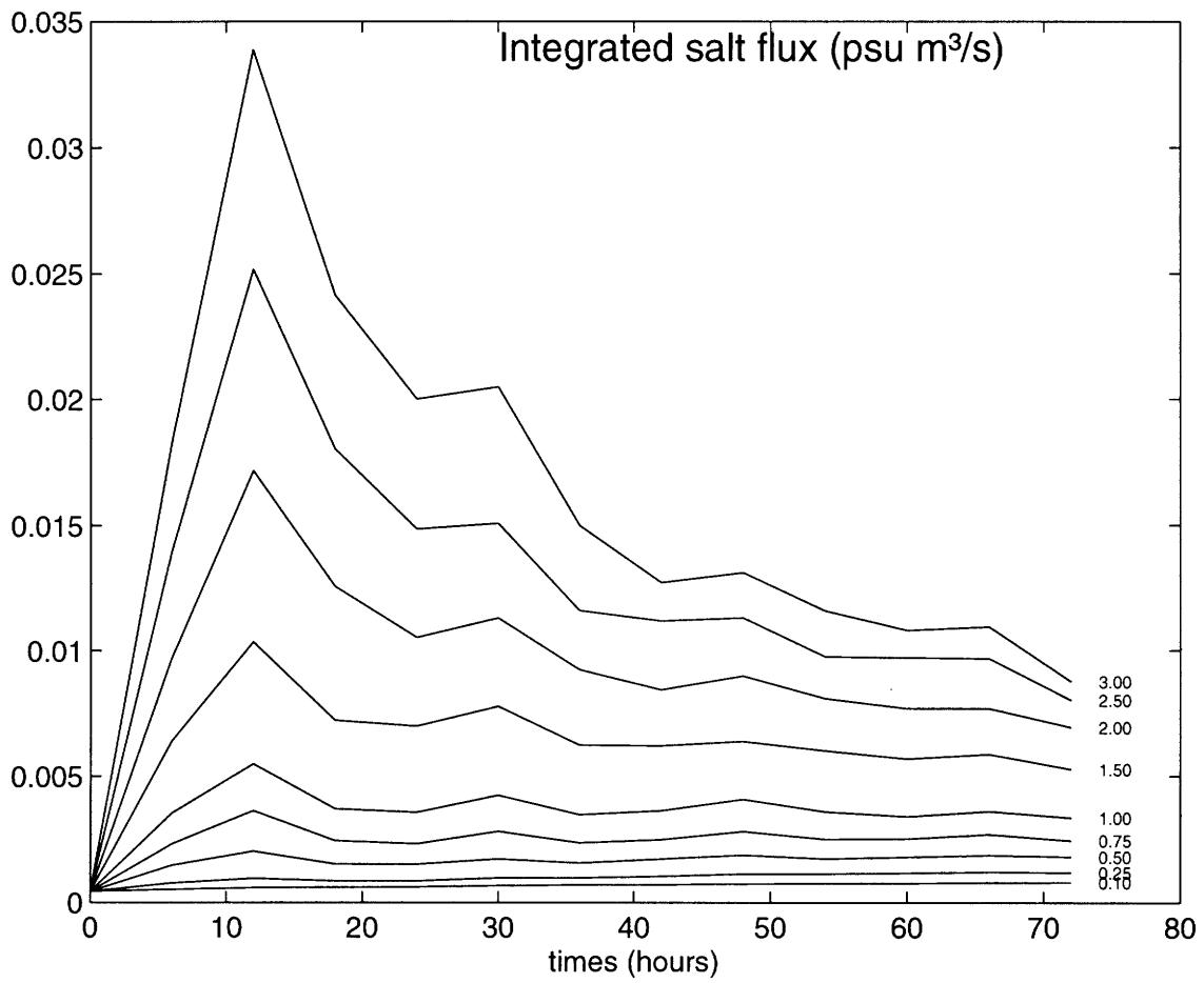
Figure 4.16: Integrated salt flux as a function of time for different wind stresses (in \text{dyne/cm}^2 ) for Runs 1-9.
