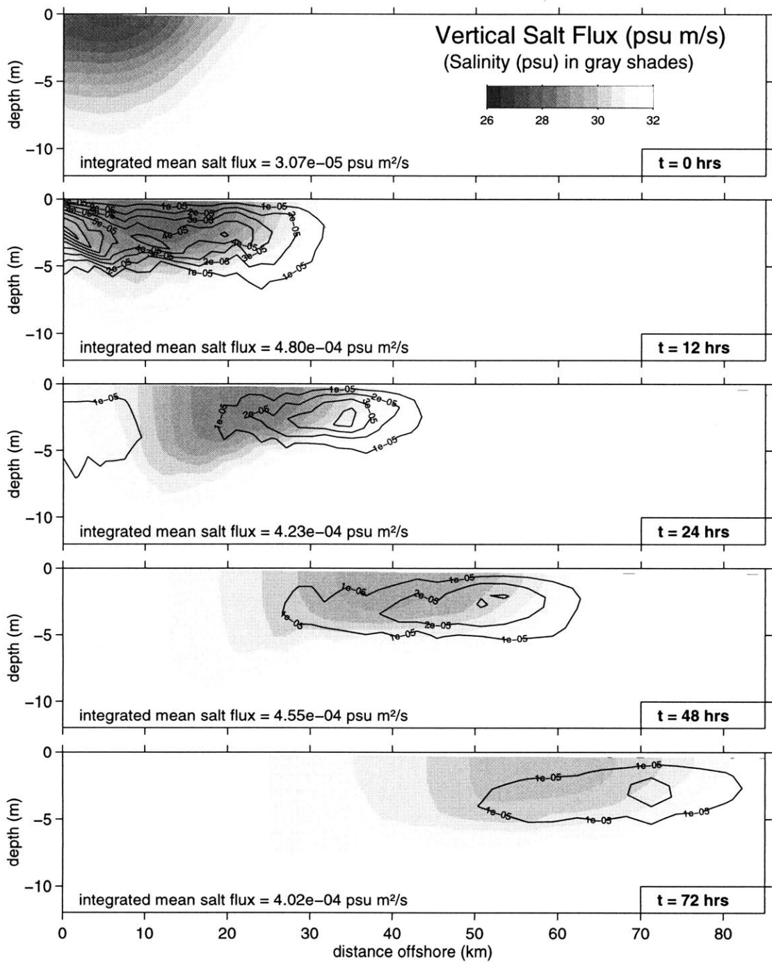
Figure 4.9: Contours of vertical salt flux and salinity for t=0, 12, 24, 48 and 72 hours. Gray contours are used to indicate salinity contours in intervals of 0.5 psu. Superimposed on the gray shading are contours of vertical salt flux in solid contour lines ( 10^{-5} psu m/s intervals). The cross-shore integrated mean vertical salt flux is indicated in the lower left corner of each panel.
