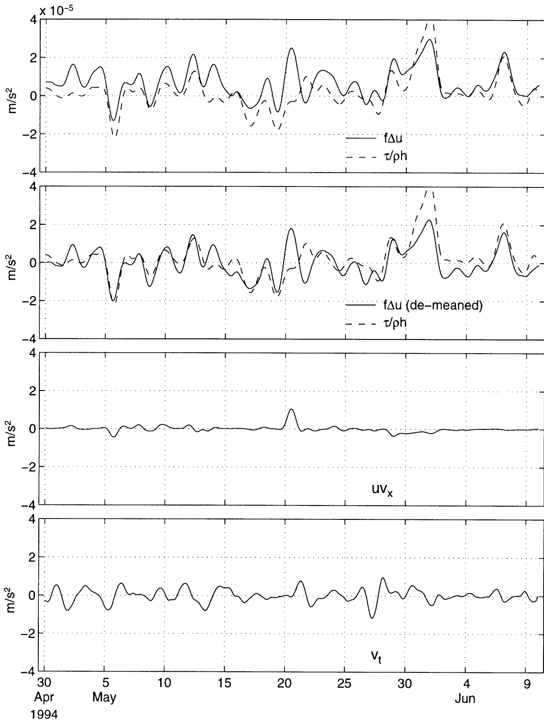
Figure 3.6: Time series of different terms in the shear alongshore momentum equation. Subscripts indicate partial differentiation.
