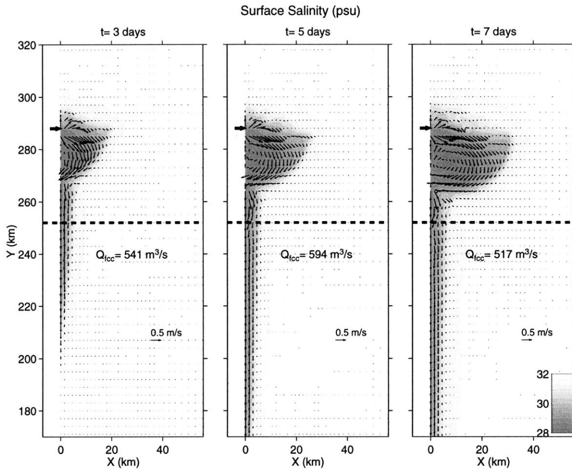
Figure 2.5: Surface salinity (psu), indicated by gray shading, for Base Case model run (Run 1) at t=3, 5, and 7 days. Velocity vectors are superimposed to indicate the flow field. Freshwater transport in coastal current is measure at y=252 km (indicated by dashed line). River mouth location is indicated by bold arrow.
