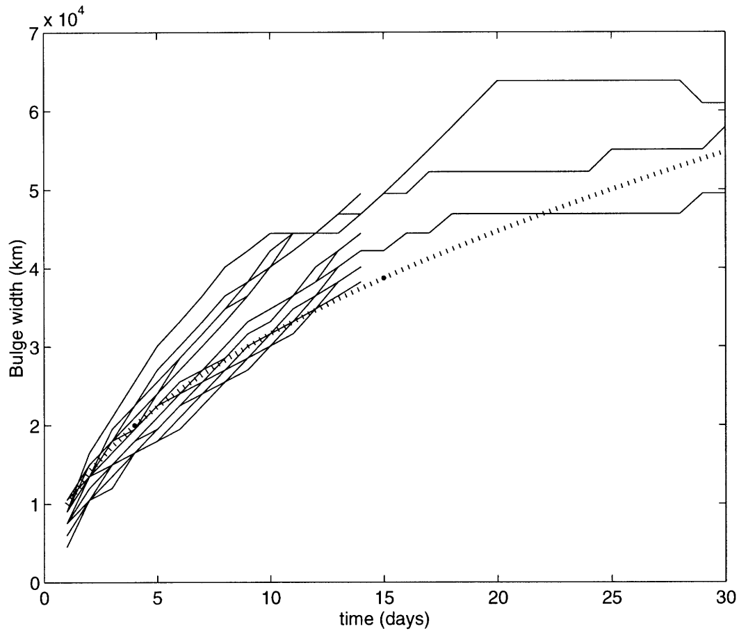
Figure 2.15: Bulge width (defined by the position of the 31.5 psu isohaline) as a function of time for different model runs. The bulge width is approximately proportional to the square root of time for the different model runs (the dotted line denotes a t^{1/2} dependence). Note: Bulge widths for t > 20 days may not be accurate due to interactions of the bulge with the offshore boundary of the model domain.
