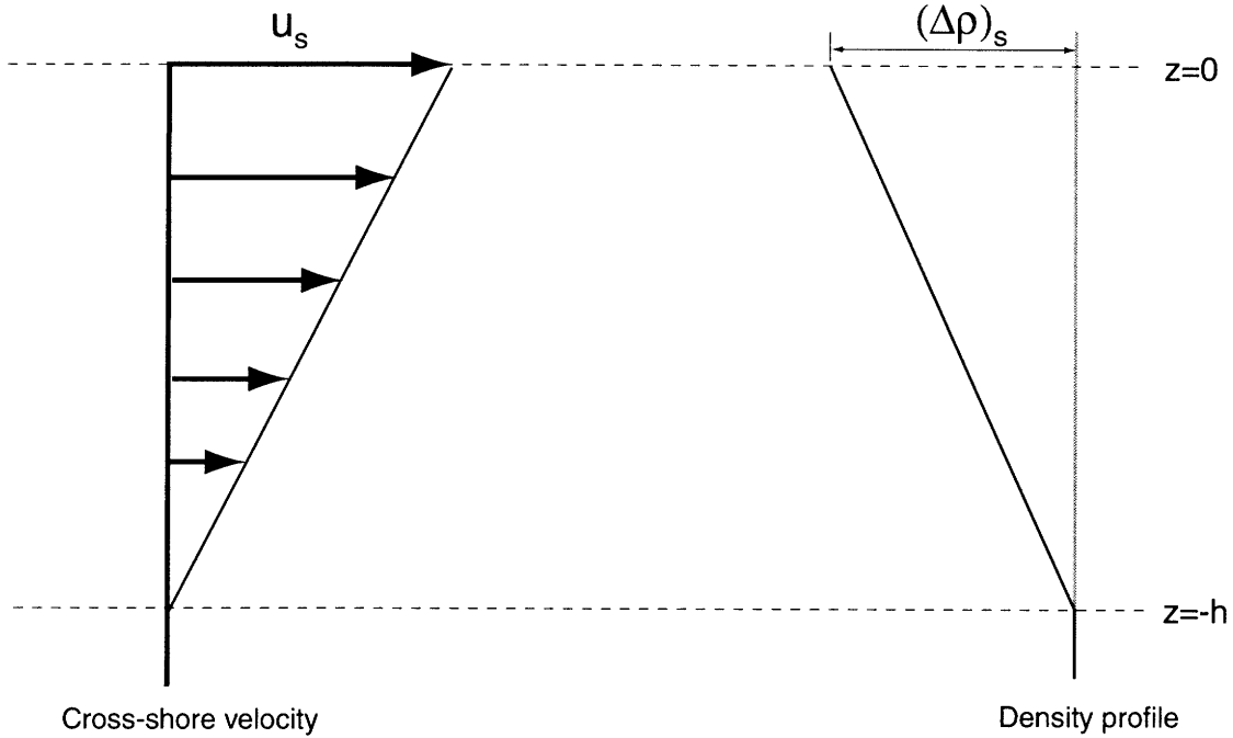
Figure 4.1: Velocity and density profiles in simple theory. The cross-shore velocity varies linearly from u_s at the surface to the bottom of the plume ( z = -h ) and vanishes beneath the plume. The density anomaly is also assumed to vary linearly within the plume with its maximum at the surface (\Delta\rho)_s . Note: the mean density anomaly \overline{\Delta\rho} = (\Delta\rho)_s/2 .
