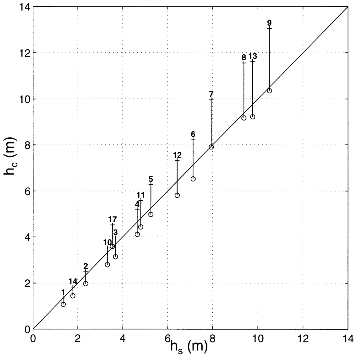
Figure 4.14: Numerical model plume thickness (at t=72 hours) h_s versus equilibrium thickness h_c for Ri_c = \frac{1}{2} (o) and Ri_c = 1 (+)
