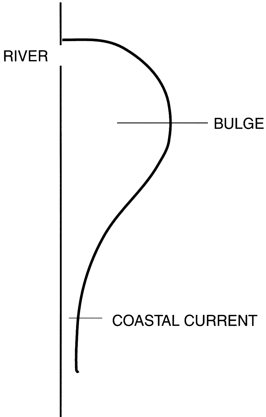
Figure 1.1: Cartoon of surface-trapped plume.
