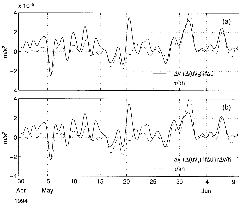
Figure 3.7: Balancing the shear alongshore momentum: (a) excluding interfacial friction (b) including interfacial friction.
