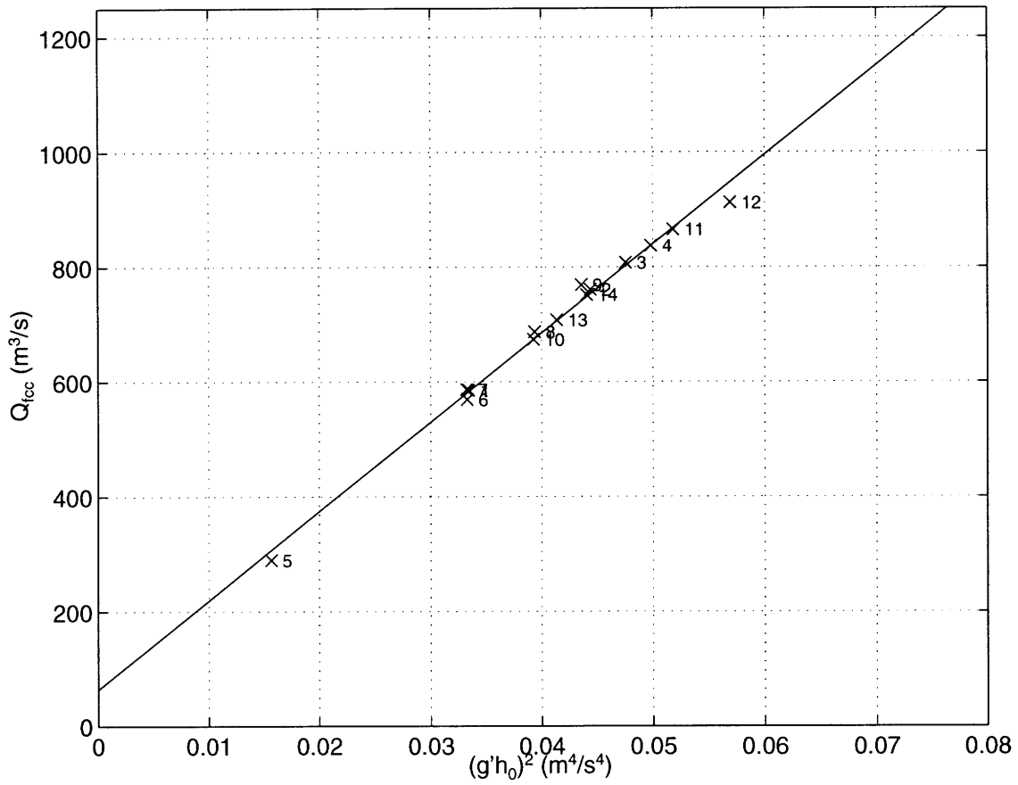
Figure 2.9: Model freshwater transport Q_{fcc} in coastal current at t=5 days, y=252 km, as a function squared potential energy in coastal current. Run numbers are indicated for each data point (see Table 2.2).
