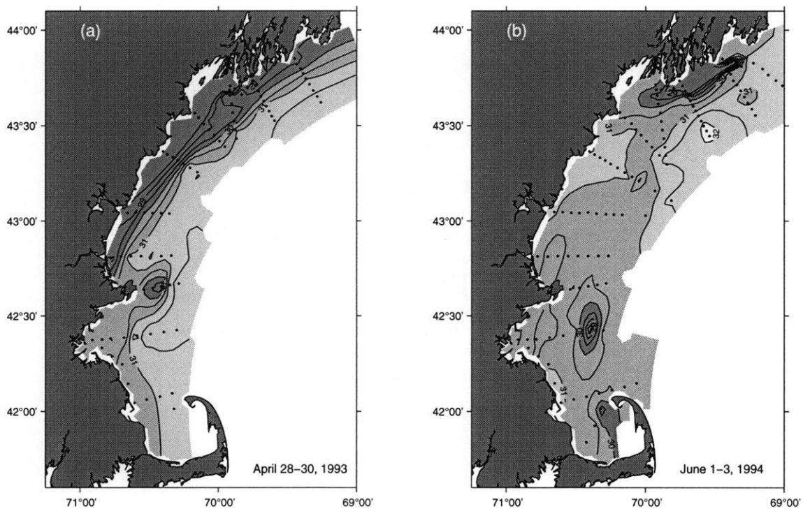
Figure 3.4: Horizontal sections of salinity at 2.5 meters depth based on Hydrographic surveys (stations indicated by dots). (a) Downwelling favorable wind conditions (Cruise 93-3: April 28-30, 1993), (b) Upwelling favorable conditions (Cruise 94-6a: June 1-3, 1994).
