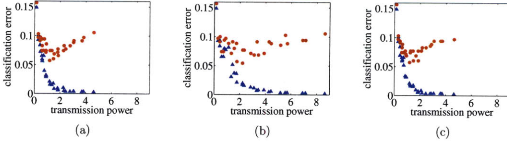
Figure 4.16. Tenfold cross-validation training error (blue triangle markers) and test error (red circle markers) on ionosphere dataset for (a) parallel, (b) serial, and (c) binary tree network architectures.
