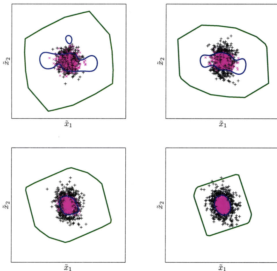
Figure 4.3. Joint linear dimensionality reduction and margin-based classification coordinate descent with the SVM classifier proceeding in raster scan order from top left to bottom right. The magenta \times markers indicate class label -1 and the black + markers indicate class label +1 . The blue line is the decision boundary. The green line outlines the zonotope Z(\mathbf{A}) .
