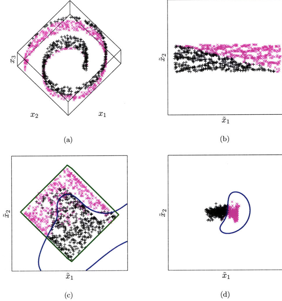
Figure 4.8. The (a) swiss roll dataset, (b) its Isomap embedding, (c) joint linear dimensionality reduction and SVM classification solution, and (d) joint nonlinear dimensionality reduction and SVM classification solution. The magenta \times markers indicate class label -1 and the black + markers indicate class label +1 . The blue line is the decision boundary. The green line outlines the zonotope Z(\mathbf{A}) in (c).
