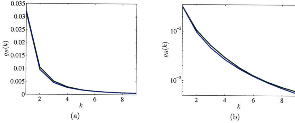
Figure 5.7. Mean Bayes risk error for MBRE-optimal quantizer (blue line) and MAE-optimal quantizer (green line) on (a) linear scale, and (b) logarithmic scale with beta(5,2) p_- and c_{+-} = 1 , c_{-+} = 1 .
