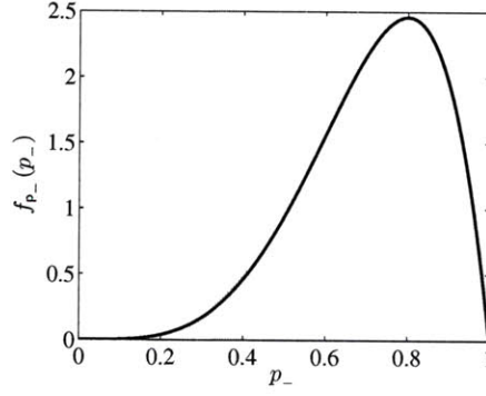
Figure 5.6. The beta(5,2) probability density function.
