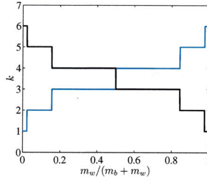
Figure 5.18. Optimal allocation of quantizer sizes to population b (black line) and population w (cyan line) for k_t = 7 as a function of m_w/(m_b + m_w) with \text{beta}(5,2) p_- and c_{+-} = 1 , c_{-+} = 1 .
