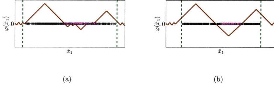
Figure 4.4. Joint linear dimensionality reduction and GLS classification. The magenta \times markers indicate class label -1 and the black + markers indicate class label +1 . The maroon line is the signed distance function whose zero level set forms the decision boundary. The dashed green line delimits the zonotope generated by \mathbf{A}^T . The initial and final dimensionality reduction projection and signed distance function are in (a) and (b) respectively.
