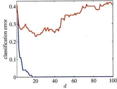
Figure 4.6. Training error (blue line) and test error (red line) on arcene dataset.
