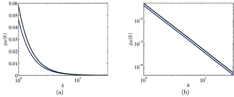
Figure 5.13. High-rate approximation to mean Bayes risk error for MBRE-optimal quantizer (blue line) and MAE-optimal quantizer (green line) on (a) linear scale, and (b) logarithmic scale with \text{beta}(5,2) p_- and c_{+-} = 1 , c_{-+} = 1 .
