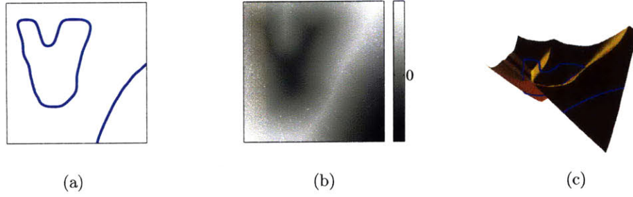
Figure 2.2. An illustration of the level set function representation of a contour with D = 2 . The contour is shown in (a), its level set function is shown by shading in (b), and as a surface plot marked with the zero level set in (c).
