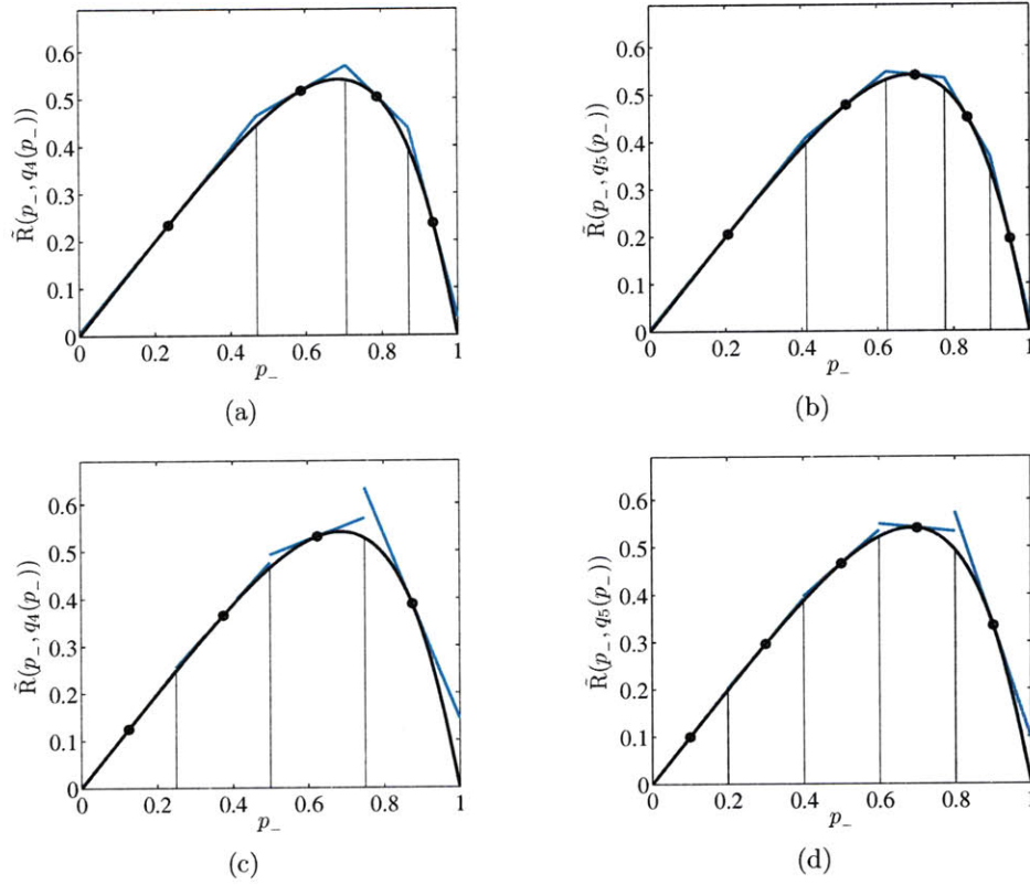
Figure 5.5. (a)–(b) MBRE-optimal, and (c)–(d) MAE-optimal quantizers for k = 4, 5 with uniform \rho_- and c_{+-} = 1 , c_{-+} = 4 .
