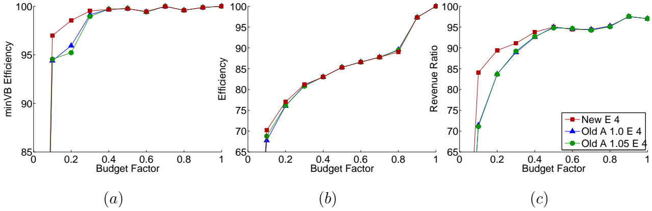
Figure 4: L2 Legacy – Uniform and Linearly Random – 20 items and 20 bidders with 15 bundles per bidder.
