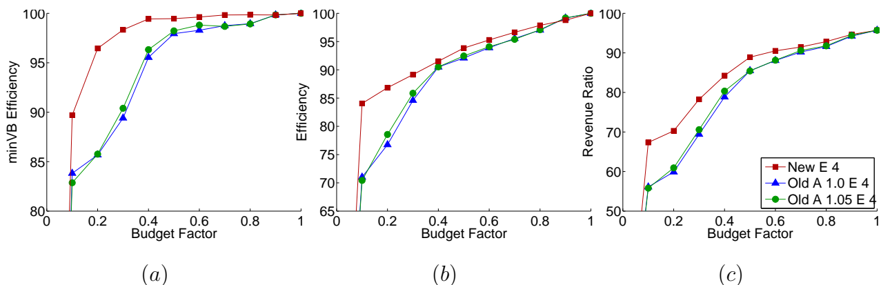
Figure 3: L4 Legacy – Decay and Linearly Random – 20 items and 20 bidders with 12.5 bundles per bidder.
