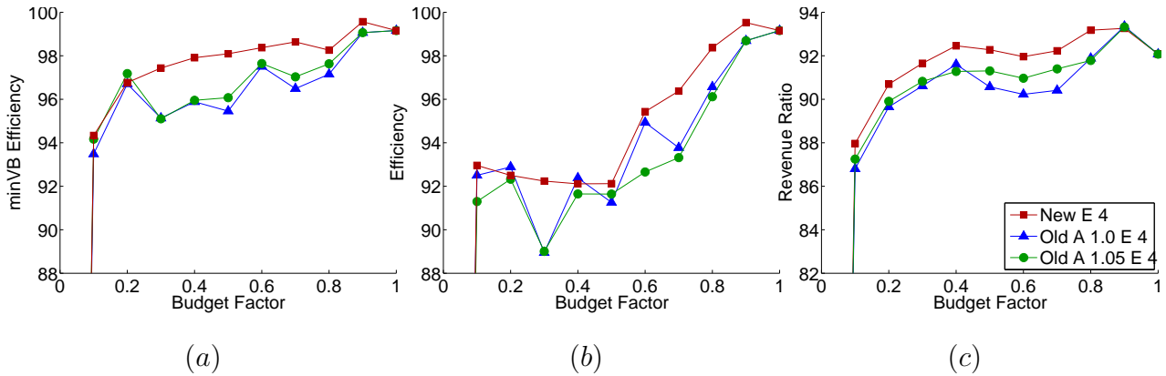
Figure 6: CATS – Arbitrary – 25 items and total number bundles randomly chosen between 400–500 (resulting in an average of 8.4 bundles per bidder and 26 bidders).
