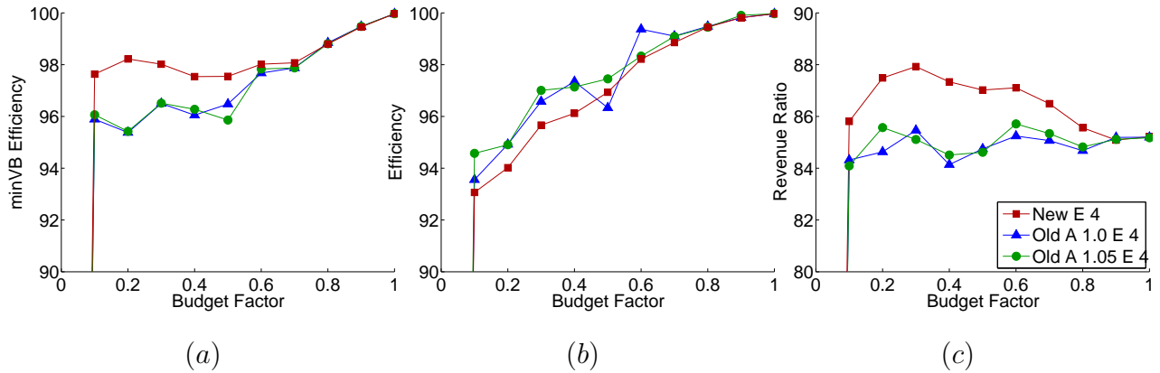
Figure 7: CATS – Scheduling – 25 items and total number of bundles randomly chosen between 200–400 (resulting in average of 18.6 bundles per bidder and 18 bidders.)
