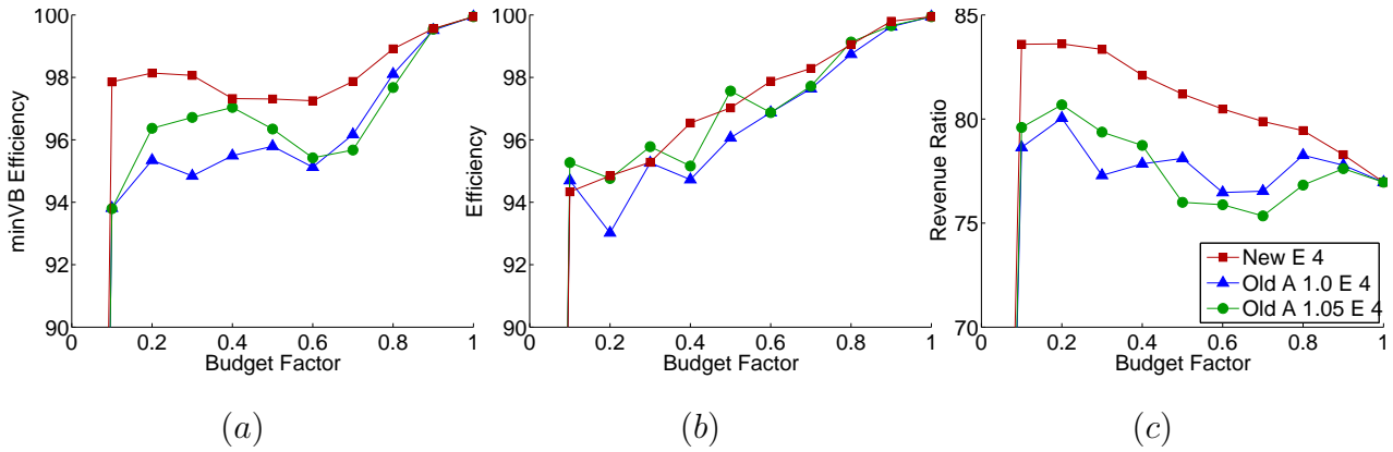
Figure 5: CATS – Matching – 32 items and total number of bundles randomly chosen between 400–500 (resulting in average of 13.3 bundles per bidder and 34 bidders).
