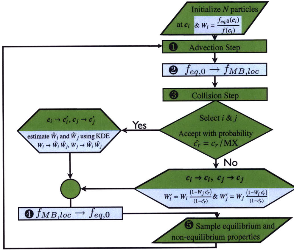
Figure 5-2: Final VRDSMC flowchart. Note that the only difference between this algorithm and the one shown in Figure 3-4 are the steps 2 and 4. These are the steps that change the reference state in the equilibrium simulation to and from a local Maxwell-Boltzmann state.
