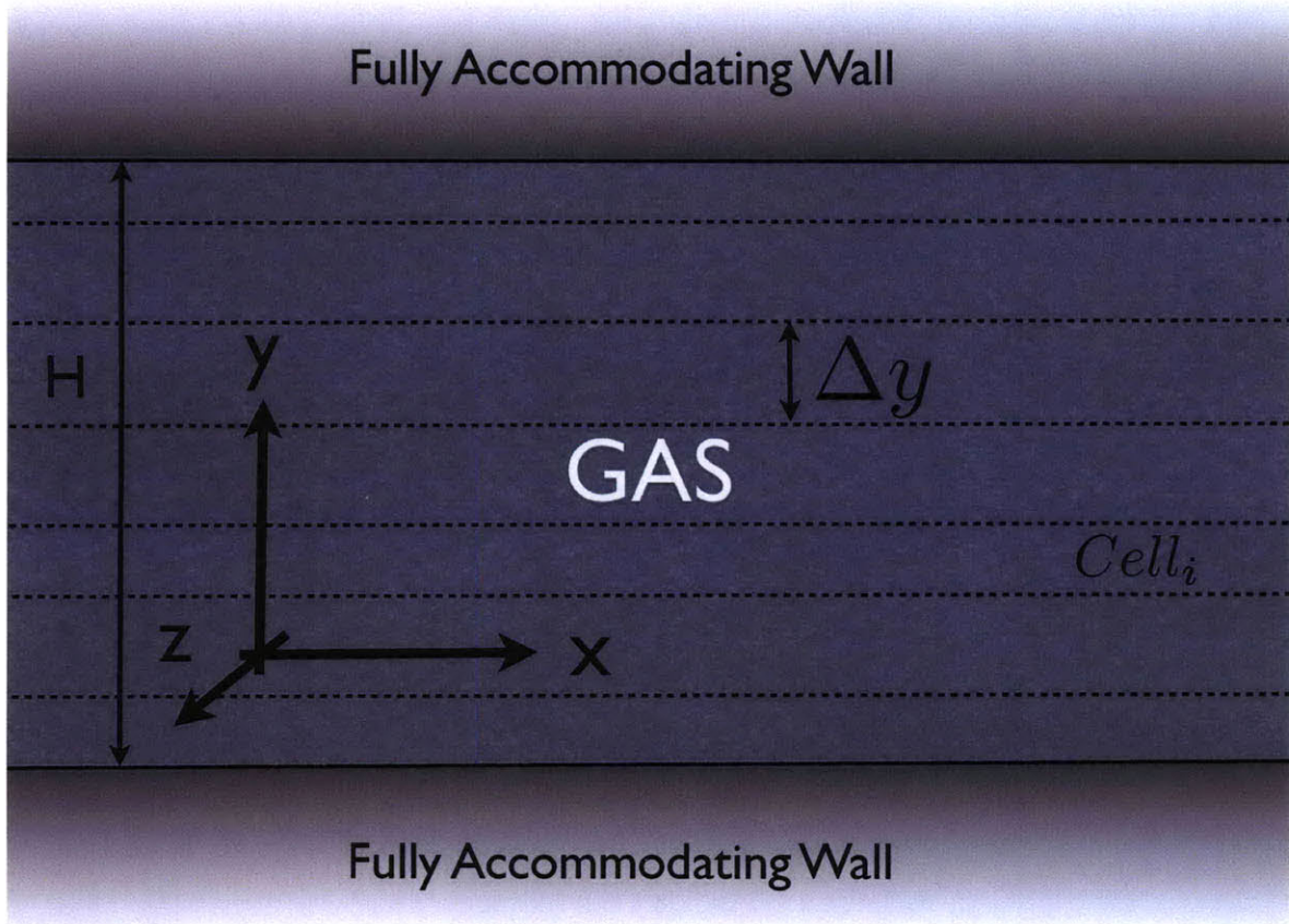
Figure 3-5: Schematic of the physical setup of our one-dimensional validation problems.
