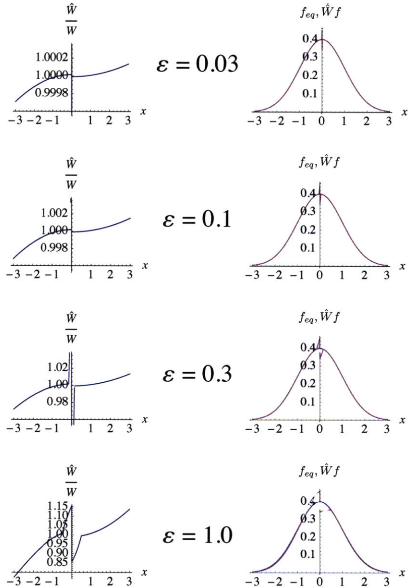
Figure 7-2: The introduction of bias in the estimates of weights is the primary cause of error in VRDSMC simulations. In this Figure, we see that as \epsilon \rightarrow 0 the bias introduced goes to 0. In this figure the left column shows the ratio of \hat{W}/W , while the right column shows f_{eq} vs. \hat{W}f .
