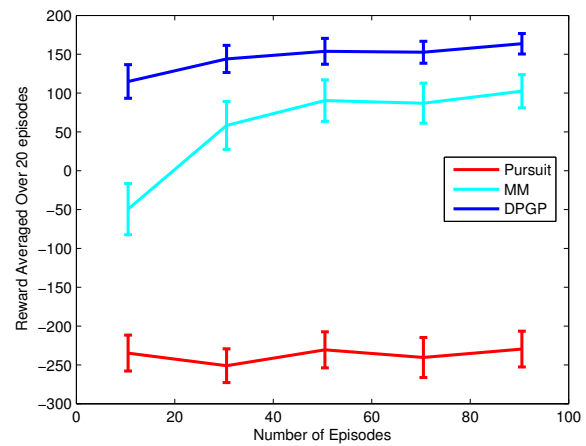
Fig. 13 Sliding window average of per-episode rewards achieved by different models on the BLOCKS scenario. Error bars show the 95% confidence interval of the mean from five repeated runs.
