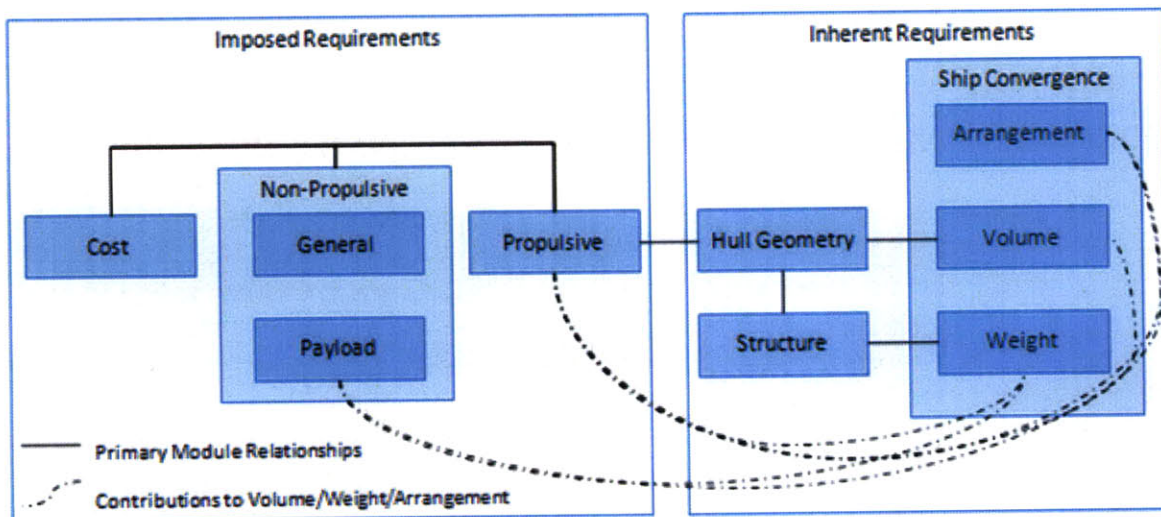
Figure 11 SUBSTART Modularization
