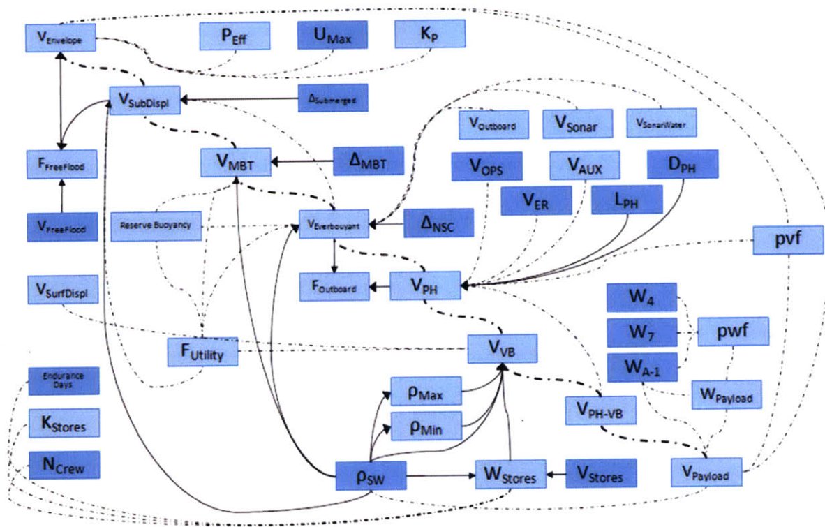
Figure 19 Alternate Configuration – Primary and Secondary Values
