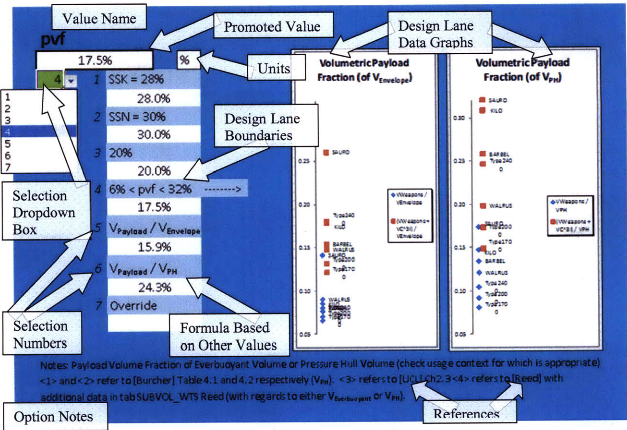
Figure 13 SUBSTART Data Structure Labeled Example – pvf
