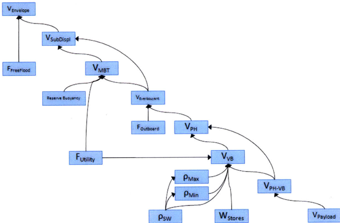
Figure 17 Primary and Secondary Values
