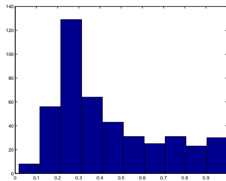
Figure 13: Center crack problem: Histogram of \beta^{\text{LB}}(\mu)/\beta(\mu) for \Xi_{\text{test}} ; \min_{\mu \in \Xi_{\text{test}}} \frac{\beta^{\text{LB}}(\mu)}{\beta(\mu)} = 0.018 , \text{avg}_{\mu \in \Xi_{\text{test}}} \frac{\beta^{\text{LB}}(\mu)}{\beta(\mu)} = 0.438 .
