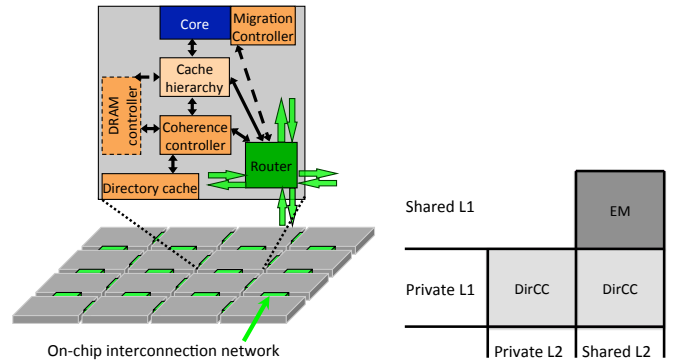
(a) Fully distributed tiled multicore (b) On-chip cache organization Fig. 1. Every tile has an in-order core, a cache hierarchy, a router, a coherence migration controller and a slice of the distributed directory cache. An execution migration controller allows each core to access another tile via the interconnect. Tiles connected to off-chip DRAM have a DRAM controller.
