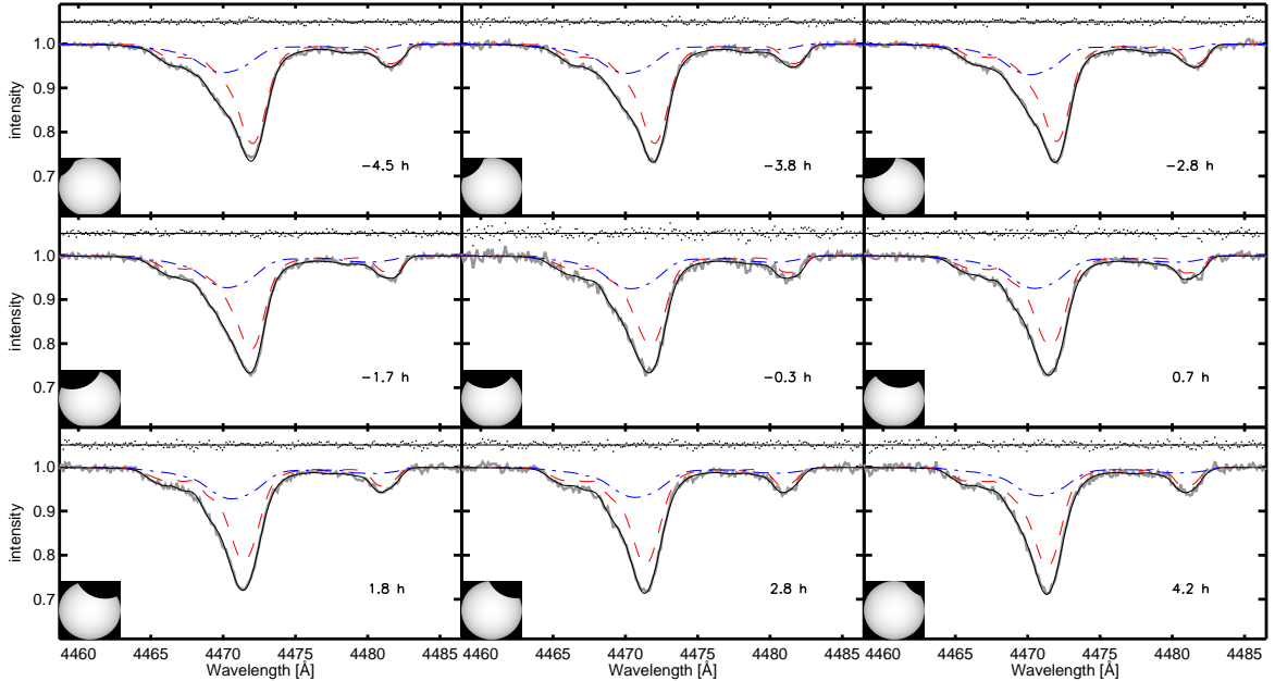
FIG. 7.— Observations of NY Cep during primary eclipse. Similar to Figure 6, but for spectra obtained during primary eclipse. The number in each panel indicates the time from mid-eclipse, in hours. The corner of each panel shows an illustration of the eclipse phase. In the best-fitting model, \beta_p = 2 \pm 4^\circ , indicating a close spin-orbit alignment. Focusing on the Mg II line, one can see in particular for the observations at -2.8 h and 2.8 h how the RM-effect creates a redshift during the first half of the eclipse and a blue shift during the second half of the eclipse. For the observation at -0.3 h, near mid-eclipse, blue and redshifted light are blocked by similar amounts.
