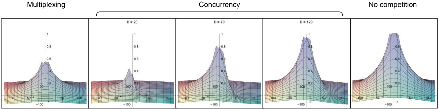
Figure 2 – Capacity “landscape” C_i(r, \theta) ; \alpha = 3, \sigma = 0, P_0 / N_0 = 65\text{dB} . Depicts capacity as a function of receiver position (x-y plane), with the sender at the origin and an interferer on the x-axis at distance D . D is identified explicitly for the concurrency cases, but not for multiplexing, where capacity is independent of D . The “no competition” case is equivalent to concurrency with D \rightarrow \infty . Distance units are in multiples of the P = 65\text{dB} unit distance.
