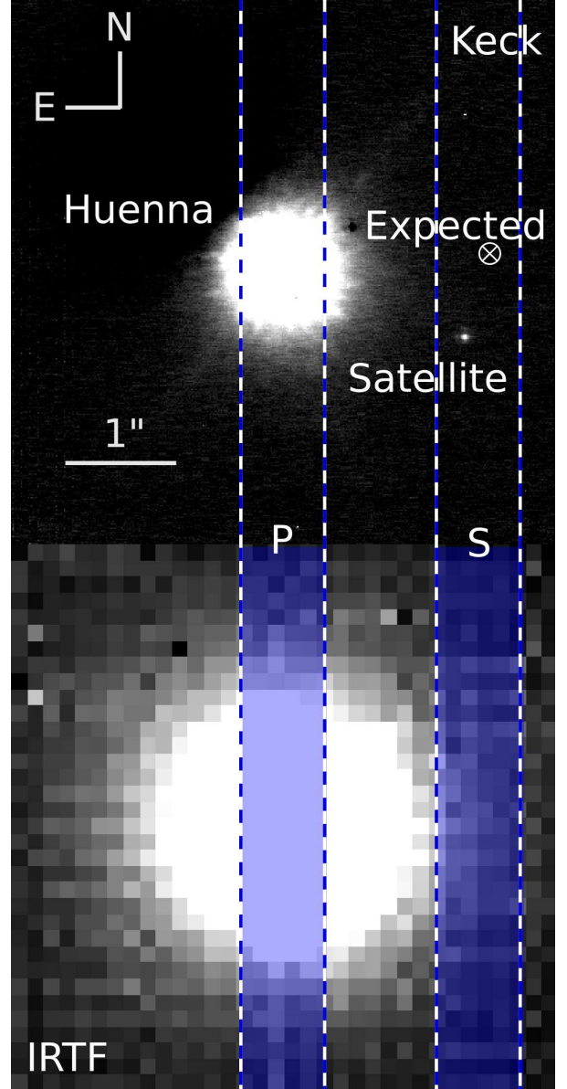
Figure 1: Observing configuration: P marks the position of the slit for observations of the primary using the IRTF observations. S marks the position for the secondary which was chosen based on the expected position of the secondary. Top : Adaptive-optics image obtained with NIRC2 at the Keck telescope. Bottom : Image obtained at the IRTF with SpeX slit-viewer, displayed at the same scale. Both images are oriented with north up and east left. The plate scale of the IRTF spectrograph and IRTF guider (slit-viewer) are 0.15 and 0.12''/pixel, respectively.
