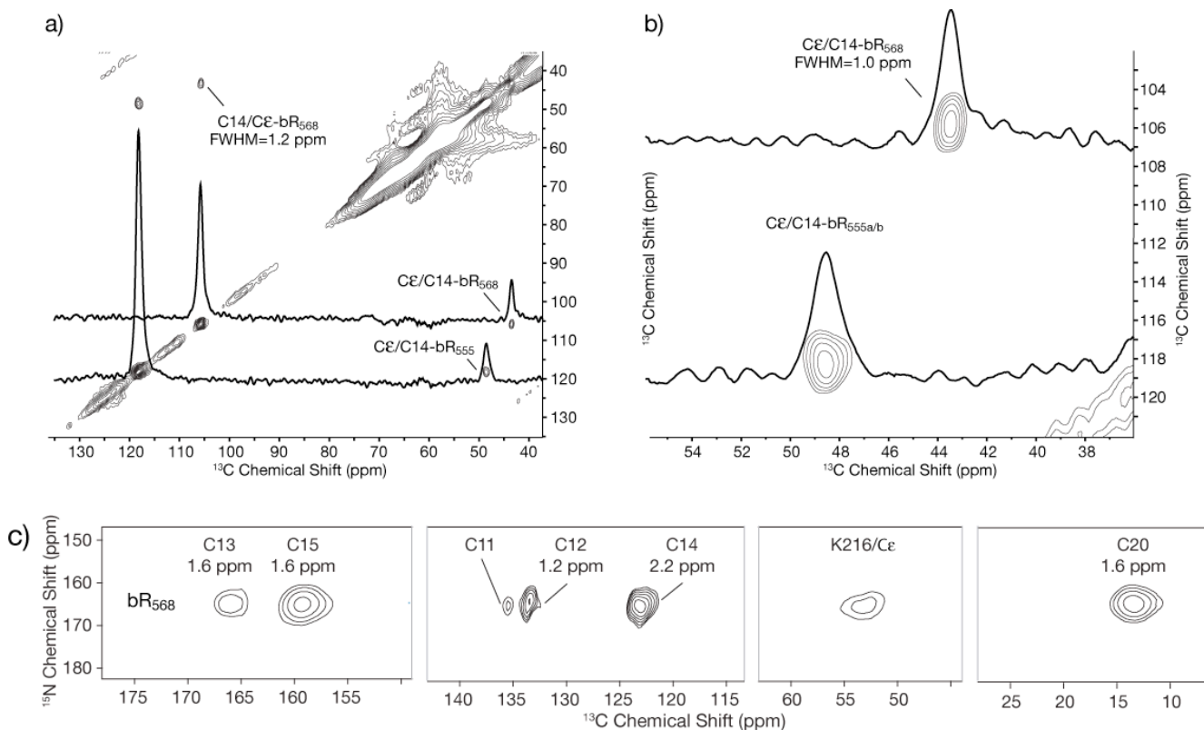
Fig. 1 High resolution DNP spectra of bR. a) RFDR correlation spectrum of 14 mg of ^{14}\text{C} -retinal, [\epsilon\text{-}^{13}\text{C}] lysine-labeled bR in the dark-adapted state with 1D direct ^{13}\text{C} dimension slices overlaid on the 2D contours. 12.5 days worth of acquisition time from mixing times between 8 and 28 ms were averaged together. The resulting signal-to-noise negated the need for any line-broadening. The bR 568 correlation in the upper left has a linewidth of 1.2 ppm (115 Hz) b) Expansion of the lower right portion of the spectrum in (a) demonstrating the narrow linewidths achievable with MAS DNP. Whereas the bR 555 correlation is slightly broader due to the presence of two conformations of bR 555 , the bR 568 resonance is extremely narrow with a linewidth of 1.0 ppm (95 Hz). c) Carbon-nitrogen 2D spectrum of uniformly ^{13}\text{C} , ^{15}\text{N} -labeled bR 568 . 21 After an indirect chemical shift evolution on the resolved Schiff base (165 ppm in the ^{15}\text{N} dimension), the magnetization is transferred along the retinal chain all the way to C11, and also in the other direction directly to C \epsilon . The carbon resonances show relatively narrow linewidths (1.2-2.2 ppm).
