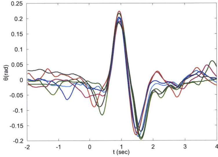
Figure 5-5: A sample of LQR-controller perturbation trajectories in \theta . Note that given the variation during normal operation, detection is difficult until the vortex has significantly perturbed the system. See Fig. 5-6 for a close up on the time at which the perturbation is just beginning.
