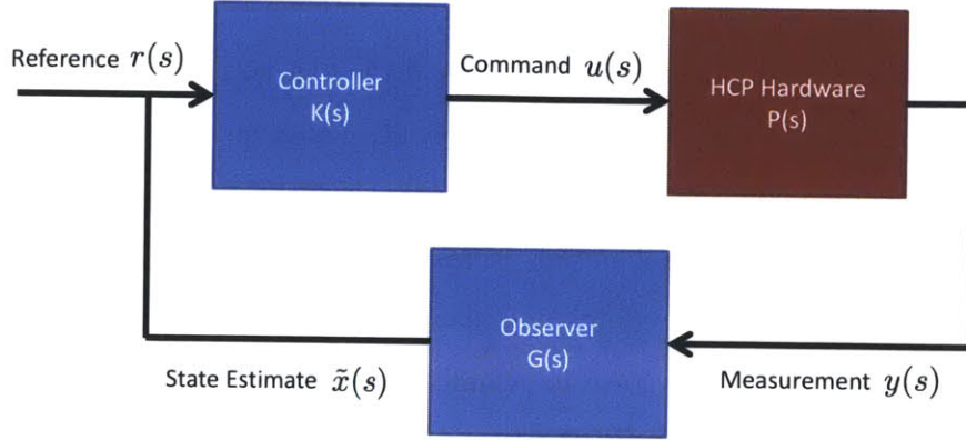
Figure 3-1: A schematic representation of the linear control loop for the HCP. When PIV is included in §5 the components needed to handle the additional sensing add complexity, but for now this simpler understanding will suffice. In general, a nonlinear observer G(y, u) is used, but near the upright a linear G(s) is sufficient.
