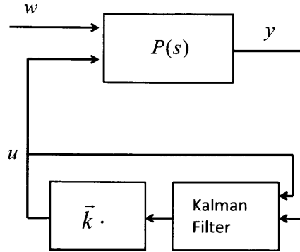
Figure B-2: Block diagram of the State Feedback Gain parameterization with a fixed observer. Controllers are parameterized by selecting n scalar gains k_1 through k_n where n is the number of states of the system.
