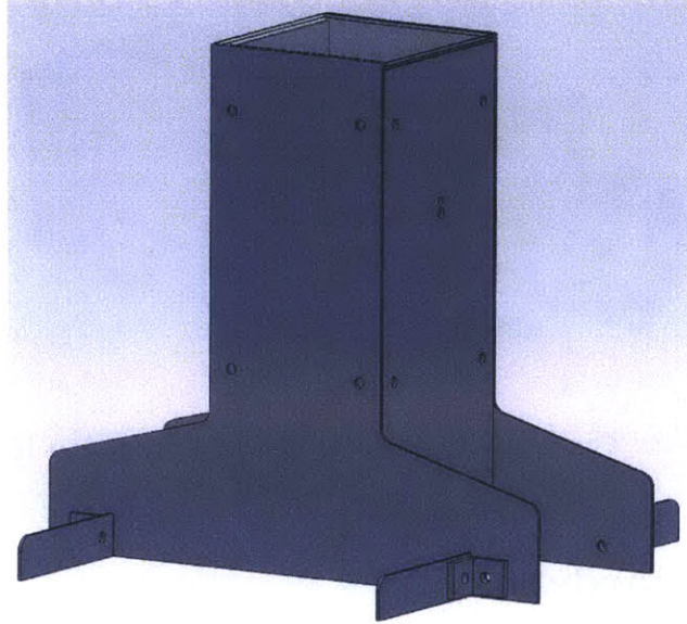
Figure A-4: SolidWorks rendering of box built to mount camera, and protect it from any droplets of water leaked from the test section.
