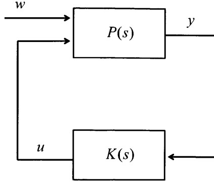
Figure B-1: Block diagram of the system used for Direct K(s) Learning. Controllers are parameterized by selecting a linear system K(s) , with the specific form shown in Eq. (B.1).
