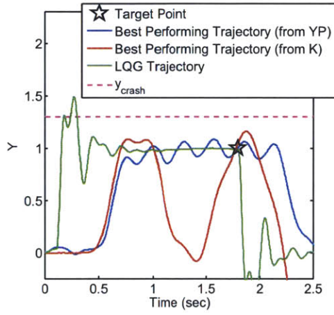
Figure B-7: Tracking performance of resulting controllers from the YP, LQR Cost Matrices Learning and Direct K(s) Learning. Note that while all three parameterizations shown here hit the target point well for the nominal values, randomization of v_b (as well as greater use of actuation) degraded the performance of the controller from Direct K(s) Learning and overshoot that could not be eliminated by learning caused the LQR Cost Matrix controller to incur unacceptable cost. As a result, the Youla Parameterization controller achieved the best performance.
