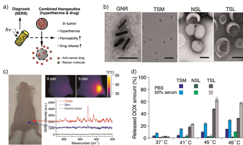
Figure 1. Characterization of the two components of a cooperative nanosystem. a) Schematic diagram depicting the cooperative nanomaterials system. b) TEM images of PEG-coated GNR, TSM, NSL, and TSL. The scale bars are all 100 nm. c) Optical image, thermal images, and Raman spectra of a mouse depicting the multifunctionality of the GNRs. The GNRs act as thermal transducers or as SERS contrast agents when irradiated with a laser of the appropriate wavelength and intensity. The mouse, bearing a MDA-MB-435 tumor, was injected intravenously with GNRs ( 10 \text{ mg Au kg}^{-1} ). The IR thermographic maps shown were obtained 24 h post-injection; the left image was acquired immediately before and the right image 5 min after onset of irradiation with a diode laser ( \lambda = 810 \text{ nm} , 0.75 \text{ W cm}^{-2} ). Raman spectra (5 acquisitions of 60 s each) were acquired from the tumoral region (red trace) and from skin near the tumor (blue trace). The GNRs in this experiment were labeled with a cyanine dye and the peaks in the trace correspond to the SERS spectrum cyanine dye (verified by in vitro control). d) Amount of DOX released in vitro from the liposome and micelle formulations used in this study, as a function of temperature. The samples were incubated for 10 min at the indicated temperatures and the amount of free DOX was quantified by fluorescence spectroscopy, relative to a standard curve. Values represent the mean and the error bars indicate standard deviation.
