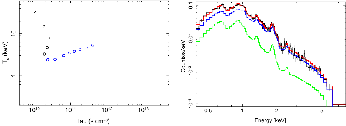
Fig. 11.— Left: The distribution of kT_e and \tau values in the H II hydrodynamics at the ACIS-00 epoch. Points of (\tau, kT_e) are plotted for all shocked mass shells in the model; symbols for the shocked ejecta (black) and CSM (blue) are larger/bold for brighter shells. Right: The ACIS-00 data (black) are fit with a model (red) that is the sum of the emission from the 14 shocked shells of the left panel; a single norm and the abundances of N, O, Ne, Mg, Si, S, and Fe were the only free parameters in the fit. The emission from the CSM shells (blue) is much larger than that of the shocked ejecta (green) at this early epoch.
