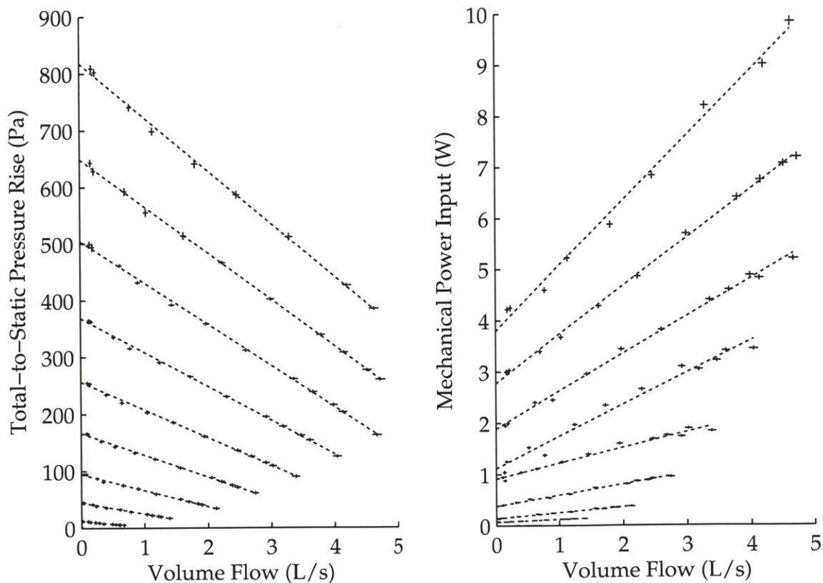
Figure 4-9: The fan and power curves were found to be well described by linear fits; this experimental data is for Fan 5 (15 blades, 90^\circ exit angle, b_b = 1.6\text{ mm} , b_g = 2.6\text{ mm} ). The curves shift away from the origin with increasing rotational speed. Fan and power curves for 1–9 krpm are shown in 1 krpm increments.
