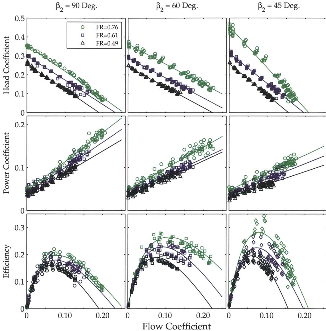
Figure 4-12: Fan performance curves for 3 15-bladed impeller geometries (Fan 8, \beta_2 = 90^\circ ; Fan 12, \beta_2 = 60^\circ ; and Fan 13, \beta_2 = 45^\circ ) are shown, with 3 fill ratios shown in each plot. As in Fig. 4-11, the fan performance curve improves in both the \psi_{ts} and \phi intercepts as the fill ratio increases. As the exit angle is reduced, the blades become more backswept; as the Euler turbomachinery equation predicts, the maximum flow coefficient decreases and the maximum head coefficient increases. The maximum efficiency increases with decreases in the blade angle.
