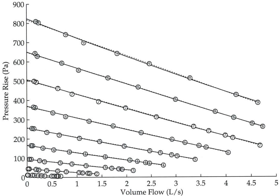
Figure 2-16: An example of some raw fan curves measured with the circular stator apparatus. These data were taken on a 15-blade fan with b_b = 1.6 mm, b_g = 2.6 mm, d_1 = 40 mm, d_2 = 100 mm, and 60^\circ exit angle. The numbers in each marker indicate the rotational speed in krpm. The solid lines are parabolic fits to each rotational speed; the dashed lines are linear fits. Most of the experiments were satisfactorily represented by a linear fit.
