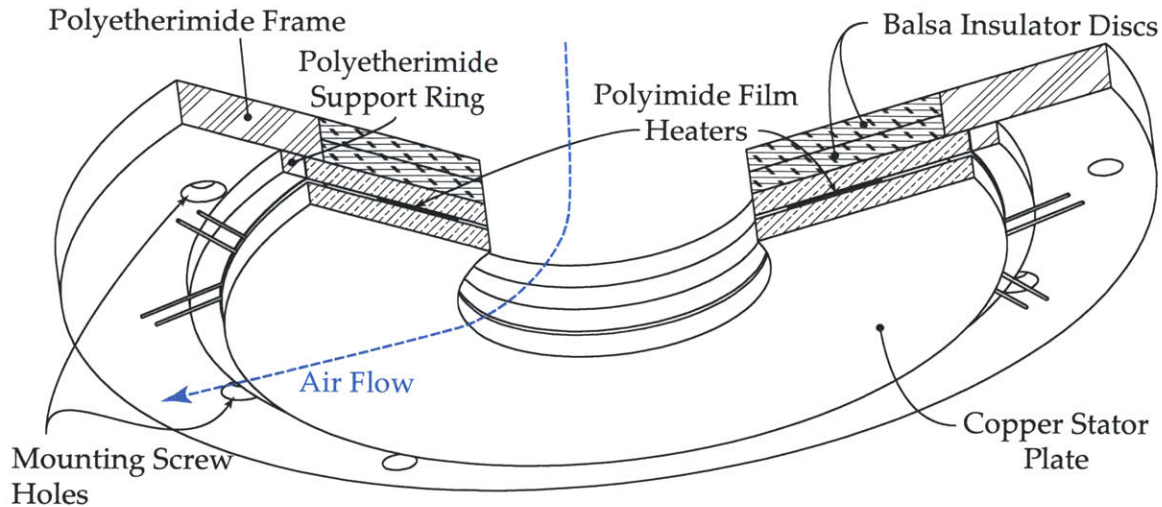
Figure 2-17: The circular stator apparatus used a sandwich structure comprised of copper plates with polyimide heaters to measure the average heat transfer coefficient. The copper plates encased the heaters and a copper foil spacer and were glued together with silver-filled, thermally conductive epoxy. A polyetherimide support structure was then adhered with conventional epoxy to the copper plates; this allowed the heater assembly to mount to the bottom of the plenum. Balsa insulator discs minimized the heat loss from the copper opposite the air-flow. This is a view of the upper stator plate from below, with a cutaway to show the internal structure of the assembly.
