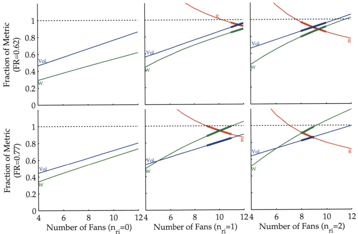
Figure 5-13: The flow circuit model was run for 4–12 layers with Fan 12 (with b_b = 1.5\text{mm} ) rotating at 6 krpm. The thermal resistance (“R”), overall device volume (“Vol.”), and mechanical power input (“W”) were calculated at each operating point, and were normalized to the DARPA metrics in Table 1.1 (viz. R = 0.05\text{K/W} , \text{Vol.} = 1\text{ L} , \dot{W} = 33\text{ W} ). The fill ratio (FR) was 0.62 in the top 3 plots and 0.77 in the bottom 3 plots; the number of radial inlets ( n_{ri} ) was varied 0, 1 and 2 for the left, middle, and right plots. In these plots, a design that meets the DARPA metrics must have all 3 quantities below the dashed line for a given number of fans . These valid design points are shown with thicker lines.
