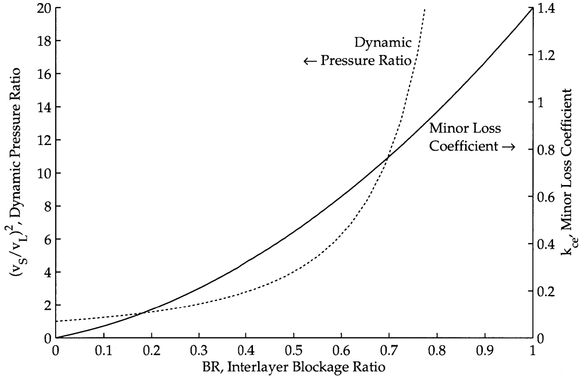
Figure 5-9: The minor loss coefficient for the contraction-expansion in the interlayer flow increases parabolically with the blockage ratio. However, the dynamic pressure ratio between the open (large) area and the obstructed (small) area diverges as the blockage ratio approaches 1, leading to significant total pressure loss in the interlayer flow. v_S and v_L are the velocities in the small and large areas, respectively.
