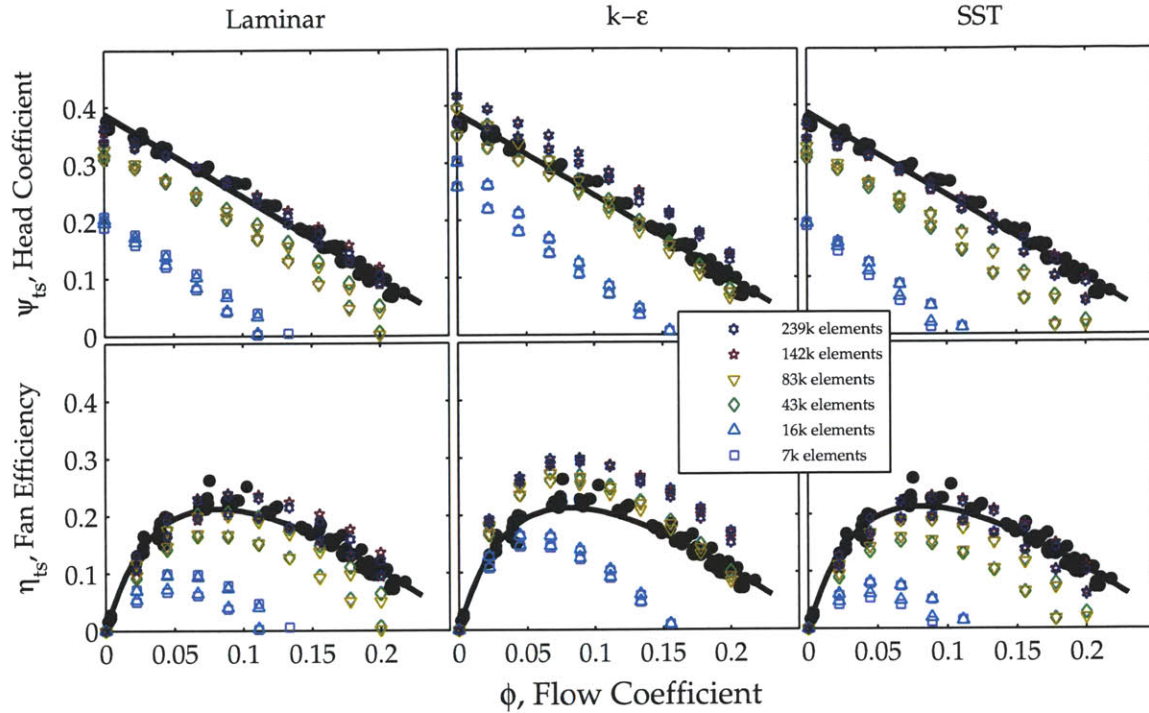
Figure 3-3: Three turbulence models (laminar, k - \epsilon , and SST) with various mesh sizes were compared to some experimental data (solid black circles with a best-fit line) for Fan 5, with a blade breadth of b_b = 1.6\text{mm} and a gap breadth of b_g = 2.0\text{mm} . The shape and color of the markers (as indicated in the legend) corresponds to the number of elements; as the number of elements increased, the CFD models more closely approximated the experimental data (with the exception of the k - \epsilon model, which slightly overpredicted the fan curve and the efficiency). Overall, the fan behavior was captured by all three of the turbulence models, as long as the number of elements in the mesh was sufficiently high.
