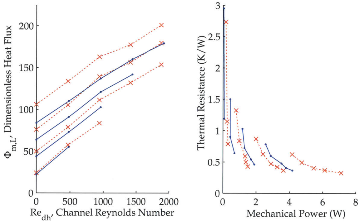
Figure 4-24: The addition of wipers to an impeller results in a slight change in the dimensionless heat transfer characteristics. In the figure, the blue dots indicate a conventional impeller (Fan 1, b_b = 1.5 mm, b_g = 3.6 mm) and the red x's indicate a wiper impeller (Fan 1, b_b = 1.5 mm, b_w = 2.5 mm, and b_g = 3.6 mm). The slight improvement in the dimensionless heat flux makes sense in light of the previous heat transfer observations: the effective aspect ratio of the wiper impeller increases (the addition of the wiper increases the effective breadth of the impeller), and Eq. 4.19 suggests an increase in the proportionality of \Phi_{m,L} with an increase in AR , explaining the wider spacing between the lines of constant rotational speed. The thermal resistance for the same mechanical power appears to be slightly improved with the wiper impeller.
