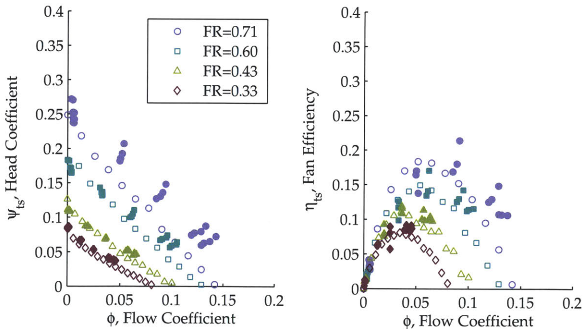
Figure 3-6: A CFD model of Fan 1 ( d_2 = 100\text{mm} , d_1 = 40\text{mm} , b_b = 1.5\text{mm} , FR = [0.33, 0.43, 0.60, 0.71] ) that used the SST turbulence model computed the trends in the fan and efficiency curves. The solid markers indicate experimental data; the hollow markers represent the CFD results for the corresponding geometry. The marker type indicates the fill ratio (see legend).
