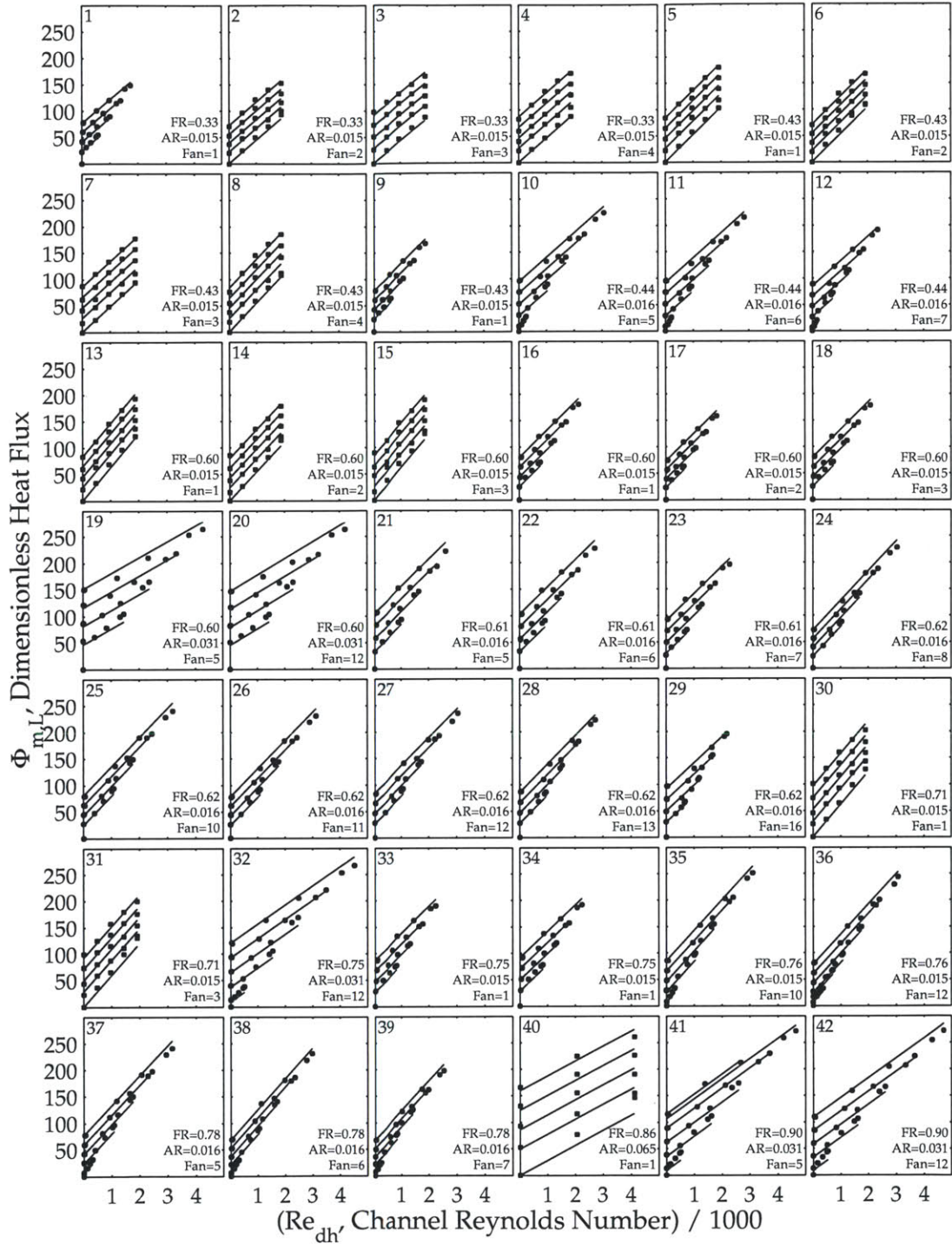
Figure 4-5: The similarity in the trends and magnitude of the dimensionless heat flux over 42 sets of experimental data shows its relative insensitivity to the impeller geometry (except the aspect ratio, which seemed to have a small effect). The dimensionless heat flux was observed to be a function of the channel Reynolds number ( Re_{dh} ) and the rotational Reynolds number ( Re_{\omega} ). The square and circular stator apparatus tests are indicated by square and circle shaped markers, respectively. First, the heat transfer appears to be insensitive to the local meridional velocity, because points with substantially different gap spacings have similar dimensionless heat fluxes at the same Re_{dh} (i.e. \dot{Q} depends only on \dot{m} and not on the local meridional velocity). The implication is that, in contrast to pipe flow, the average through-flow velocity is not the dominant contributor to the turbulence and heat transfer. Second, the channel Reynolds numbers are quite low and fall solidly within the laminar range; however, the observed heat transfer coefficients are higher than the laminar flow estimates.
