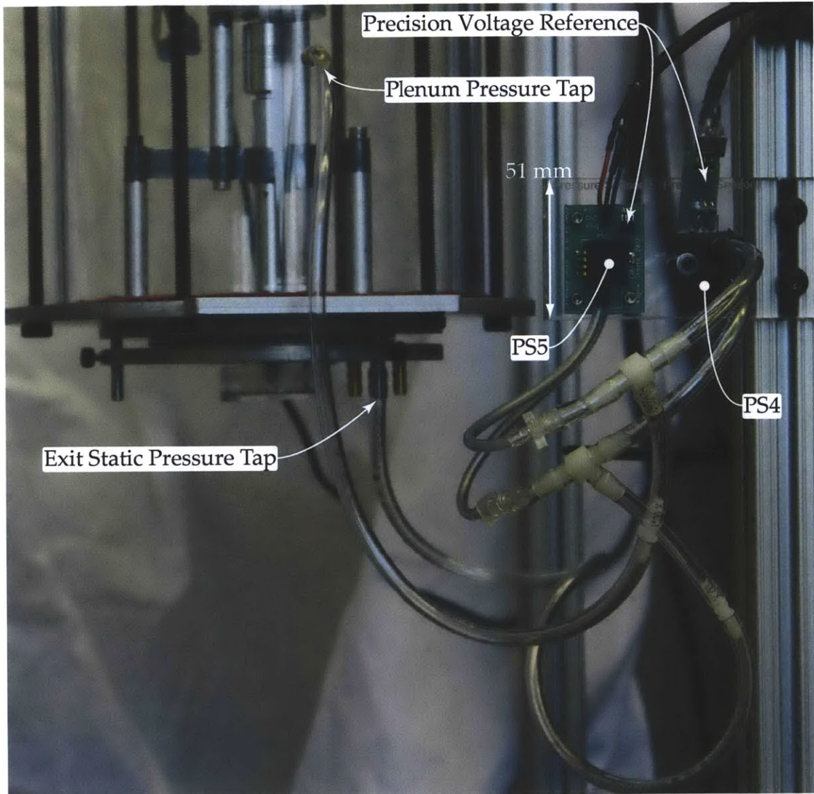
Figure 2-11: Pressure sensors 4 and 5, used in the circular stator apparatus, measured the pressure difference between the plenum and the exit of the fan.
