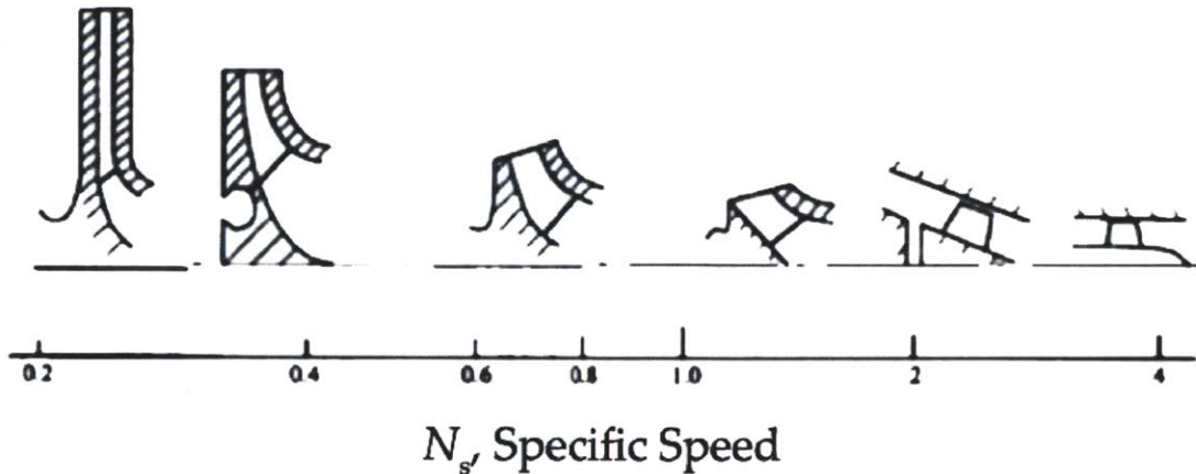
Figure 1-10: The specific speed is a dimensionless performance parameter that describes turbomachinery and serves as a design guideline for selection of optimal topology. For a fan in the diameter range of the PHUMP, and a reasonable rotational speed ( \sim 5000 rpm), the specific speed is about 0.4. This specific speed suggests that a centrifugal fan would yield the best results (Figure from [48]).
