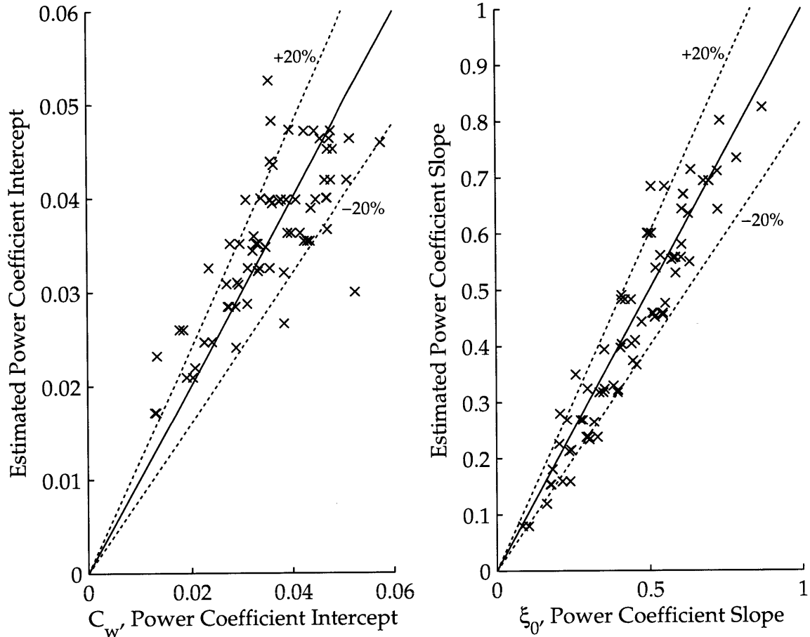
Figure 4-15: The power curve parameters \xi_0 and C_w were correlated to the fan geometry using Eq. 4.36; the estimates produced using Eq. 4.36 can be seen agree to within 20% for most of the experiments. Lines of \pm 20\% are shown as dashed lines; the solid line indicates a perfect estimate.
