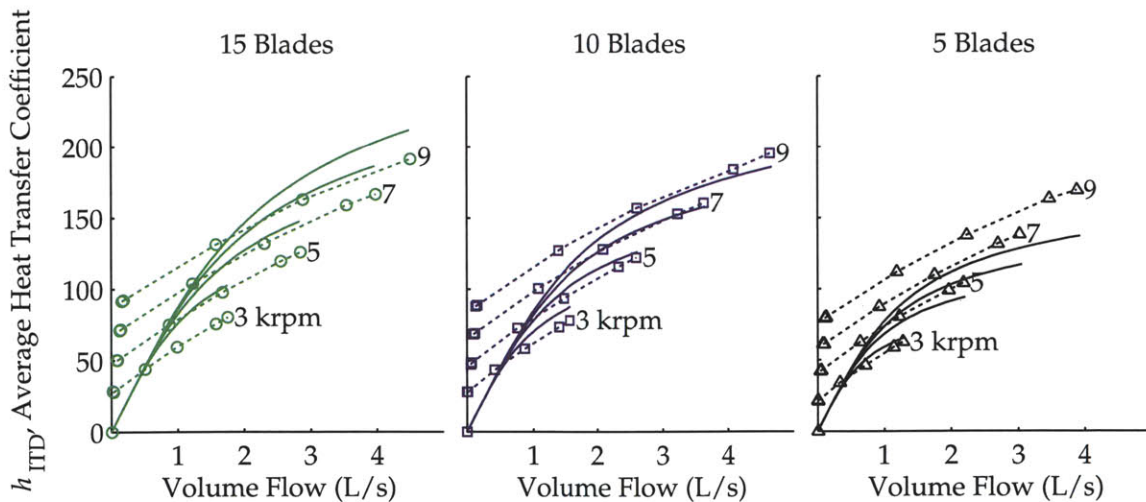
Figure 4-3: The heat transfer in three impellers with various numbers of blades (15, 10 and 5) was predicted to be significantly different by the surface renewal theory; however, experimental data only showed a small difference in the heat transfer coefficient at a fixed volume flow through the fan. In these plots, the experimental data points with the same rotational speed are connected with a dashed line; the solid lines are the surface renewal theory estimates. The main effect of increasing the number of blades to improve the fan performance (the 5-blade impeller cannot pump as much air as the 10- or 15-blade impeller at the same rotational speed).
