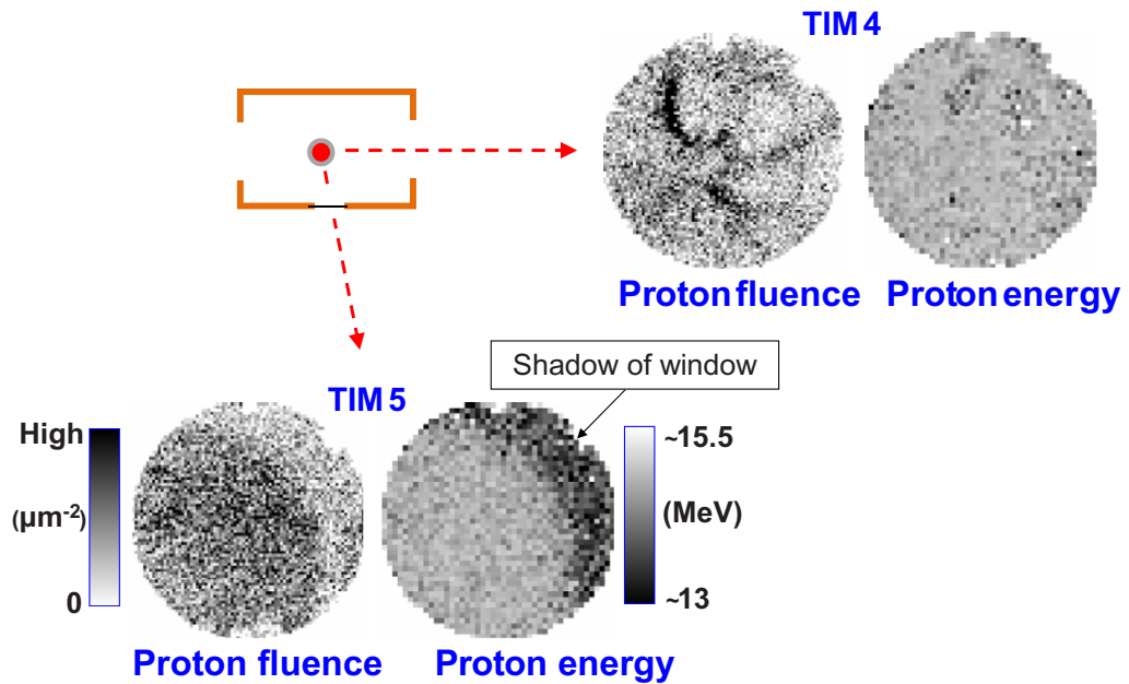
Figure 9. Images showing fluence and mean energy, respectively, of self-emitted \text{D}^3\text{He} protons as a function of position in detectors viewing the capsule from two different directions in OMEGA shot 54741. Compared with the self-emission image made in the equatorial direction, the one recorded through the LEH shows very nonuniform proton fluence, but it also shows no significant correlated nonuniformities in energy. This suggests that the observed fluence variation has been largely caused by fields near the LEHs and not by proton scattering in the plasma, because Coulomb interactions are always accompanied by energy loss [26].
