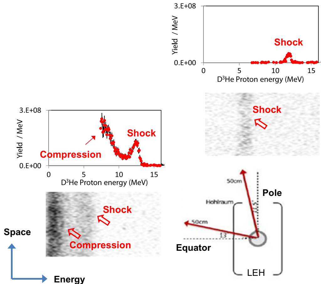
Figure 3. Typical images of proton fluence as a function of energy and spatial direction of self-emitted protons generated from the fusion reaction of D and ^3\text{He} in an indirect-drive, NIC ICF implosion (shot N101211). Data were acquired simultaneously at two different angles. The high-energy peak in each spectrum is associated with shock-flash burn, and the low-energy part seen in the equatorial direction results from compression burn. (Note that the equatorial spectrum above has been corrected for the extra energy lost by the protons while passing through the hohlraum wall.)
