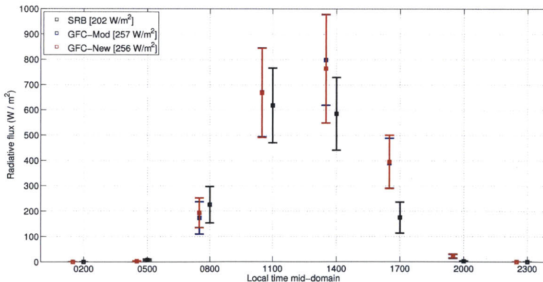
Figure 4-14. Diurnal cycle of insolation (in W\ m^{-2} ) averaged over land for period 1998-2001, from SRB observations and simulations using Grell Fritsch-Chappell scheme with modifications from Chapter 3 (GFC-Mod), and with new convective cloud cover (GFC-New). Square symbol indicates the mean value; error bars indicate +/- 1 standard deviation.
