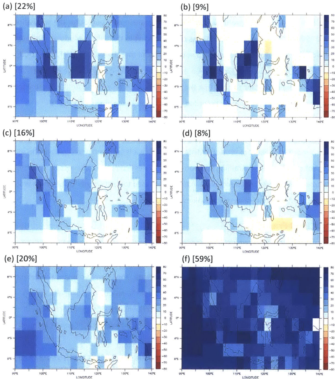
Figure 4-5. Average low cloud fraction for 1998-2001: simulation minus ISCCP data for (a) GFC (default model), (b) EMAN (default model), (c) GFC-Mod (as in Chapter 3), (d) EMAN-Mod (as in Chapter 3), (e) GFC-New (with new FC_{cnv} ) and (f) EMAN-New (with new FC_{cnv} ). Domain-averaged error (model – ISCCP cloud fraction) is shown in parentheses. Color bar indicates fractional coverage of grid cell.
