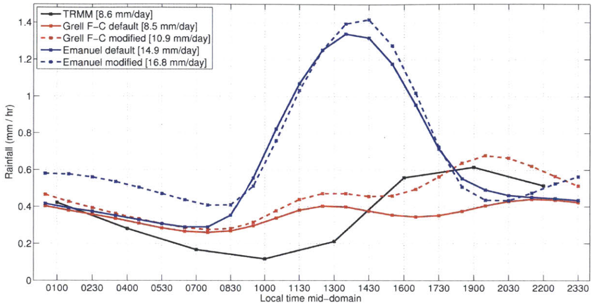
Figure 3-17. Diurnal cycle of rainfall (in \text{mm hr}^{-1} ) averaged over land for period 1998-2001, comparing default simulations to the modified version of the model.
