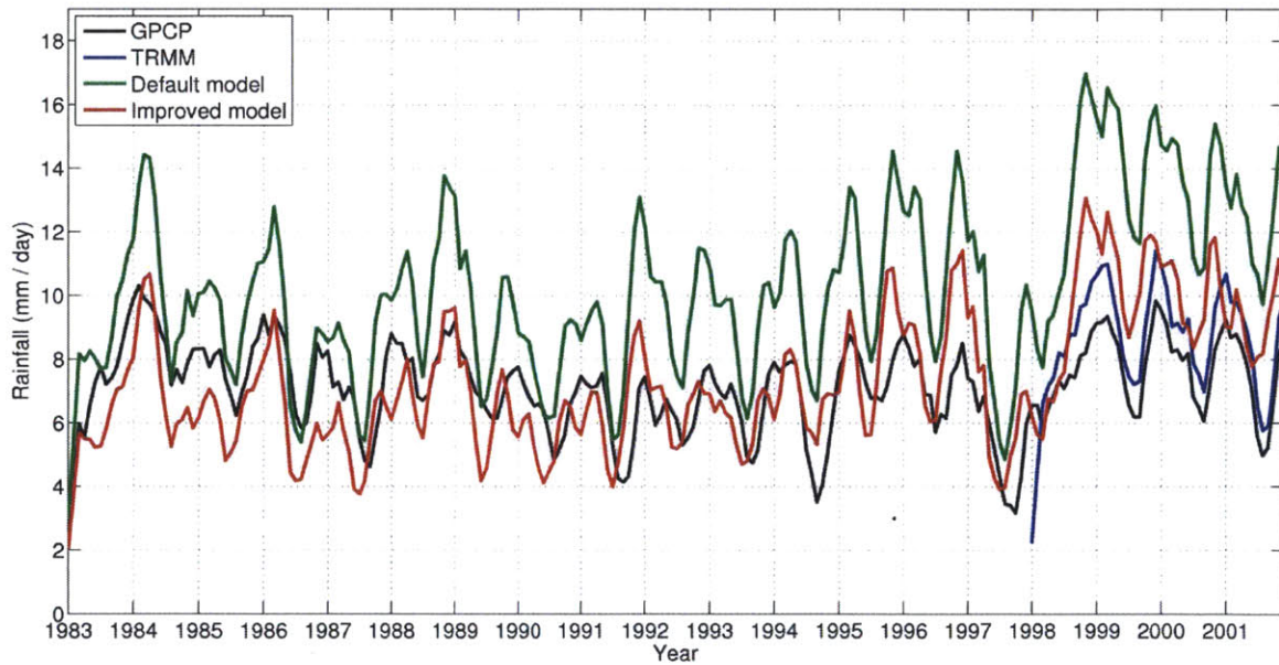
Figure 7-5. 3-month moving average of rainfall (mm day -1 ) over land for period 1983-2001, comparing GPCP (black), TRMM (blue; for period 1998-2001), default version of RegCM3-IBIS using Emanuel scheme (green) and improved version of the model (red).
