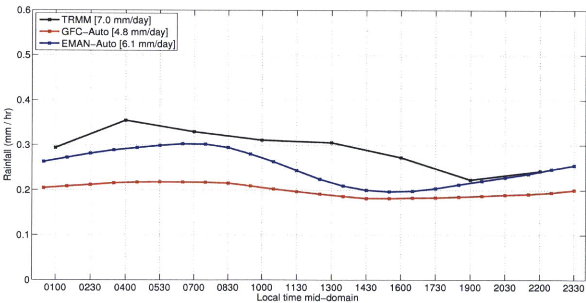
Figure 5-18. Diurnal cycle of rainfall (in mm hr -1 ) averaged over ocean for period 1998-2001 for TRMM and the new simulations with all modifications (to PBL region, convective cloud fraction and autoconversion, '-Auto').
