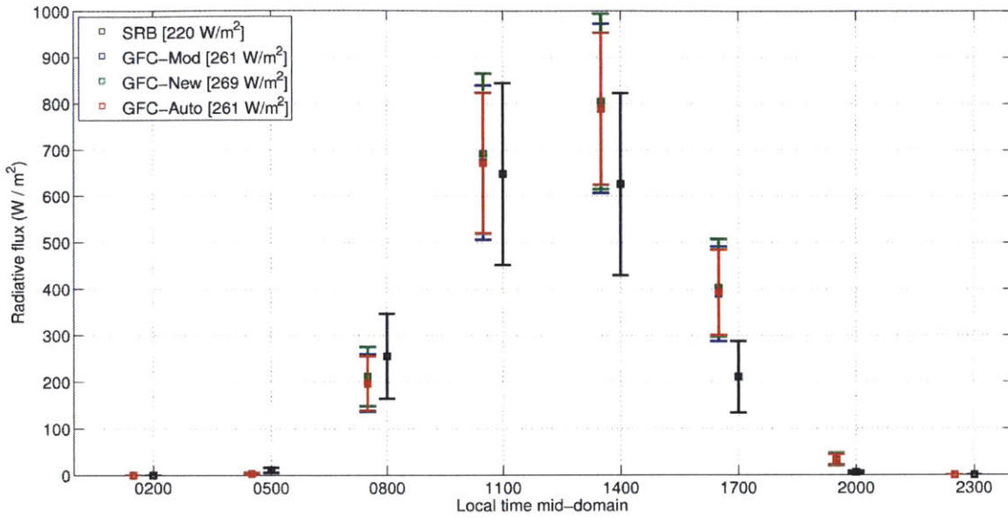
Figure 5-13. Diurnal cycle of incoming solar radiation (in W/m^2 ) averaged over ocean for period 1998-2001, from SRB observations and simulations using Grell Fritsch-Chappell scheme with modifications from Chapter 3 ('GFC-Mod'), those modifications plus the new convective cloud fraction and CLW from Chapter 4 ('GFC-New') and new autoconversion formulation combined with all other changes ('GFC-Auto'). Square symbol indicates mean value; error bars indicate +/- 1 standard deviation.
