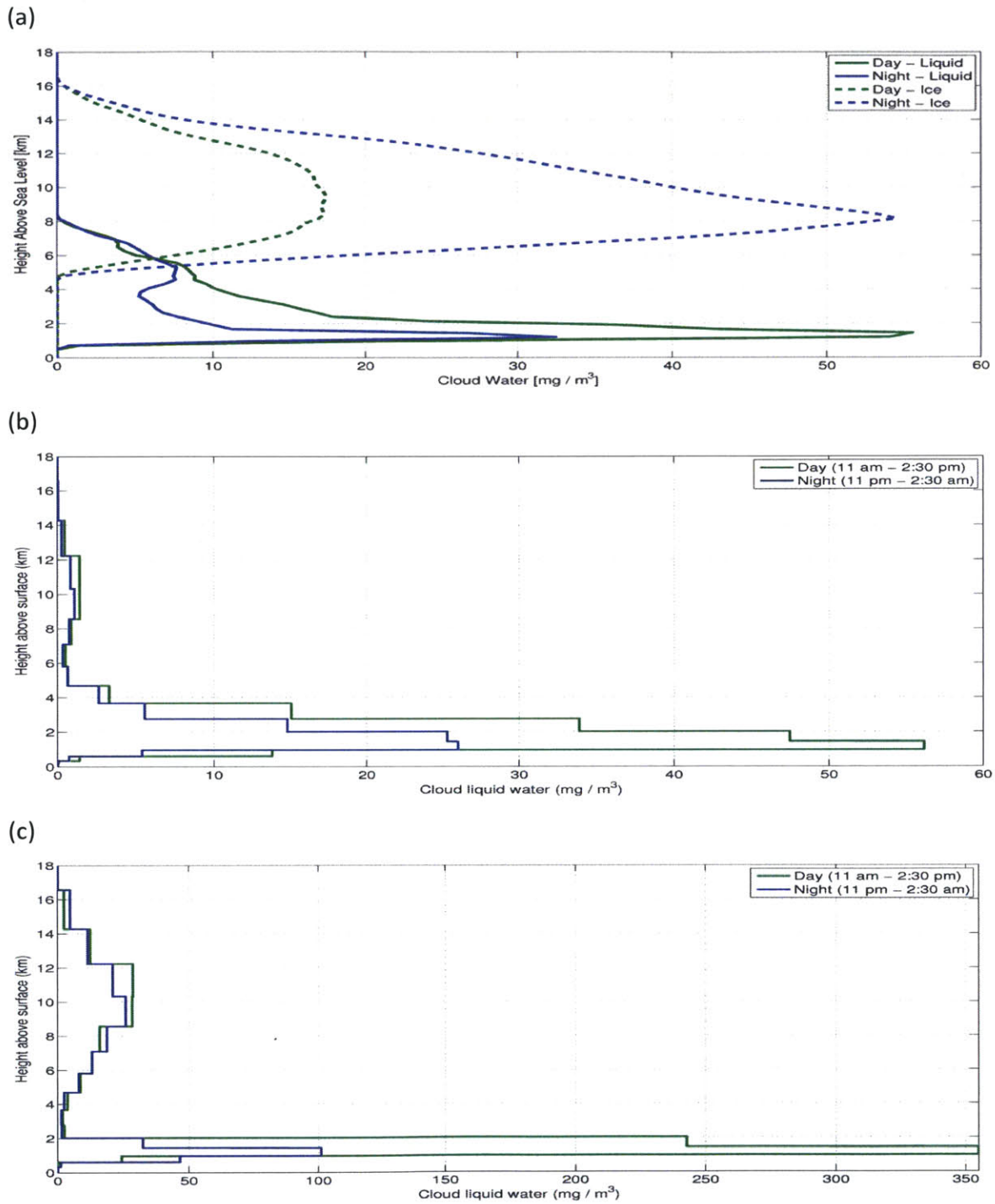
Figure 5-9. Average cloud liquid water (in \text{mg m}^{-3} ) profile over central Borneo from (a) CloudSat for period 2006-2011, (b) simulation using Grell Fritsch-Chappell scheme with new convective cloud cover for period 1998-2001, (c) as for middle but using Emanuel scheme (note the change in x-axis).
