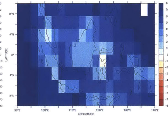
Figure 4-6. Average middle cloud fraction for 1998-2001: simulation minus ISCCP data for (a) GFC (default model), (b) EMAN (default model), (c) GFC-Mod (as in Chapter 3), (d) EMAN-Mod (as in Chapter 3), (e) GFC-New (with new FC_{cnv} ) and (f) EMAN-New (with new FC_{cnv} ). Domain-averaged error (model – ISCCP cloud fraction) is shown in parentheses. Color bar indicates fractional coverage of grid cell.
