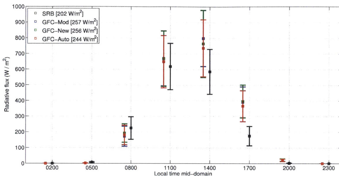
Figure 5-11. Diurnal cycle of incoming solar radiation (in W\ m^{-2} ) averaged over land for period 1998-2001, from SRB observations and simulations using Grell Fritsch-Chappell scheme with modifications from Chapter 3 ('GFC-Mod'), those modifications plus the new convective cloud fraction and CLW from Chapter 4 ('GFC-New') and new autoconversion formulation combined with all other changes ('GFC-Auto'). Square symbol indicates mean value; error bars indicate +/- 1 standard deviation.
