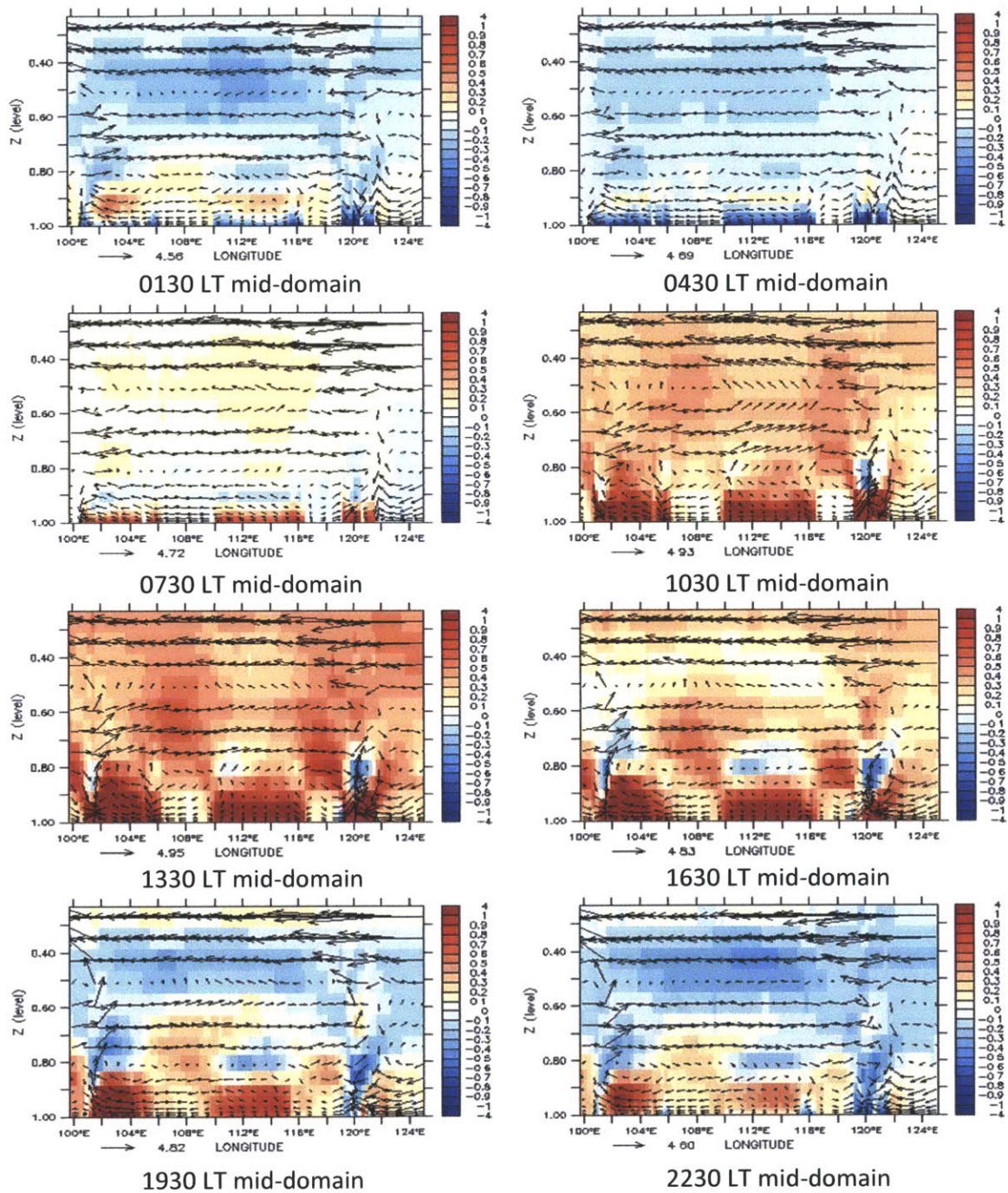
Figure 6-18. Diurnal cycle averaged over the period 1998-2001 of temperature anomaly ( ^{\circ}\text{C} , see color bar) with zonal and vertical winds ( \text{m s}^{-1} , with vertical wind component amplified 10 times) along 2^{\circ}\text{S} from simulation using Emanuel scheme with new version of the model. Vertical axis shows sigma levels up to about 350 mb. Local time for the center of the domain is given at the bottom of each panel. Arrows underneath each panel indicate the maximum wind strength.
