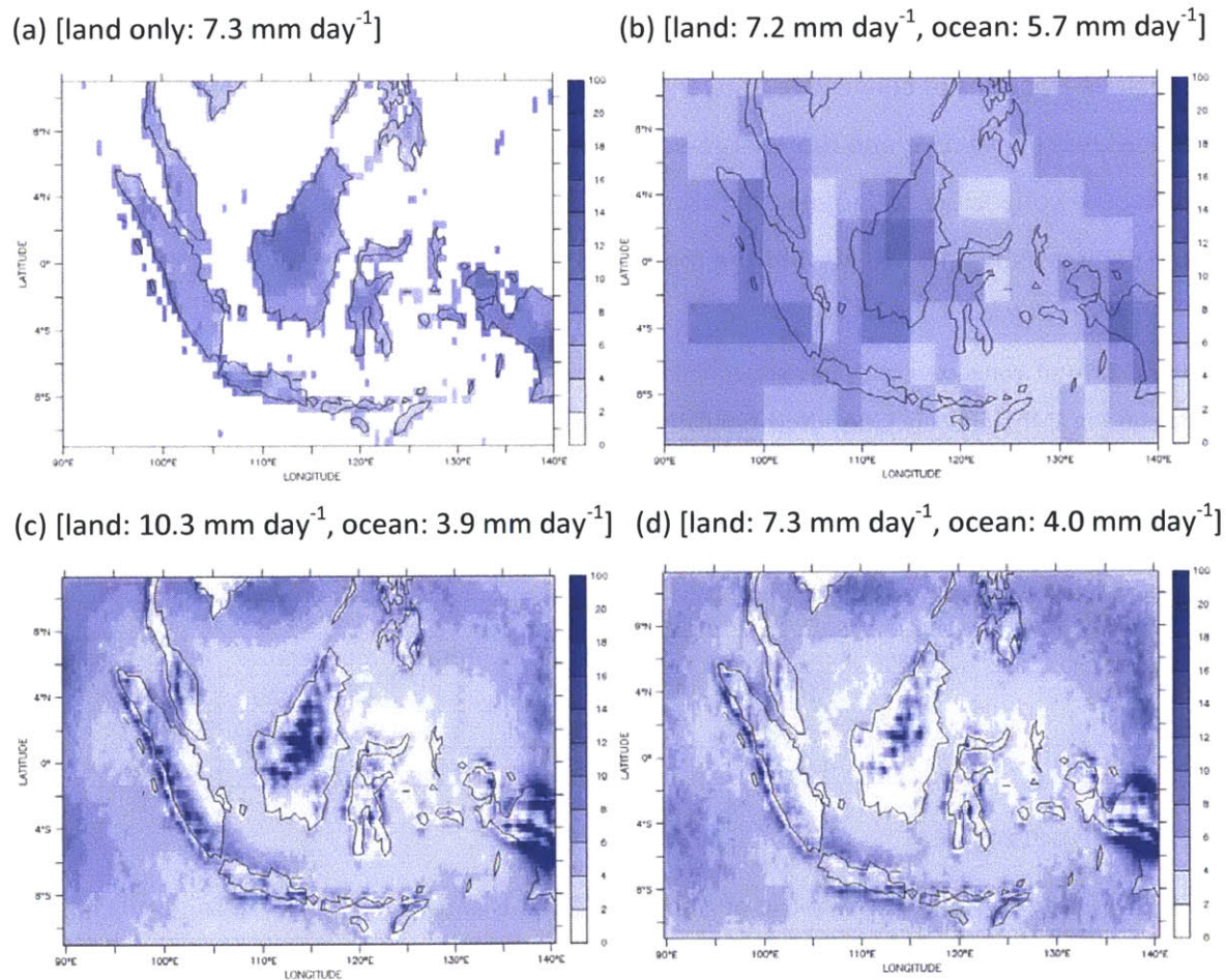
Figure 7-3. Average rainfall (in mm day -1 ) for period 1983-2001, from (a) CRU TS3.0, (b) GPCP V2.2, (c) EMAN-Def (default) simulation, (d) EMAN-New simulation (incorporating all modifications presented in Chapters 3 to 5). Domain-average values are given in parentheses.
