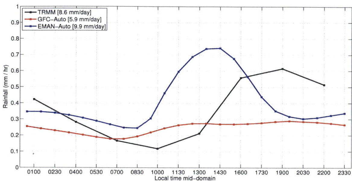
Figure 5-17. Diurnal cycle of rainfall (in mm hr -1 ) averaged over land for period 1998-2001 for TRMM and the new simulations with all modifications (to PBL region, convective cloud fraction and autoconversion, '-Auto').
