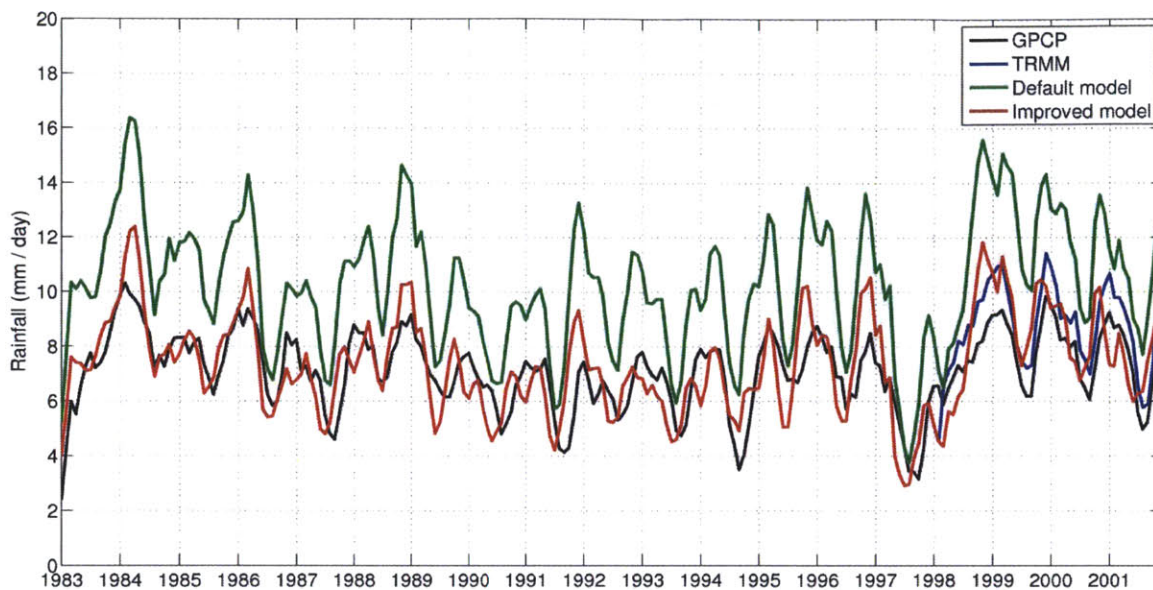
Figure 7-7. 3-month moving average of rainfall (mm day -1 ) over land for period 1983-2001, comparing GPCP (black), TRMM (blue; for period 1998-2001), default version of RegCM3-IBIS using Emanuel scheme (green) and improved version of the model (red). A positive trend in the simulated rainfall has been removed.
