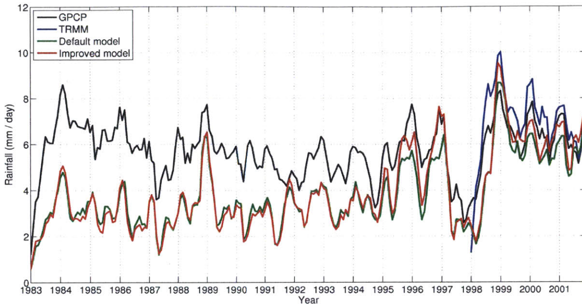
Figure 7-6. 3-month moving average of rainfall ( \text{mm day}^{-1} ) over ocean for period 1983-2001, comparing GPCP (black), TRMM (blue; for period 1998-2001), default version of RegCM3-IBIS using Emanuel scheme (green) and improved version of the model (red).
