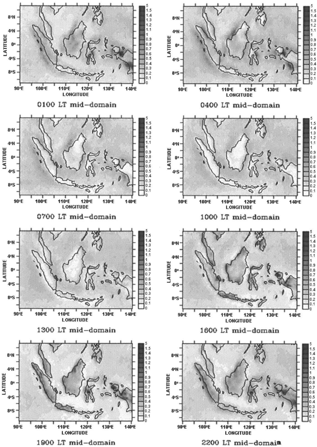
Figure 2-6. Diurnal cycle of rainfall from TRMM. Local time for the center of the domain is given at the bottom of each panel. Each panel represents the average rainfall rate in \text{mm hr}^{-1} (shown by the color scale bar) over a 3-hour period centered at the given time, averaged over the period 1998-2001.
