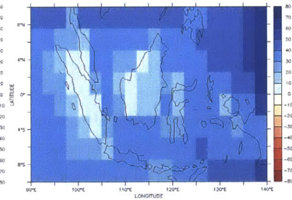
Figure 5-4. Average high cloud fraction for 1998-2001: simulation minus ISCCP data for (a) GFC-Mod, (b) EMAN-Mod, (c) GFC-New, (d) EMAN-New, (e) GFC-Auto and (f) EMAN-Auto. Domain-averaged error (model – ISCCP cloud fraction) is shown in parentheses. Color bar indicates fractional coverage of grid cell.
