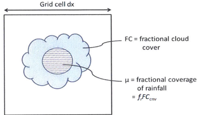
Figure 5-1. Relationship between fractional cloud cover, FC, and fractional coverage of rainfall, \mu .
