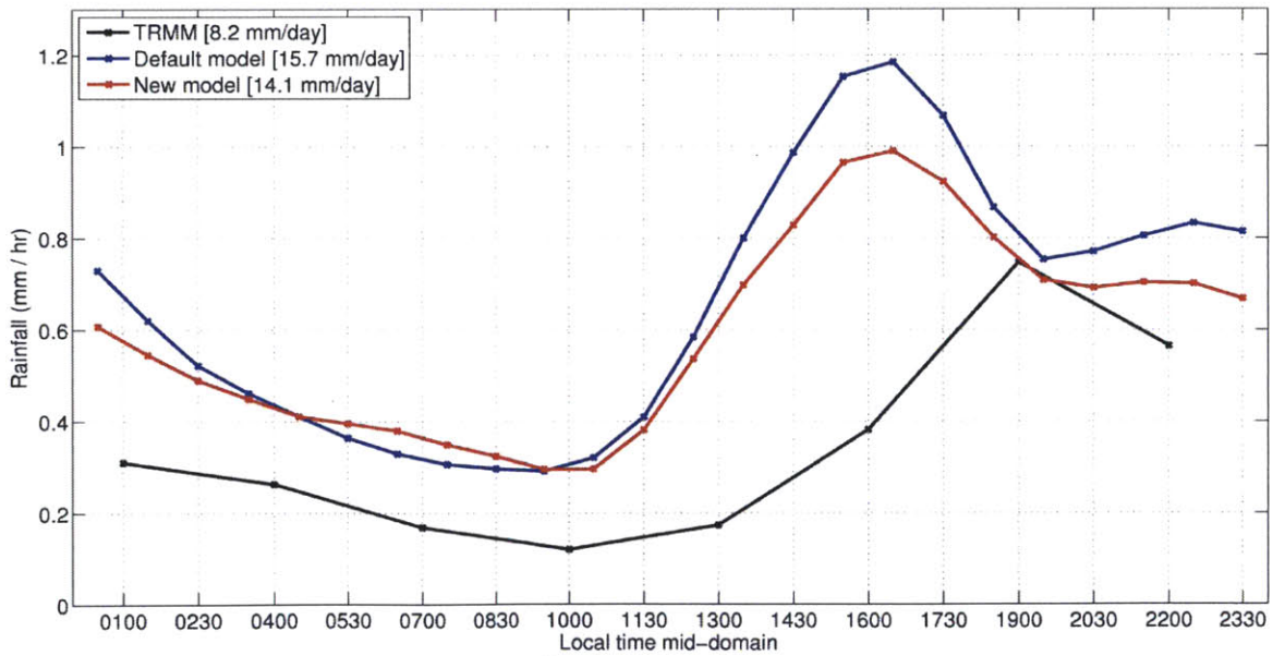
Figure 6-13. Diurnal cycle of rainfall (in \text{mm hr}^{-1} ) averaged over northern Sumatra sub-region for period 1998-2001 for TRMM and simulations using Emanuel scheme with default version of the model and version with all modifications (to PBL region, convective cloud fraction and autoconversion). Mean values are given in parentheses.
