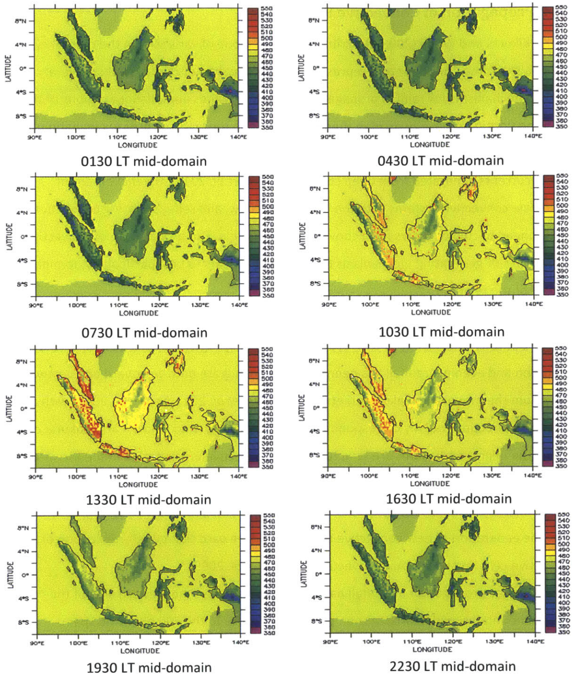
Figure 6-20. Diurnal cycle averaged over the period 1998-2001 of longwave radiation (in W m^{-2} ) away from surface (i.e. radiative cooling) from simulation using Emanuel scheme with new version of the model. Local time for the center of the domain is given at the bottom of each panel.
