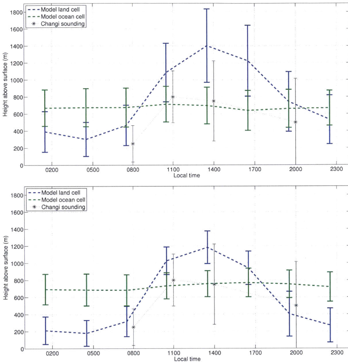
Figure 3-11. Diurnal PBL height (in m) over or near Singapore, simulated by the (top) Grell Fritsch-Chappell and (bottom) Emanuel convection schemes using either a land (blue) or ocean (green) grid cell to represent Singapore, compared to the PBL height estimated from the Changi soundings (black stars; dotted lines are shown to interpolate between the measurement times). The vertical bars signify one standard deviation of each sample set and illustrate the variability in the simulated and observed PBL height.
