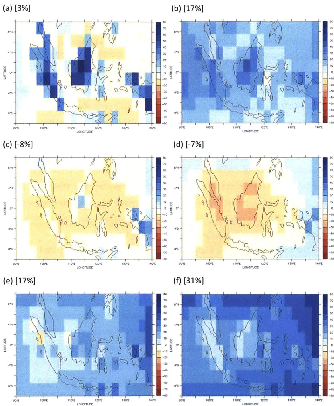
Figure 7-2. Average cloud fraction over 1983-2001: EMAN-Def simulation minus ISCCP data for (a) low, (c) middle and (e) high clouds, and EMAN-New simulation minus ISCCP data for (b) low, (d) middle and (f) high clouds. Domain-averaged error (model – ISCCP cloud fraction) is shown in parentheses. Color bar indicates fractional coverage of grid cell.
