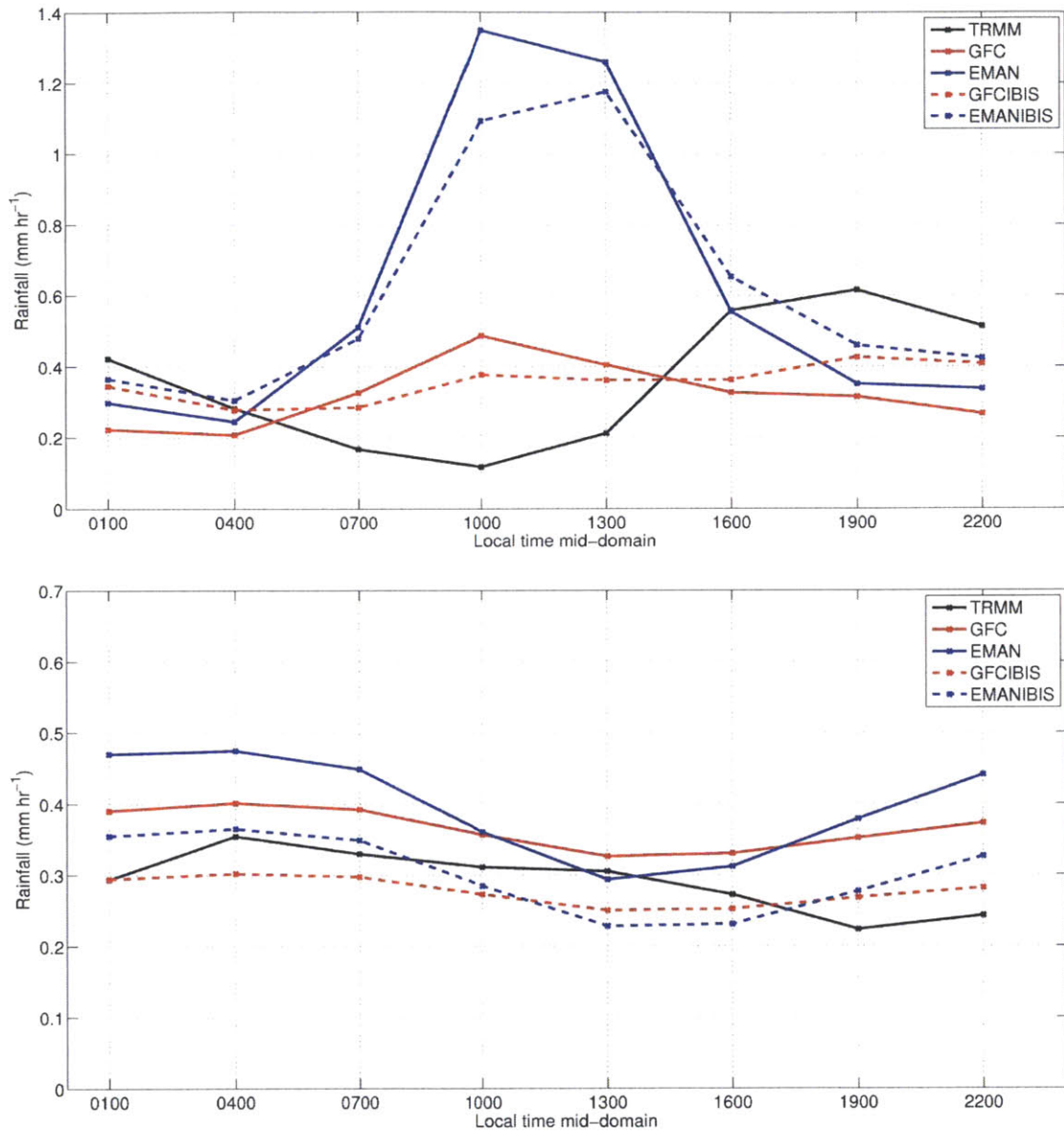
Figure 2-11. Average diurnal cycle of rainfall (in \text{mm hr}^{-1} ) over period 1998-2001: comparison between TRMM and the GFC (red) and EMAN (blue) simulations using BATS1e (solid lines) and IBIS (dashed lines). (a) Upper panel shows average of land cells within the domain; (b) lower panel shows average of ocean cells.
