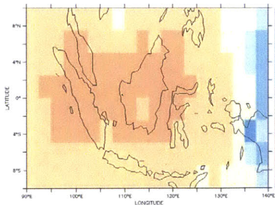
Figure 5-3. Average middle cloud fraction for 1998-2001: simulation minus ISCCP data for (a) GFC-Mod, (b) EMAN-Mod, (c) GFC-New, (d) EMAN-New, (e) GFC-Auto and (f) EMAN-Auto. Domain-averaged error (model – ISCCP cloud fraction) is shown in parentheses. Color bar indicates fractional coverage of grid cell.
