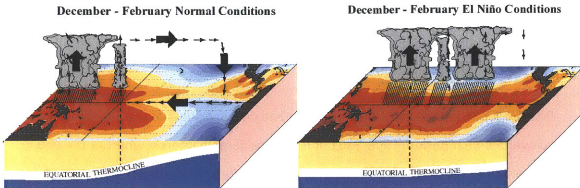
Figure 7-1. Schematic showing the typical circulation and temperature patterns over the Pacific Ocean under (left) average and (right) El Niño conditions during the northern winter. El Niño episodes feature reduced easterly winds across the Pacific in the lower atmosphere and reduced westerly winds in the upper atmosphere. These conditions reflect a reduced strength of the equatorial Walker Circulation. (From NOAA Climate Prediction Center, Accessed 22 October 2012.
