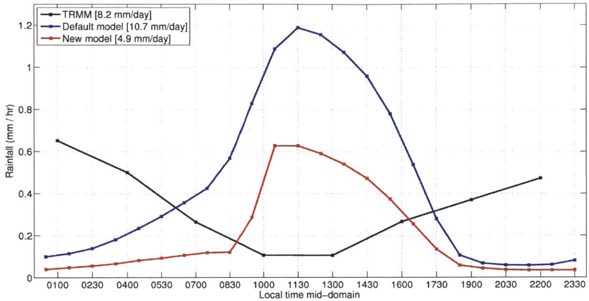
Figure 6-12. Diurnal cycle of rainfall (in \text{mm hr}^{-1} ) averaged over lowland Borneo sub-region for period 1998-2001 for TRMM and simulations using Emanuel scheme with default version of the model and version with all modifications (to PBL region, convective cloud fraction and autoconversion). Mean values are given in parentheses.
