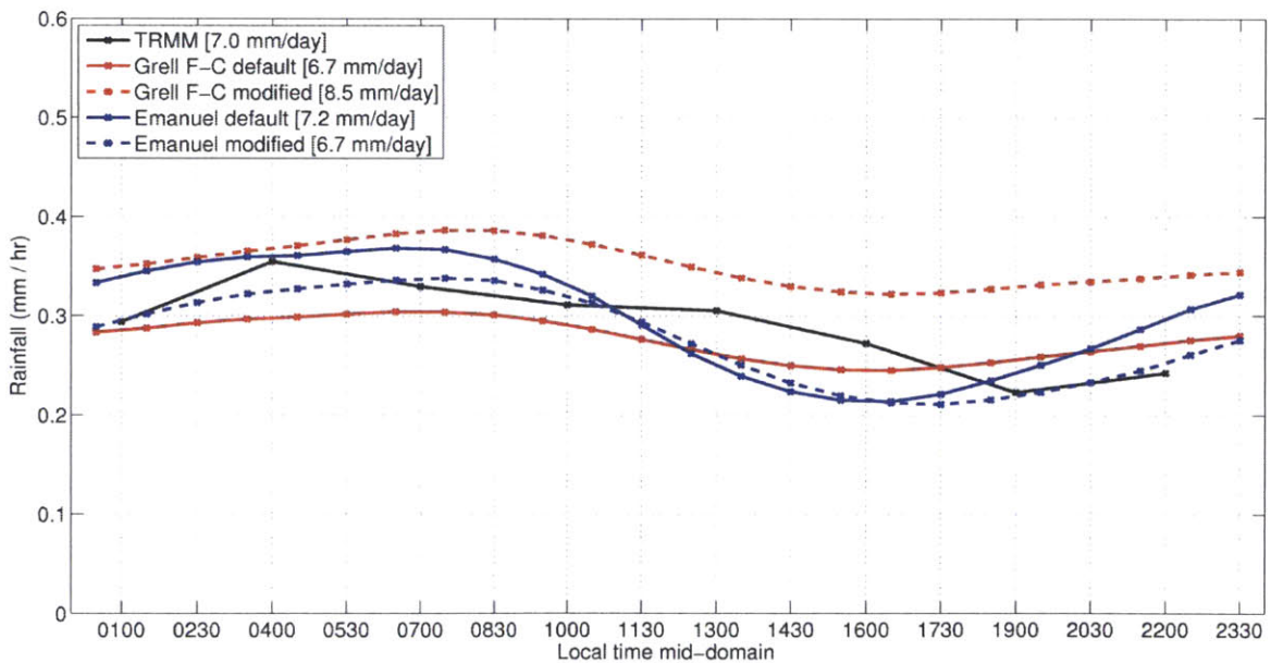
Figure 3-18. Diurnal cycle of rainfall (in \text{mm hr}^{-1} ) averaged over ocean for period 1998-2001, comparing default simulations to the modified version of the model.
