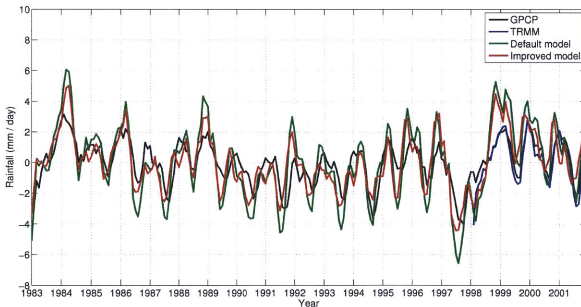
Figure 7-8. Rainfall (mm day -1 ) over land for period 1983-2001, showing the difference between the 3-month moving average and the mean rainfall for GPCP (black), TRMM (blue; for period 1998-2001), default version of RegCM3-IBIS using Emanuel scheme (green) and improved version of the model (red). A positive trend in the simulated rainfall has been removed.
