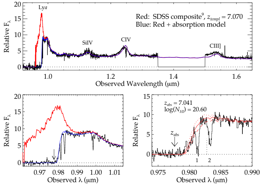
Figure 1: FIRE spectrum of ULAS J1120+0641, alongside our estimate of the intrinsic source spectrum and a composite model including foreground absorption. The unabsorbed continuum is shown in red, and the blue curve includes the absorption. The continuum is constructed from a composite of quasars in the Sloan Digital Sky Survey 14,16 . C IV absorption intrinsic to the quasar host galaxy is seen to the red of the labeled CIV emission peak. However, the C IV emission line is anomalously blueshifted 6 in ULAS J1120, so we compute the redshift distance between the absorber and quasar host using its MgII 6 or [C II] (ref 25) redshift. Bottom Left: The Lyman alpha region of the spectrum with unabsorbed continuum model (red) and absorbed continuum (blue). The vertical arrow marks the location of Ly \alpha absorption at z = 7.04 . Bottom right: Detail of the damping wing with HI absorption fit. The quasar's emission redshift 25 (7.0842) is indicated with the vertical dashed line. Two additional optically thin Ly \alpha absorbers (labeled 1 and 2) are apparent in the quasar's near zone at z = 7.0721 \pm 0.0001 and z = 7.0855 \pm 0.0001 ( \Delta v = -424, +161 km / s from the host, see Supplementary Information). These data have not been continuum normalized, so a slight downward slope is visible toward redder wavelengths.
