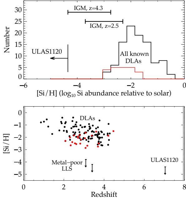
Figure 3: Comparison of z = 7.04 abundance measurement in ULAS J1120 with existing values from the literature. The top panel displays a histogram of the Silicon abundance for known DLAs 11,12,21 , while the bottom panel shows the same systems at their respective redshifts. The top panel includes the \pm 1\sigma abundance ranges for intergalactic absorption systems 22,23 at redshift 2.5 and 4.3. The bottom panel also shows the locations of two recently reported metal-poor Lyman limit QSO absorbers 4 at z \sim 3 . DLAs at lower redshift exhibit -2.5 < [\text{Si}/\text{H}] < -0.5 , 11 with the lowest previously known system having [\text{Si}/\text{H}] = -2.75 . 13 Surveys designed expressly to uncover metal-poor DLAs (shown with red histogram and points) find -2.86 < [\text{Si}/\text{H}] < -1.5 . 12
