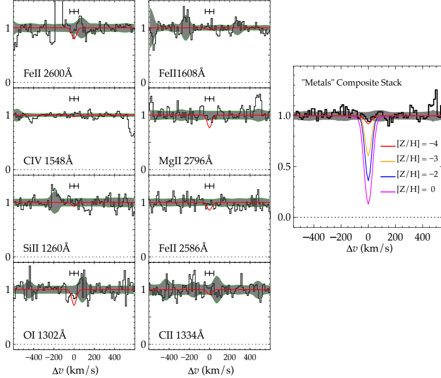
Figure 2: Continuum-normalized spectral regions where key heavy element transitions would fall at z=7.041 if the absorber were typical of a low redshift DLA. 1\sigma error contours are shaded grey, and the extraction aperture is indicated with horizontal bars. A Voigt profile with b = 10 km/s and N set by our column density upper limit is shown in red for each panel. Velocity offsets are relative to the rest frame of the HI absorber. Right Panel: Composite stack of all heavy element transitions, generated using an inverse-variance weighted mean and solar relative abundances. Each transition is scaled to the cross section and relative abundance of O I. Overlaid curves show the predicted profiles for varying metallicity levels. The stack shows no statistically significant absorption, though there is a fluctuation at the 1\sigma level, corresponding to an effective [O/H] < -4 .
