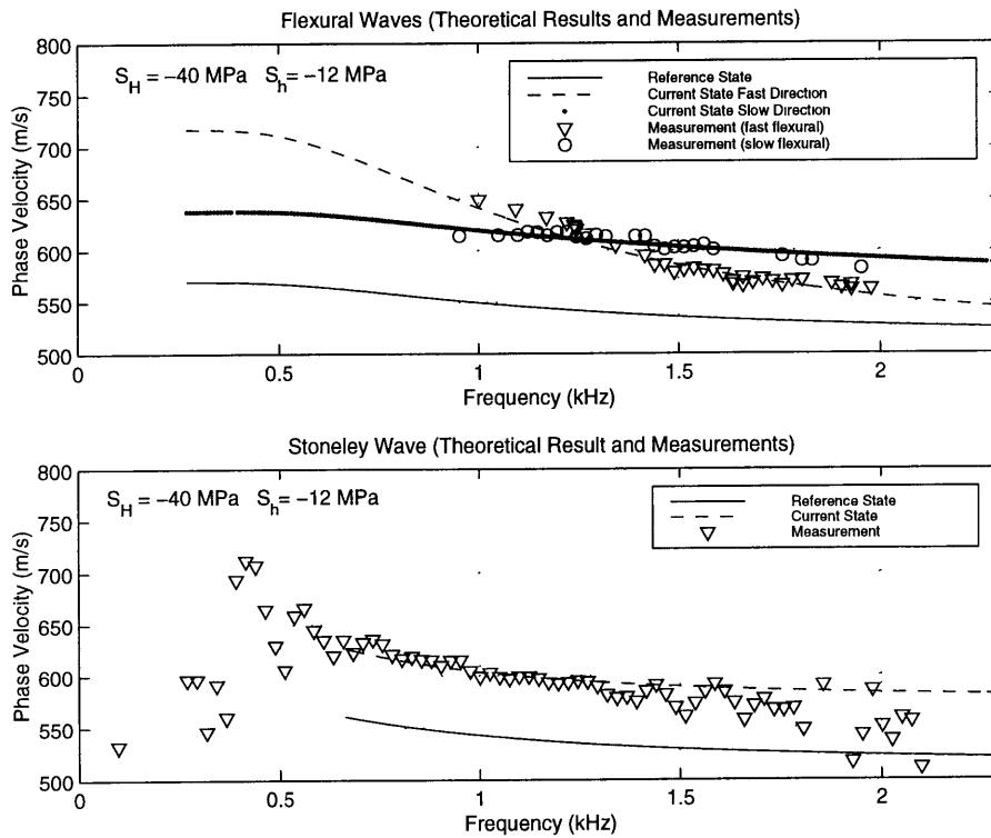
Figure 6-8: Dispersion curves that are estimated from data as well as calculated by the perturbation theory with inverted tectonic stresses and nonlinear elastic constants as inputs. The heavy line in the first figure is the theoretical dispersion curve of the slow flexural wave.
