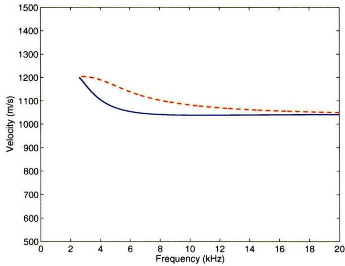
Figure 4-6: Dispersion of quadrupole modes. Solid line: with LWD tool; Dash line: without LWD tool. Formation properties: v_p=3000 m/s, v_s=1200 m/s, \rho=2200 kg/m 3 . Fluid properties: v_p=1500 m/s, \rho=1000 kg/m 3 . Tool properties: v_p=5860 m/s, v_s=3130 m/s and \rho=7800 kg/m 3 .
