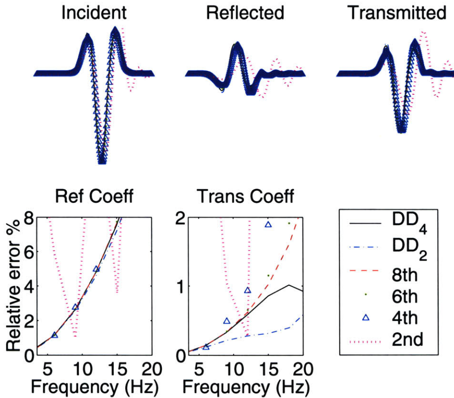
Figure 2-9: The incident, reflected and transmitted waves that propagate in a 2-layer model and are obtained from 6 FDTD computations using uniform grid. The grid size is 1/7 of the smallest wavelength. Both 2nd order and 4th order solutions show noticeable numerical dispersions. The reflection and transmission coefficients are computed from those waves. Their relative errors to the analytical answer are plotted in the frequency domain.
