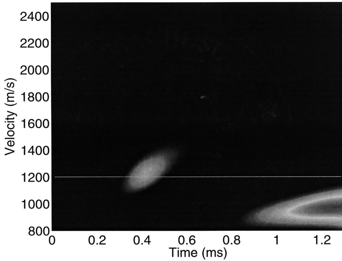
Figure B-5: Semblance result of wayeforms in figure B-2.
