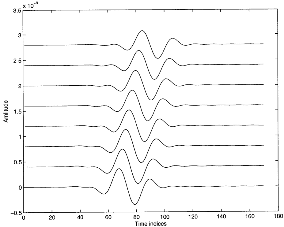
Figure A-1: Synthetic borehole flexural waveforms obtained by a Finite Difference algorithm.
