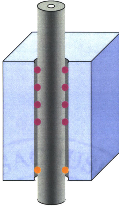
Figure 4-1: A schematic diagram of an LWD tool.
