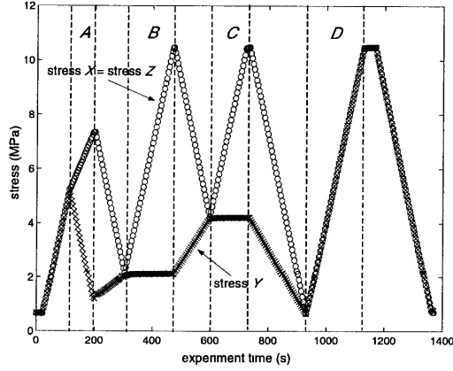
Figure C-2: Loading cycle ABCD of the tri-axial pressure machine. To preserve the intrinsic transverse isotropy of the sample, the stress in the X -direction is equal to the stress in the Z -direction (Dillen, 2000).
