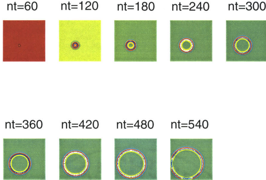
Figure 2-13: The progressive development of the wave shown in figure 2-12. The wavefront keeps its circular shape, suggesting no phase distortion, throughout its propagation across the medium and there is no noticeable numerical reflections observed.
