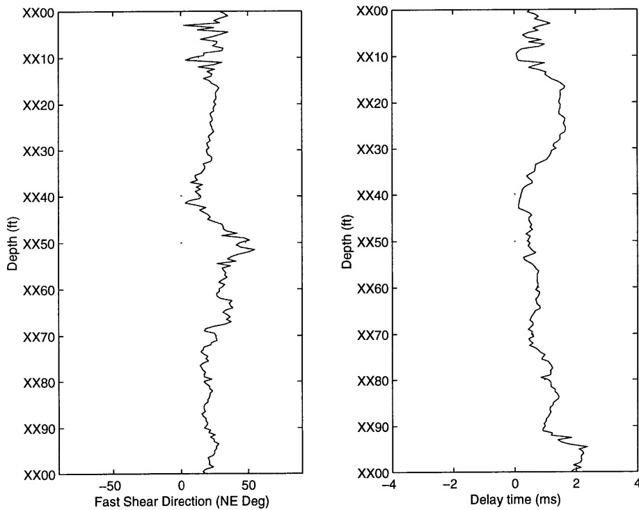
Figure 6-6: Maximum stress direction in the stressed zone where crossovers in flexural dispersions are continuously observed. The maximum horizontal stress is oriented 30^{\circ} \sim 40^{\circ} northeast. The result agrees with the world stress map (figure 6-7). The second panel shows the group delay of the slow flexural wave from the fast one obtained by cross-correlating the low-frequency part of the fast and slow flexural waveforms.
