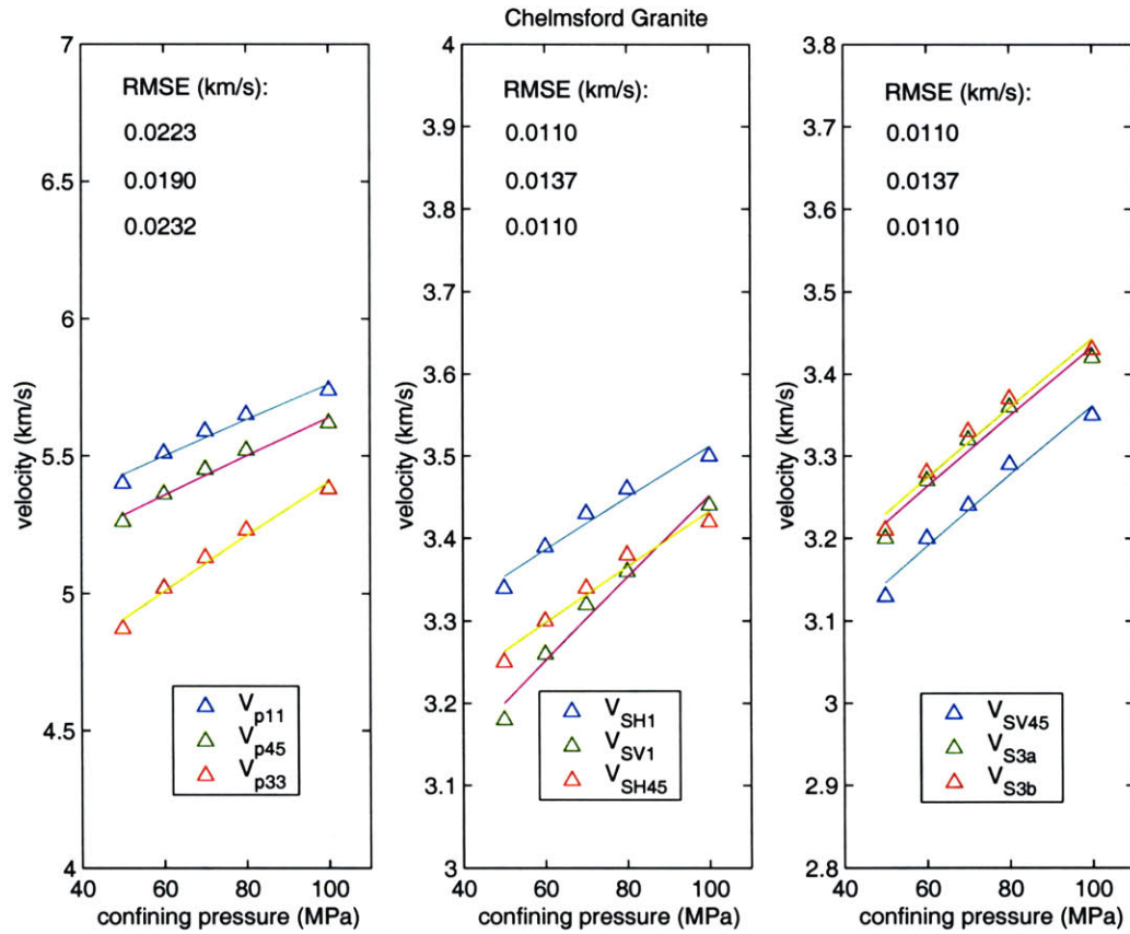
Figure C-11: Theoretical and experimental results and their relative errors for Chelmsford granite (experiment by Lo et al (1986). \Delta : experiment; solid line: theory.
