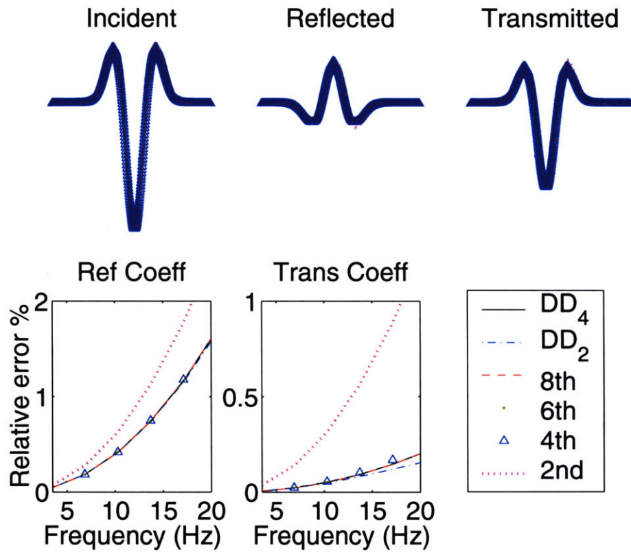
Figure 2-11: Same as figure 2-9 except that the grid size is about 3 times smaller while errors in reflection and transmission coefficients drop more than 5 times. With little numerical dispersion, the 2nd order scheme does not produce the most accurate reflections and transmissions as some studies suggested.
