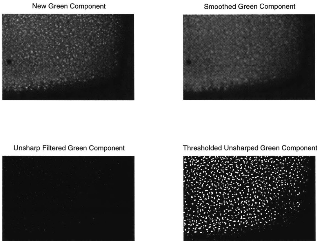
Figure B-6: The fluorescein component is shown, along with the results of the low-pass filter, the unsharp mask, and then the thresholding.
