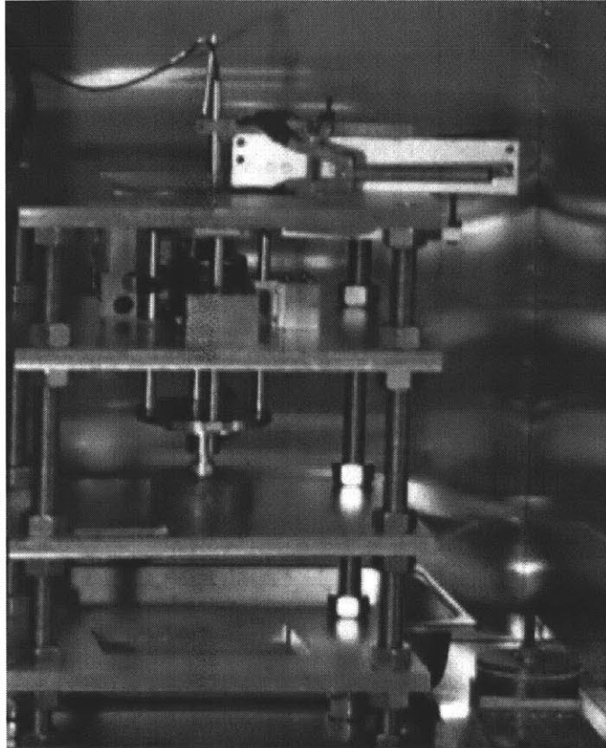
Figure A-2: The incustat machine inside a standard cell culture incubator. The chamber in the machine is being compressed. The chamber to the right of the incustat is being used as a static control.
