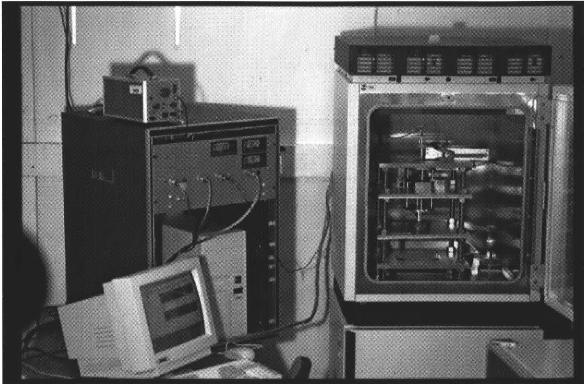
Figure A-6: The incustat within its incubator along with the controlling computer and electronic hardware. This is an old picture taken when an actual signal generator was used to drive the hardware feedback circuitry in dynamic compression experiments.
