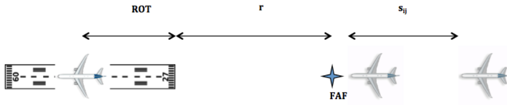
Figure 2-6. Representation of an opening case used for the runway capacity model
