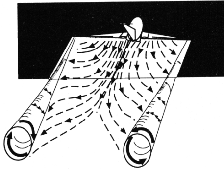
Figure 2-1. Illustration of a wake vortex generator aircraft in flight [1]
