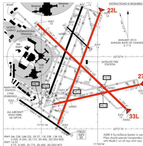
Figure 3-3. ROT data measured on runway 22L, 27, and 33L at Boston
