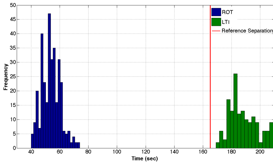
Figure 4-12. Runway occupancy and landing time interval for Boeing 757 - small arrival pairs
