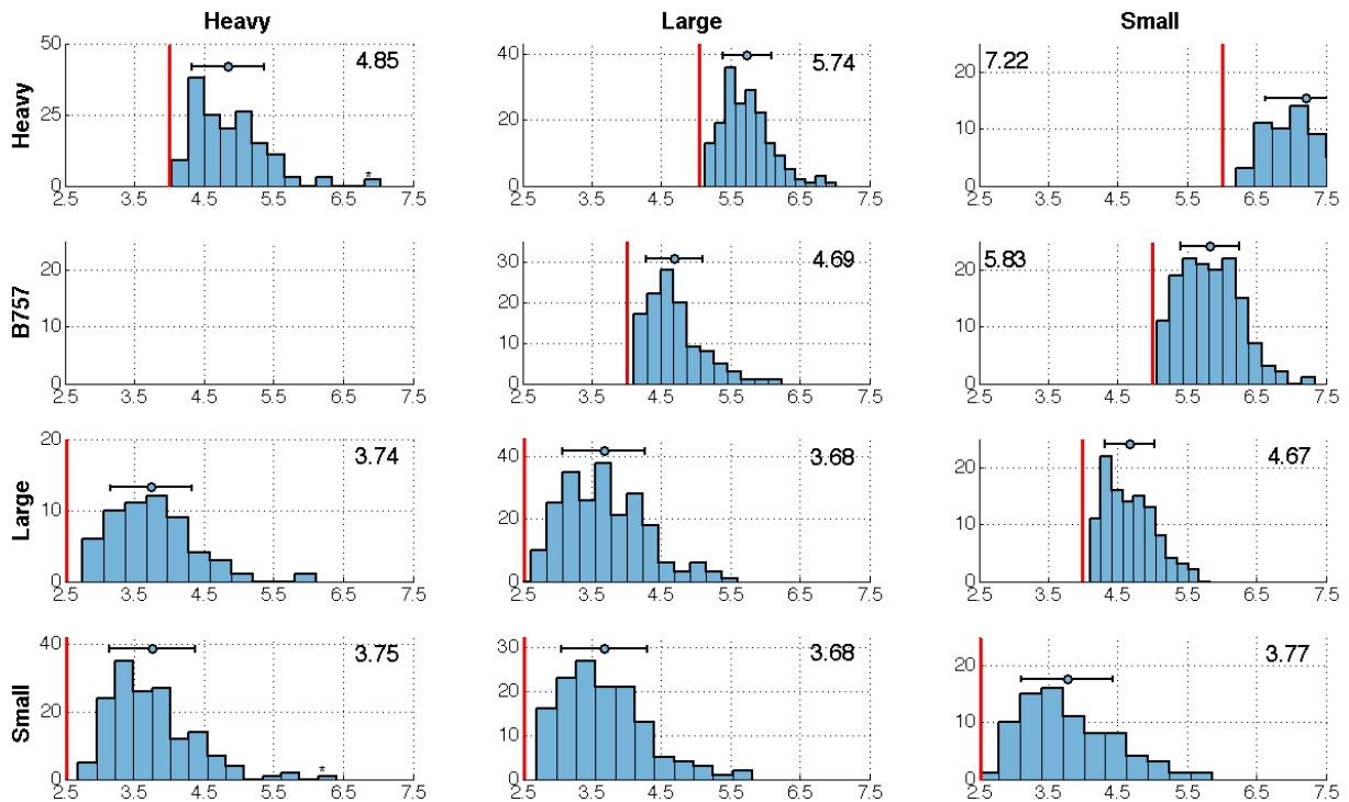
Figure 4-5. Inter-arrival distance measurements at Boston (no B757-heavy pairs)
