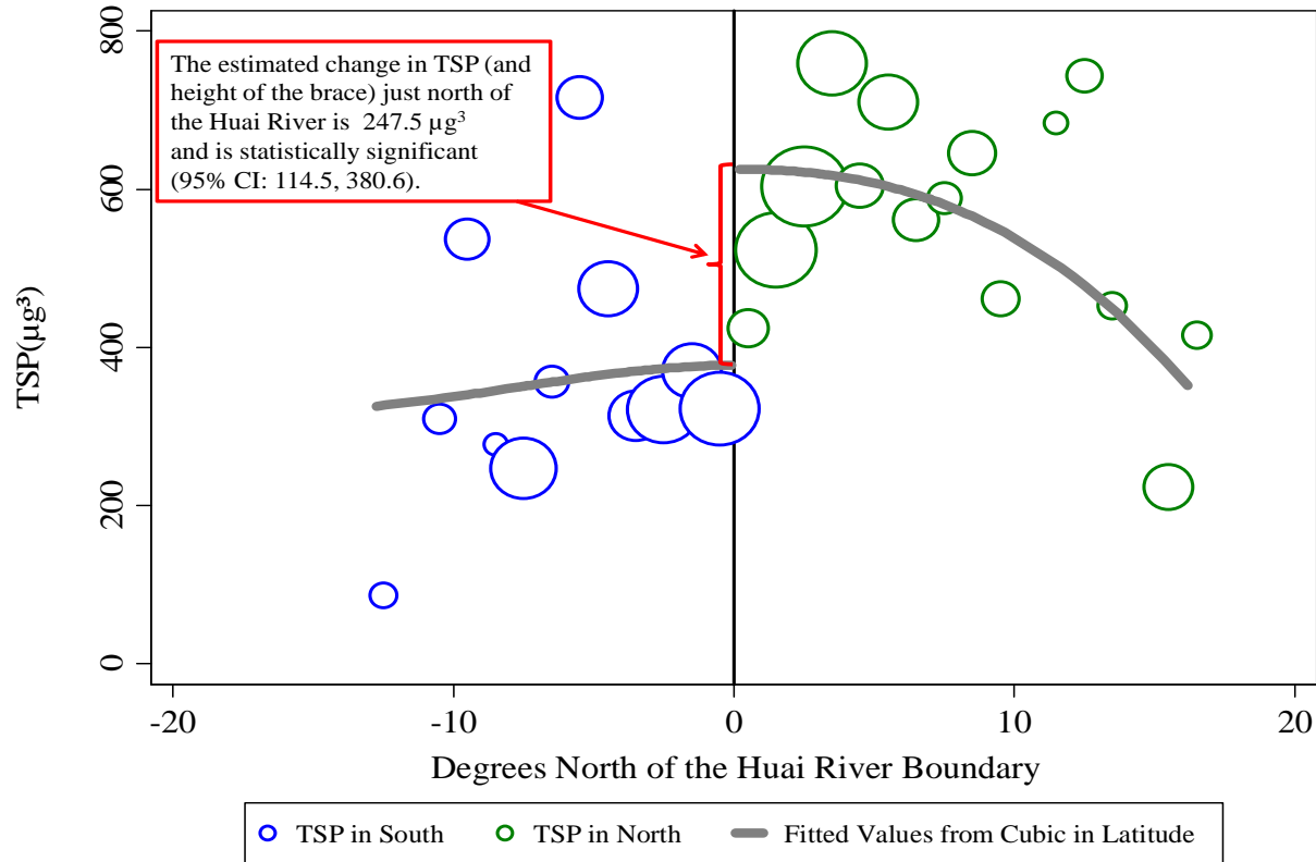
Total Suspended Particulate Concentration Rises at the Huai River Boundary
