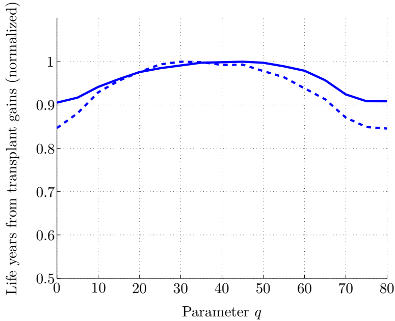
Figure 4: Predicted (solid) and simulated (dashed) life years from transplant gains for different values of the parameter q for the case study in Section B.
