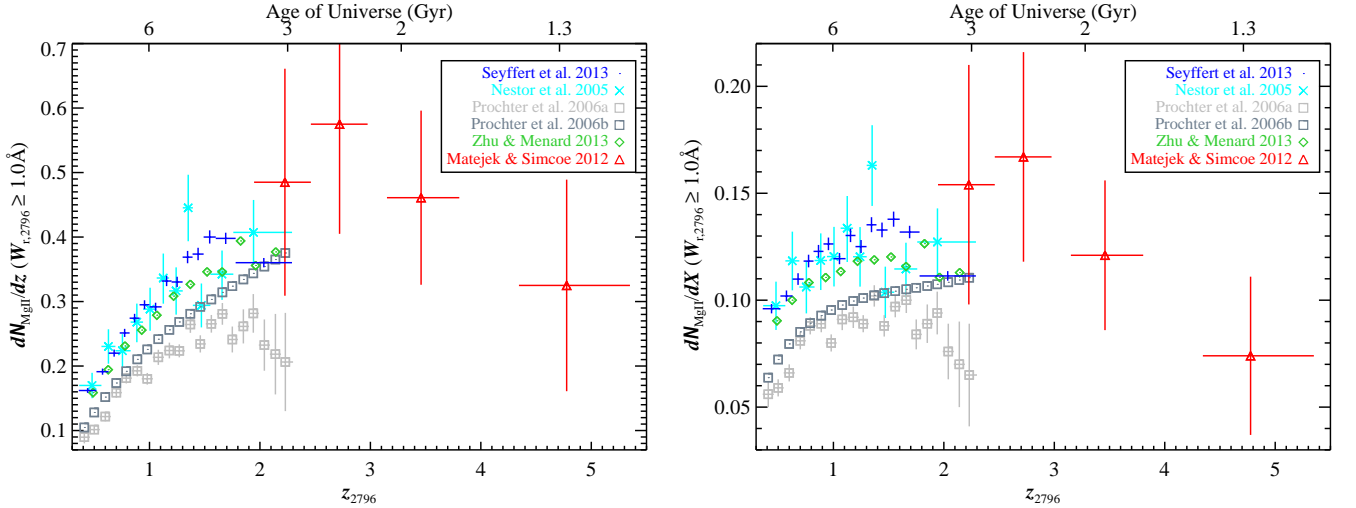
Figure 7. Redshift (left) and co-moving path length (right) Mg II line densities. We compare apples-to-apples dN_{\text{Mg II}}/dz with W_r \geq 1 \text{ \AA} from six surveys: this work (blue pluses); N05 (cyan crosses); P06 (light gray squares); Prochter et al. (2006b, dark gray squares); ZM13 (green diamonds); and Matejek & Simcoe (2012, red triangles). The redshift density steadily increases from z \approx 0.4 to \approx 1.75 . The relatively flat dN_{\text{Mg II}}/dX indicates modest evolution in the product of the co-moving number density and the physical cross-section of the absorbing clouds.
