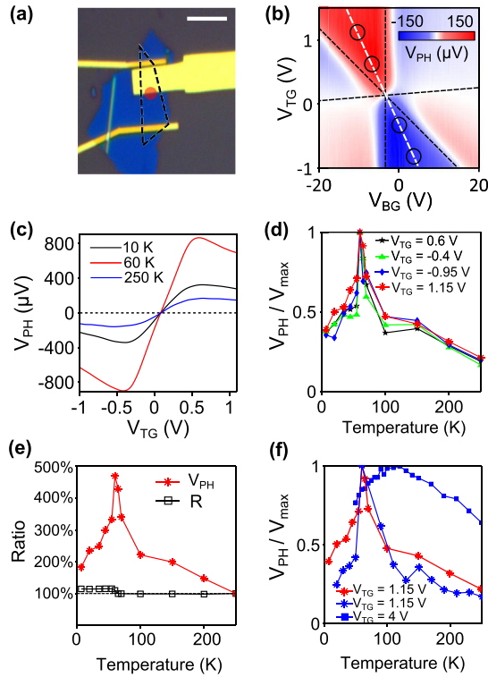
FIG. 1 (color online). (a) Optical microscope image of the device incorporating boron nitride top-gate dielectric. The dashed black line marks the boundary of graphene underneath the boron nitride. (b) Photovoltage V_{PH} versus V_{BG} and V_{TG} at T = 250 K with laser fixed at the p - n interface [red dot in (a)]. Optical power P = 100 \mu\text{W} . The white dashed line indicates \mu_1 = -\mu_2 . (c) Traces of (b) for \mu_1 = -\mu_2 at different temperatures T = 10 K, T = 60 K, T = 250 K. Along \mu_1 = -\mu_2 , the cooling profile is symmetric from the p - n interface. (d) V_{PH} as a function of temperature (normalized to the maximum value) at particular points [black circles in (b)] along the \mu_1 = -\mu_2 line. (e) Comparison between the temperature dependence of the photovoltage V_{PH} and the resistance R . Both V_{PH} and R are normalized by their values at T = 250 K. (f) The temperature dependence of V_{PH} at low ( |\mu_1| = |\mu_2| \approx 100 MeV) and high ( |\mu_1| = |\mu_2| \approx 200 MeV) densities, showing a shift of T^* . Red curve, device 1; blue curve, device 2.
