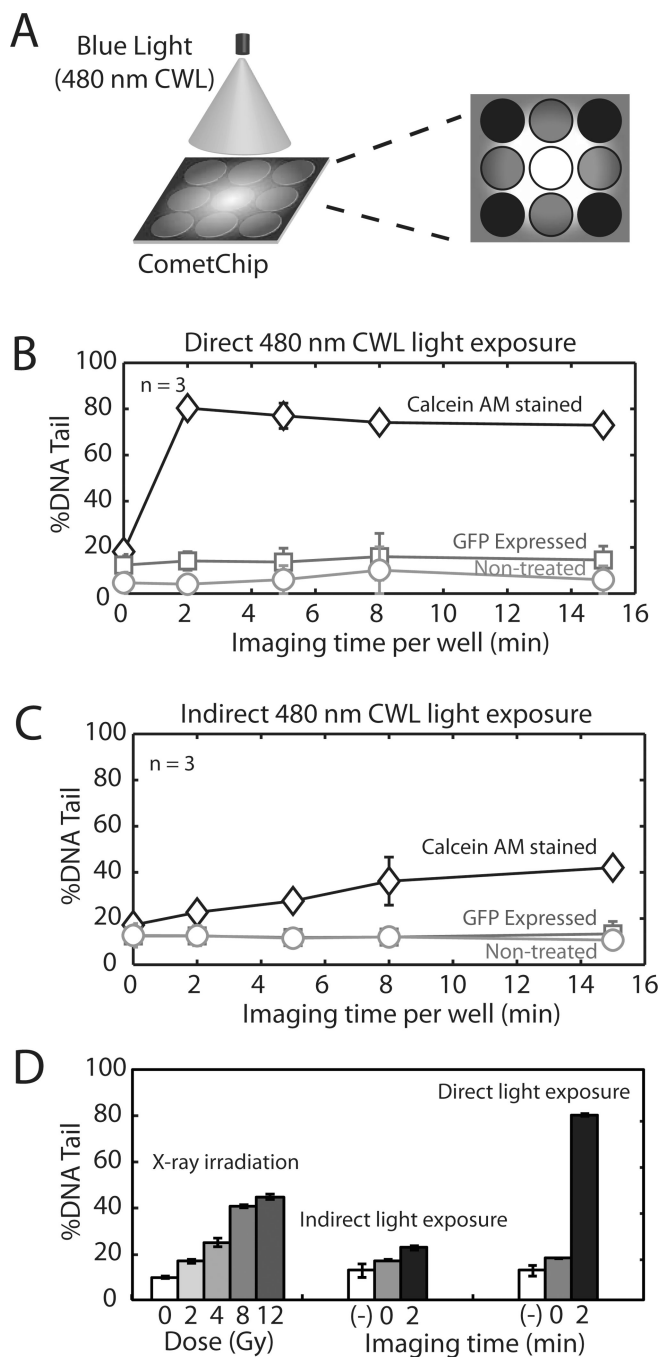
Figure 3. Direct and Indirect light-induced damage in fluorescent cells. (A) Diagram indicating indirect light exposure in neighboring wells when imaging the center well. (B–C) DNA damage levels in U2OS cells exposed to direct and indirect blue light (480 nm CWL) from microscope. Data for control cells, cells expressing GFP, and Calcein AM-stained U2OS cells are shown. (D) Comparison of damage levels from X-ray irradiation and fluorescent imaging using Calcein AM. (–) represent wild type U2OS cells un-stained with Calcein AM. Data and error bars represent averages and standard errors of three independent experiments.
