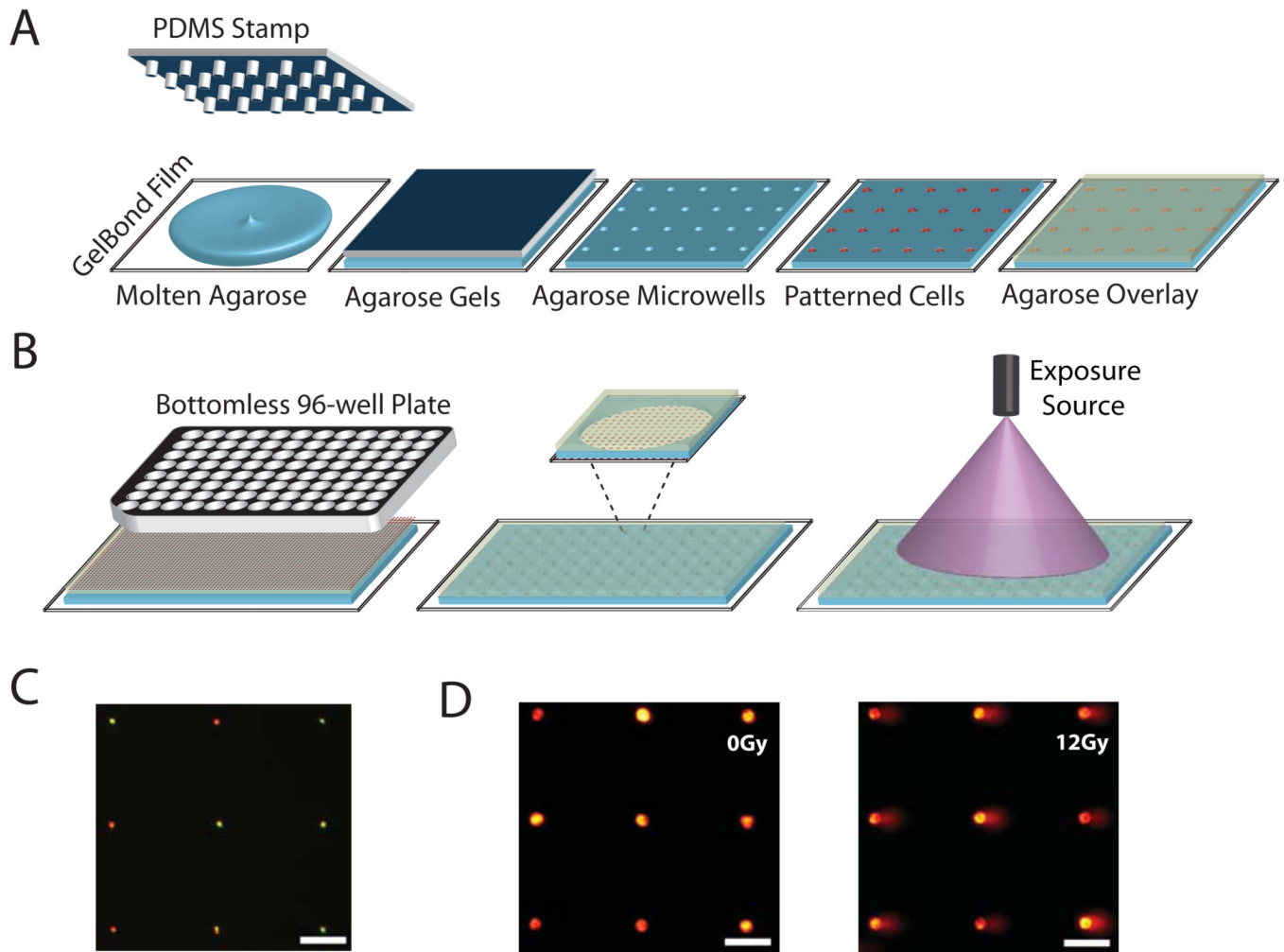
Figure 1. High throughput comet analysis platform. (A) A microfabricated PDMS stamp with microposts is placed onto molten agarose. After the agarose gels, the stamp is removed and cells are loaded into the microwells by gravity. An agarose overlay encloses cells. (B) To create the CometChip, a bottomless 96-well plate is pressed on agarose gel with embedded cell array that is placed on a glass substrate to create the macrowell platform (each well of the 96 well plate is considered to be a single macrowell). Each macrowell has within it ~300 microwells loaded with cells. (C) Single cell loading in microwells. Two populations of cells stained red and green were loaded concurrently. (D) Arrayed non-irradiated (left) and 12-Gy irradiated (right) microwell comets observed under 10x objective lens. Monochrome images were collected from microscope camera and colored with Red Hot lookup Table using Image J. Horizontal scale bars are 100 \mu\text{m} .
