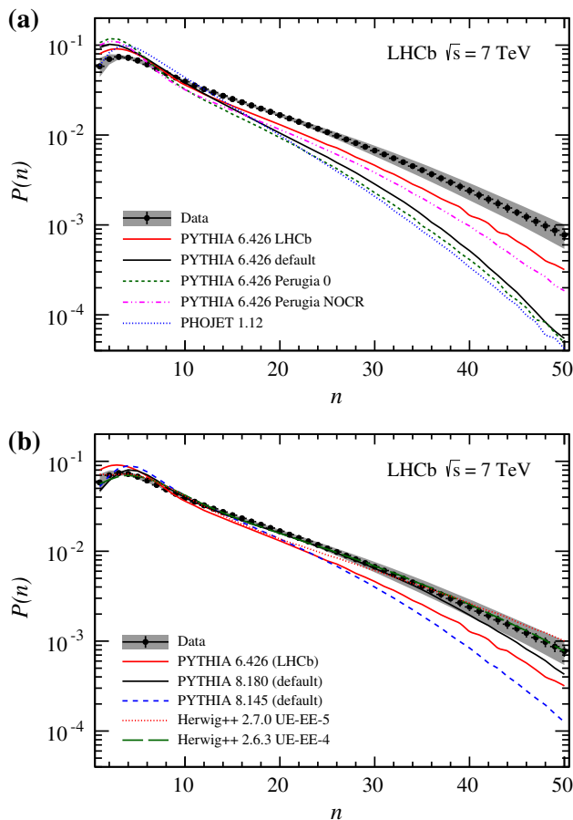
Fig. 3 Observed charged particle multiplicity distribution in the full kinematic range of the analysis. The error band shows the combined statistical and systematic uncertainties. The data are compared to several Monte Carlo predictions, a PYTHIA 6 and PHOJET, b PYTHIA 8 and HERWIG++. Both plots show predictions of the LHCb tune of PYTHIA 6, which is used in the analysis
