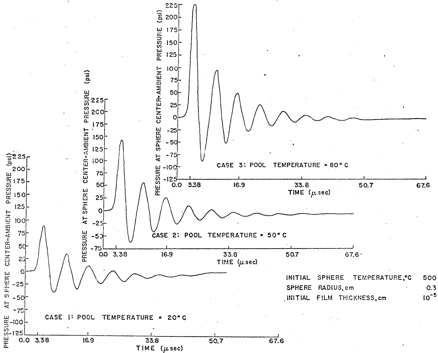
FIGURE 6 THE CALCULATED EFFECT OF POOL TEMPERATURE ON THE PRESSURE AT THE SPHERE CENTER
