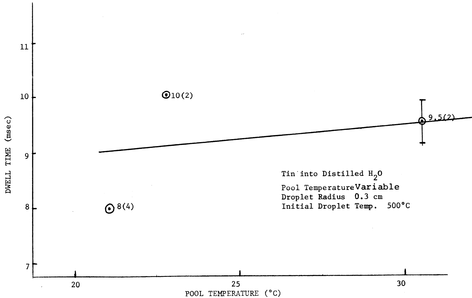
FIGURE 17 DWELL TIME VS. POOL TEMPERATURE
