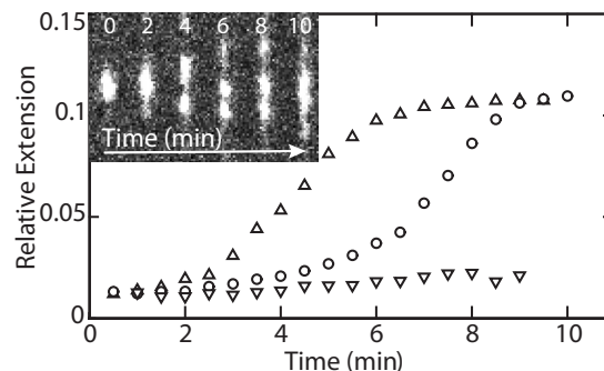
Fig. 5 Unpacking of T4–DNA following exposure to a solution of 1 ( \Delta ), 3 ( \circ ) and 5 ( \nabla ) \mu\text{M} protamine in 1\times\text{T} buffer and 100 mM NaCl. Prior to unpacking, the DNA molecules were brought into the array of 200 \times 250 \text{ nm}^2 channels in compacted form. The data represent averages pertaining to the unpacking of five different DNA molecules. The inset shows a time-lapse series of fluorescence images pertaining to unpacking following exposure to 1 \mu\text{M} protamine in 1\times\text{T} buffer and 100 mM NaCl.
