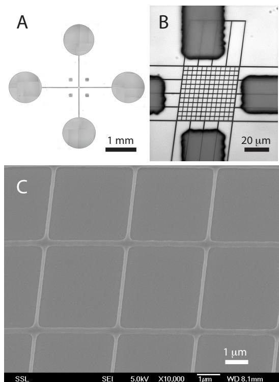
Fig. 1 (A) Bright field optical image of the bonded lab-on-chip device. The loading reservoirs are connected to the central grid of nanochannels by microchannels in SU-8 resin. (B) Optical image of the master stamp featuring the nanochannel grid with connecting microchannels. (C) Scanning electron micrographs of the central HSQ master showing a positive standing crossed-channel structure with widths of 250 and 150 nm and a uniform height of 200 nm. The wide and narrow channels are laid on a rectangular grid and separated by 4.0 and 3.75 \mu\text{m} , respectively.
