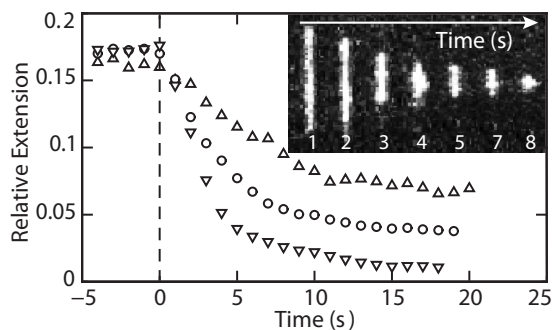
Fig. 4 Compaction of T4–DNA following exposure to a solution of 1 ( \Delta ), 3 ( \circ ) and 5 ( \nabla ) \mu\text{M} protamine in 1\times\text{T} buffer. The DNA molecules are confined in channels with a cross-section of 200 \times 250 \text{ nm}^2 . The data represent average trajectories pertaining to the compaction of five different molecules. The inset shows a time-lapse series of fluorescence images pertaining to the compaction following exposure to 5 \mu\text{M} protamine in 1\times\text{T} buffer. Time zero is defined as the moment when the molecules start to compact.
